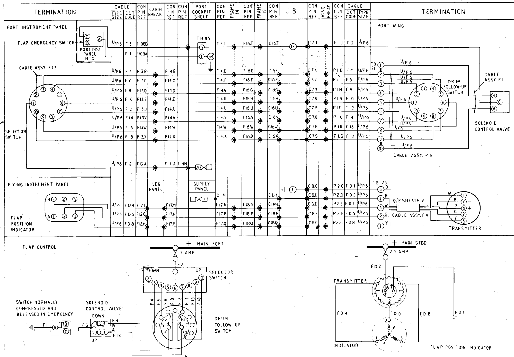
Fig.1. Flap control and position indicator
