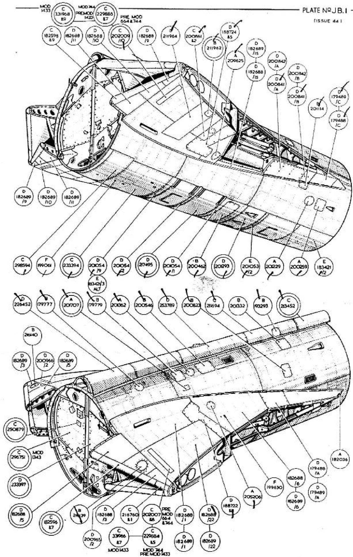
CENTRE FUSELAGE
