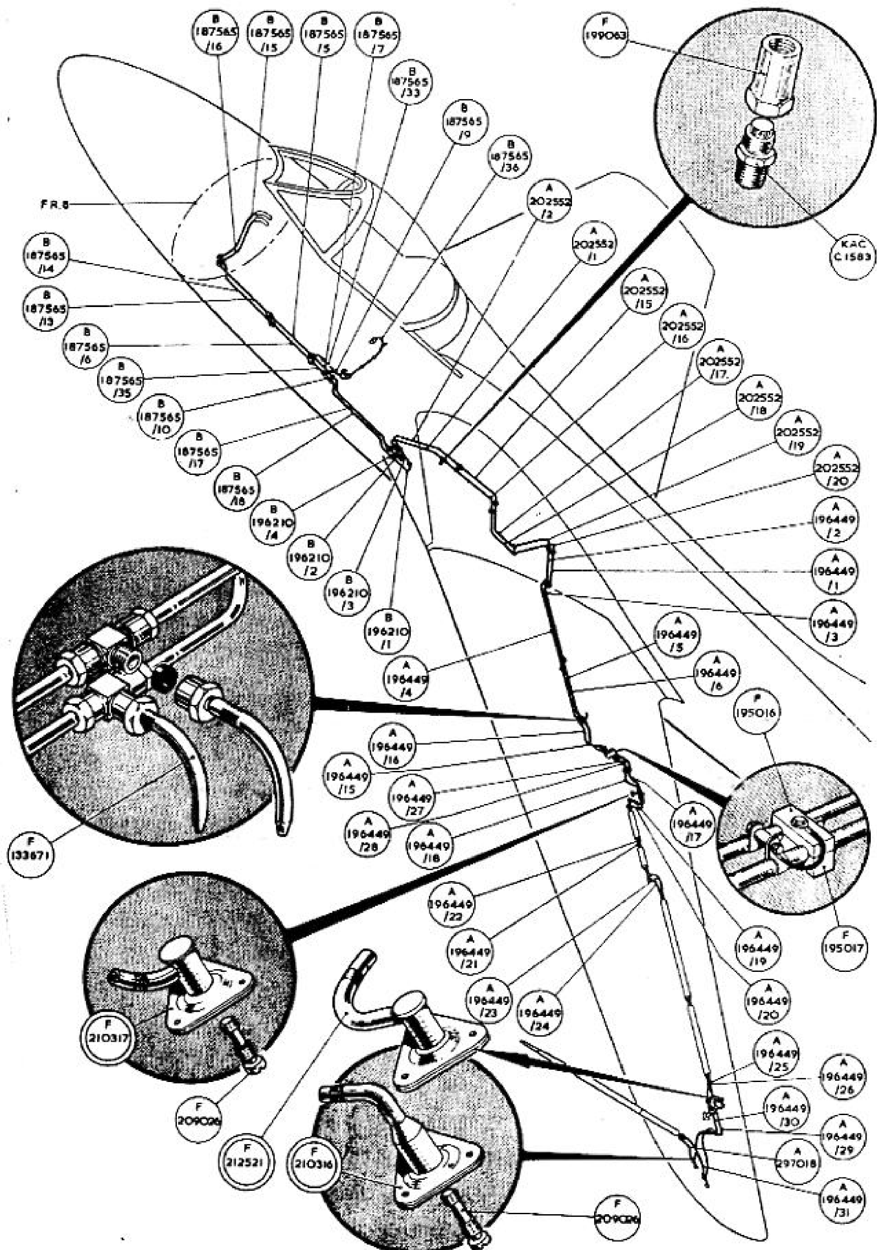
PITOT INSTALLATION
