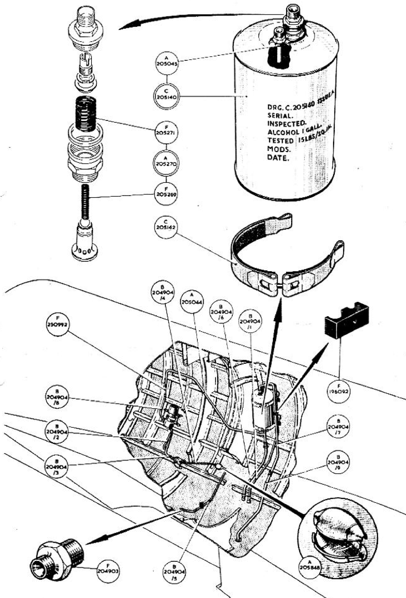
FUEL FILTER DE-ICING SYSTEM
