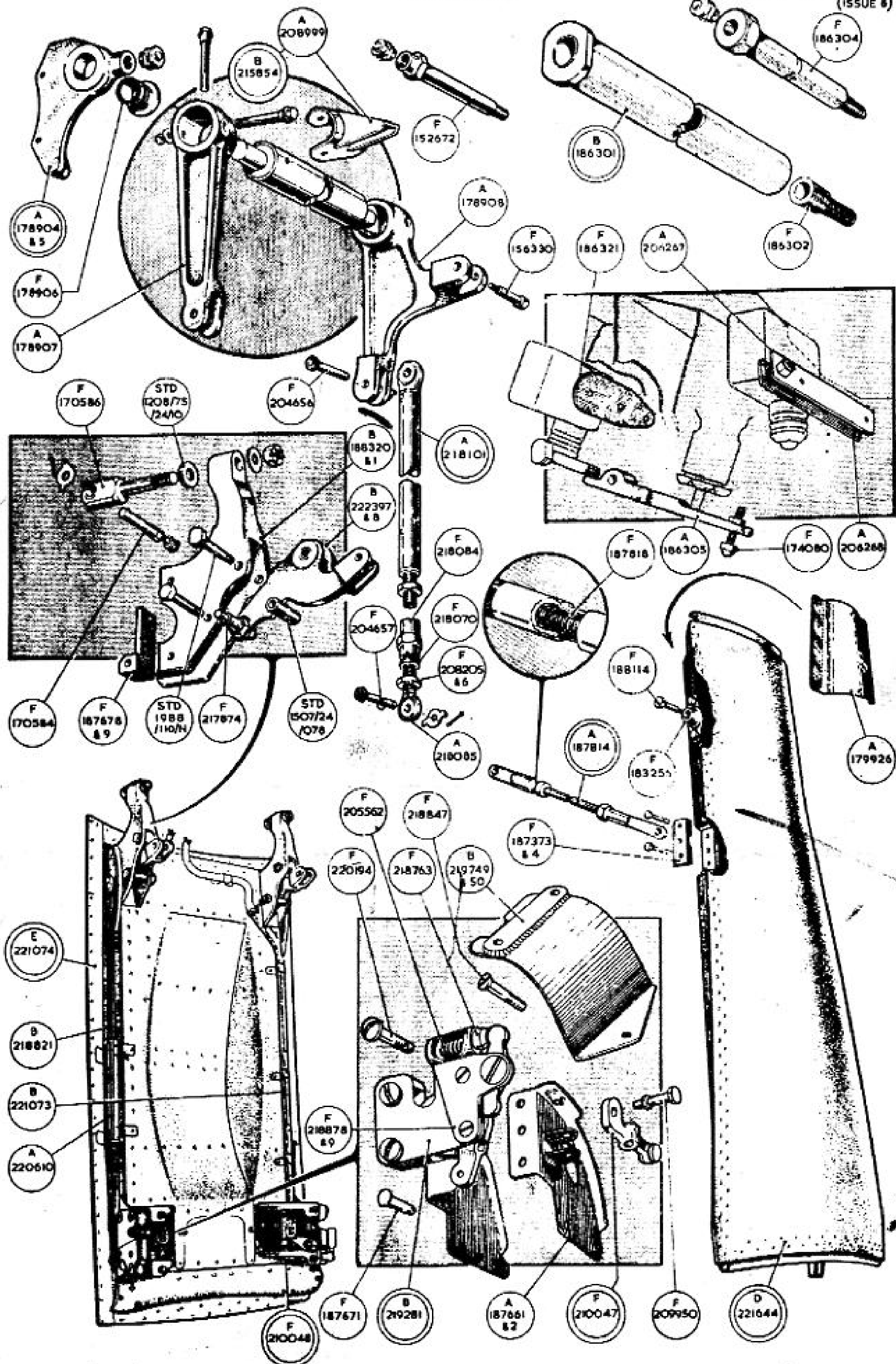
NOSE UNDERCARRIAGE
