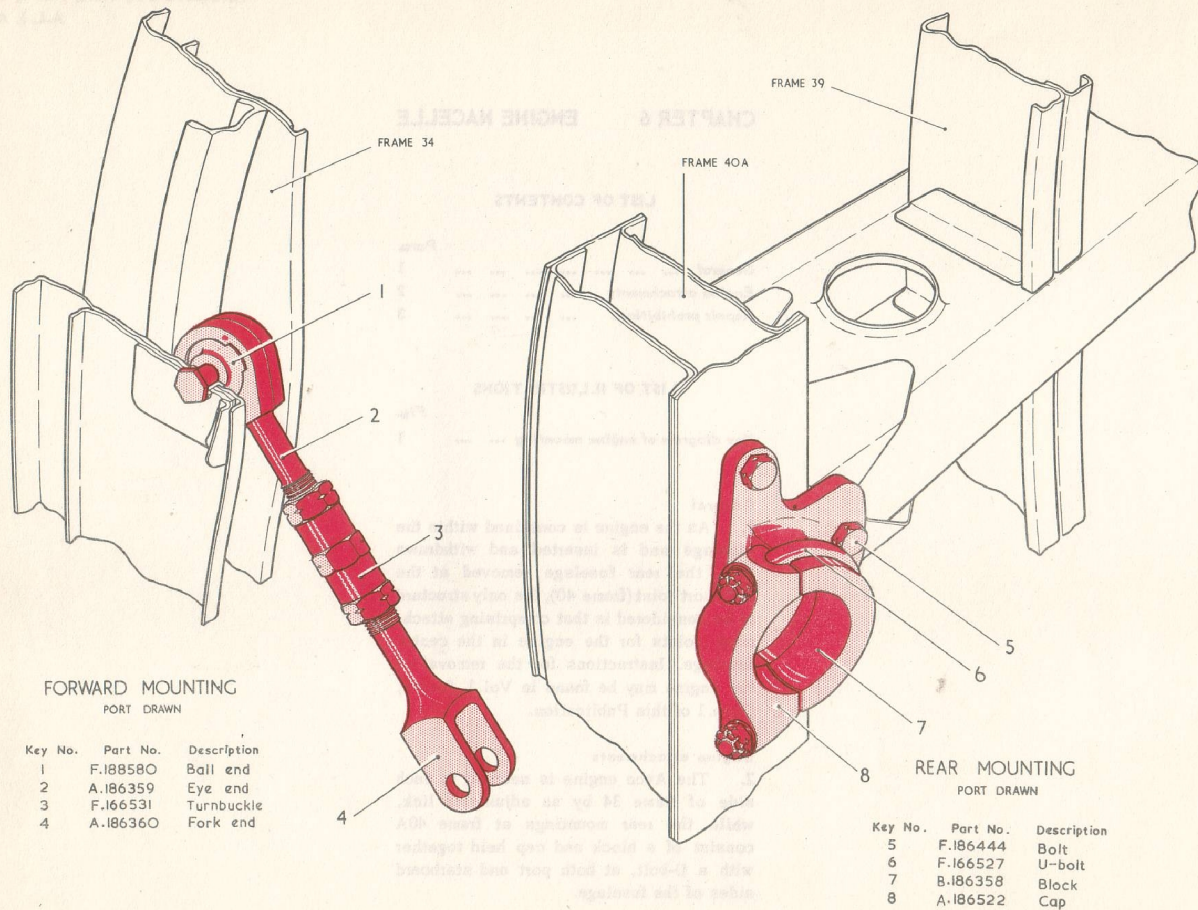
FIG.1. KEY DIAGRAM OF ENGINE MOUNTING
