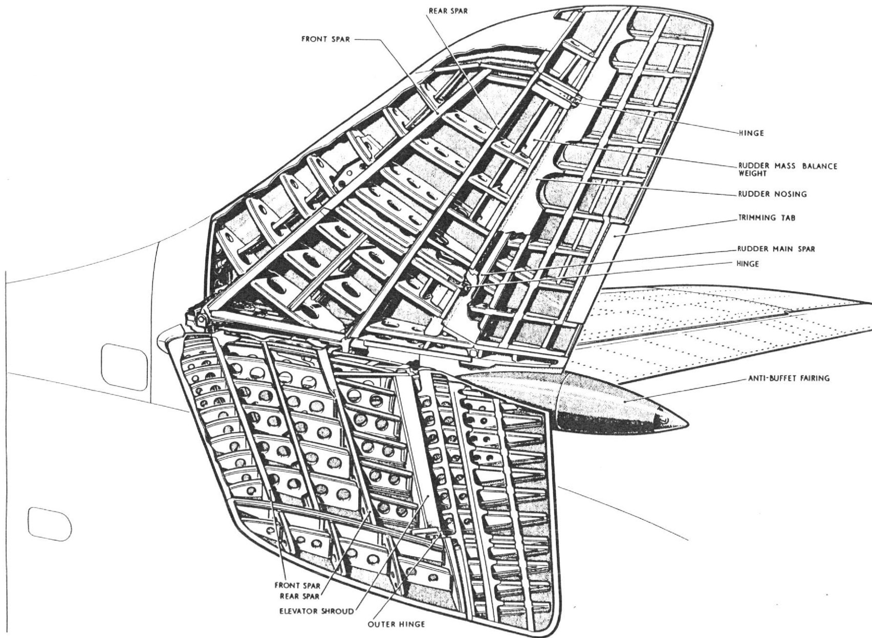
Fig. 1 Tail unit
