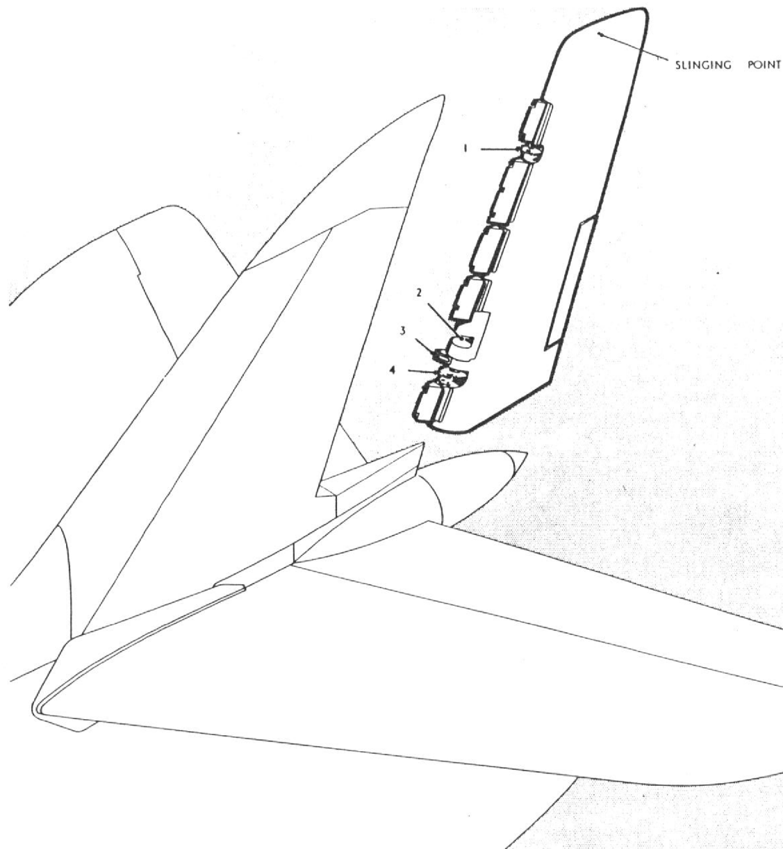
Fig. 2 Removal of rudder
