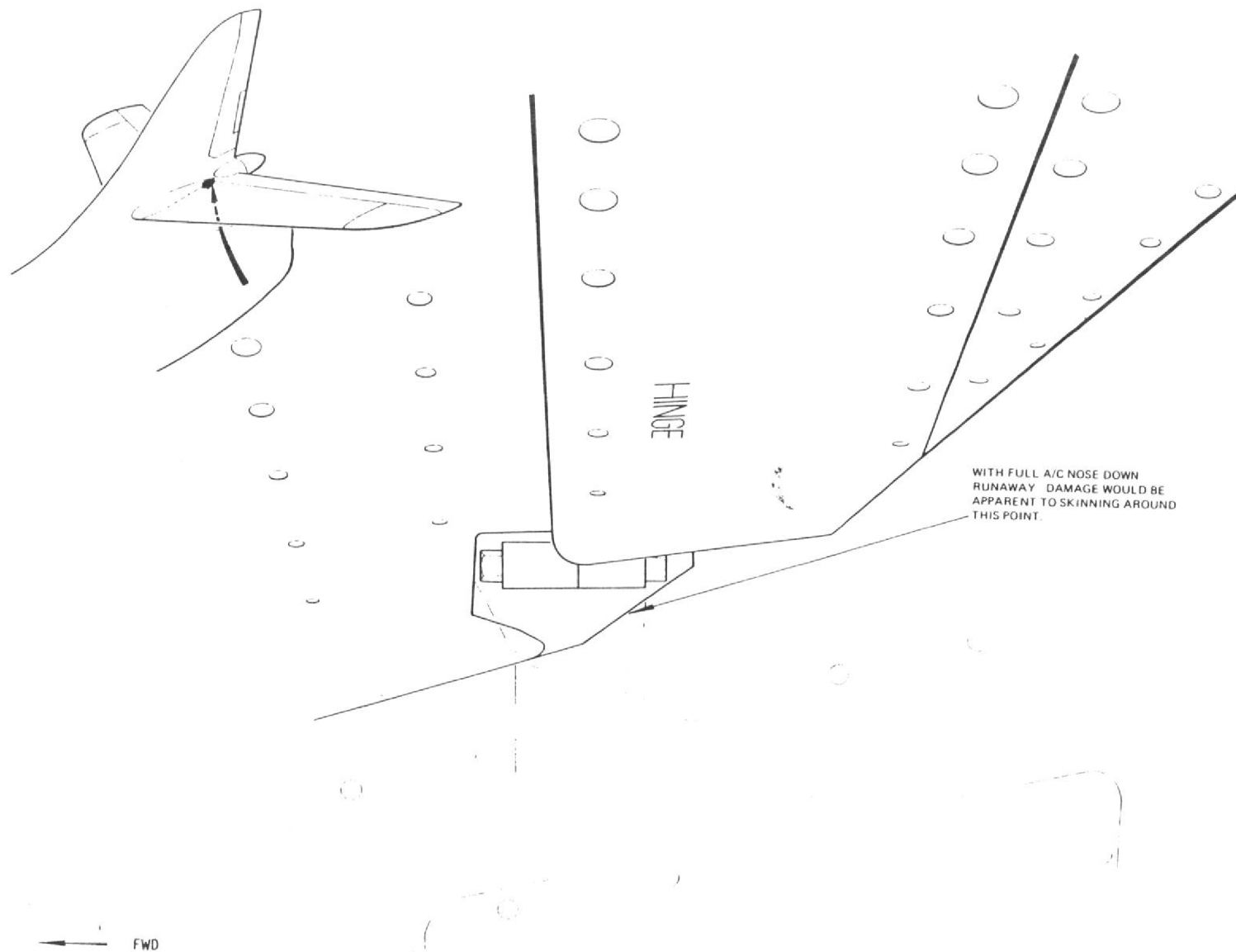
VIEW ON UNDERSIDE INBOARD PORT ELEVATOR
