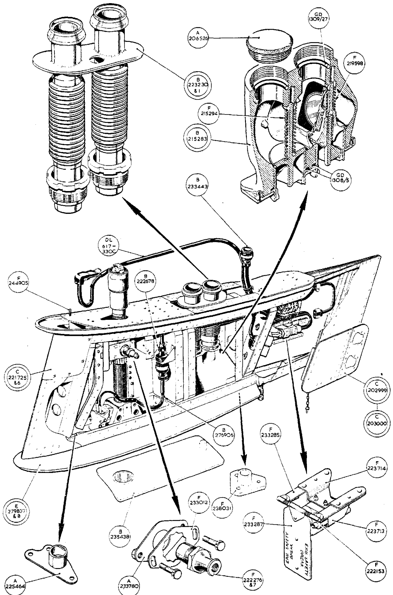
PYLONS - INBOARD
