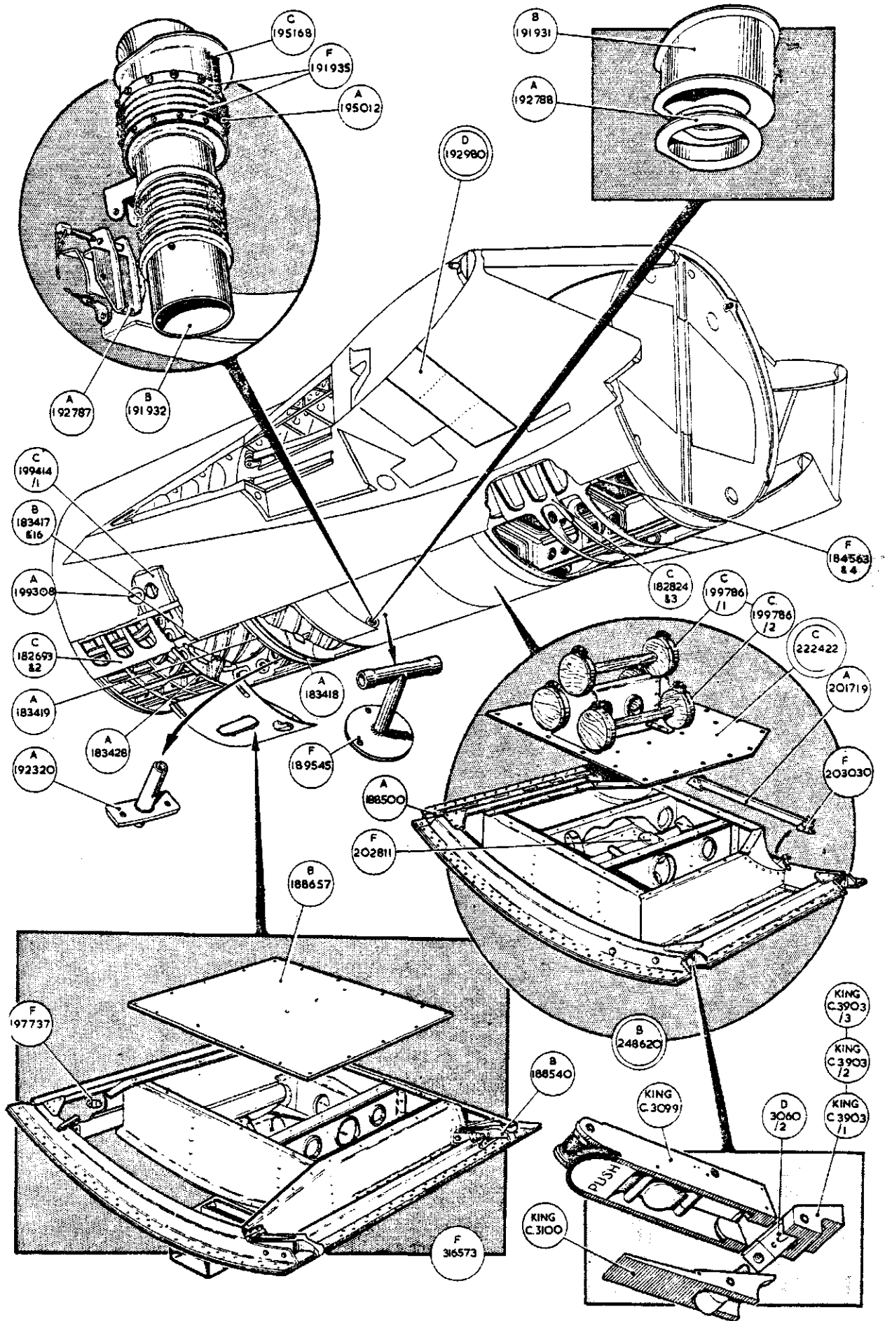
CENTRE FUSELAGE
