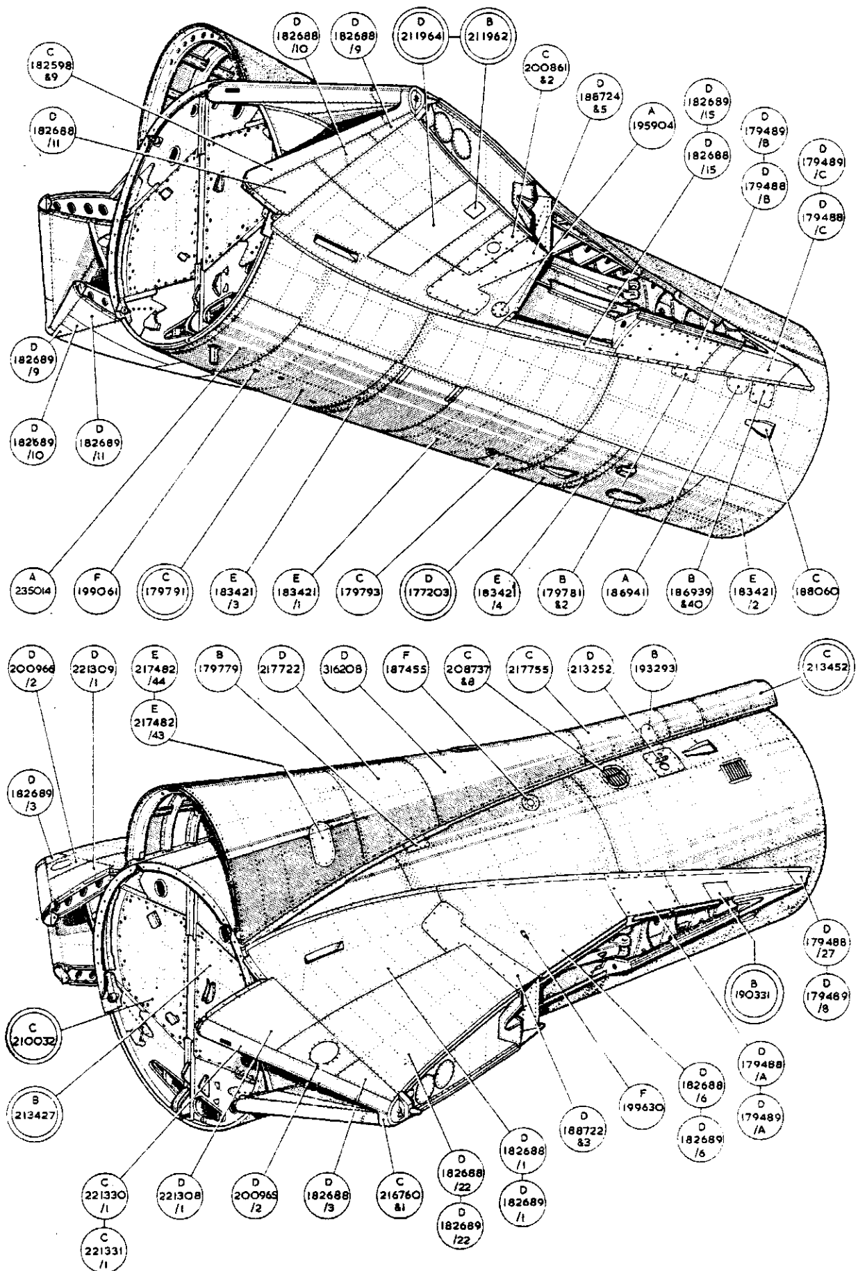
CENTRE FUSELAGE
