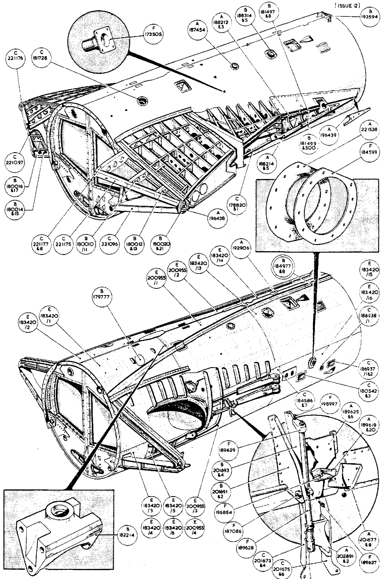
CENTRE FUSELAGE
