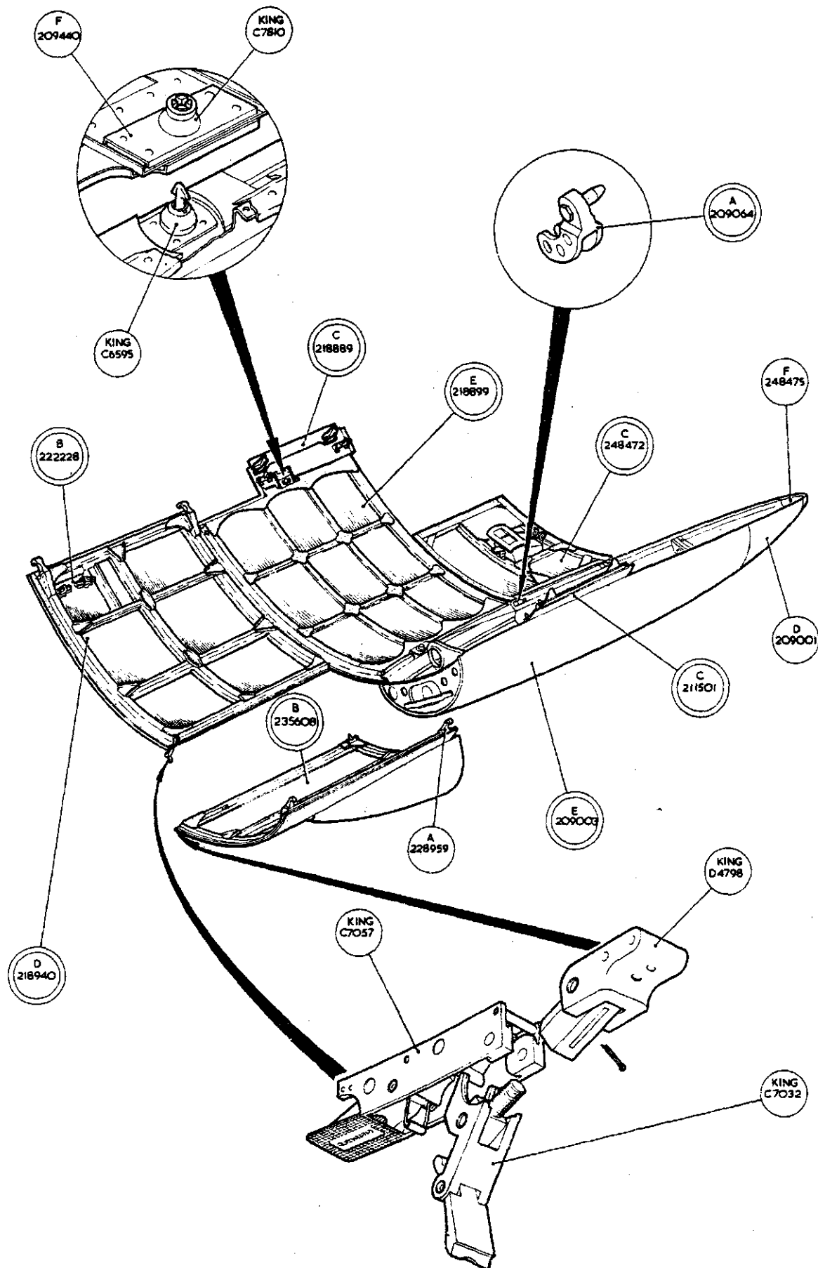
FRONT FUSELAGE
