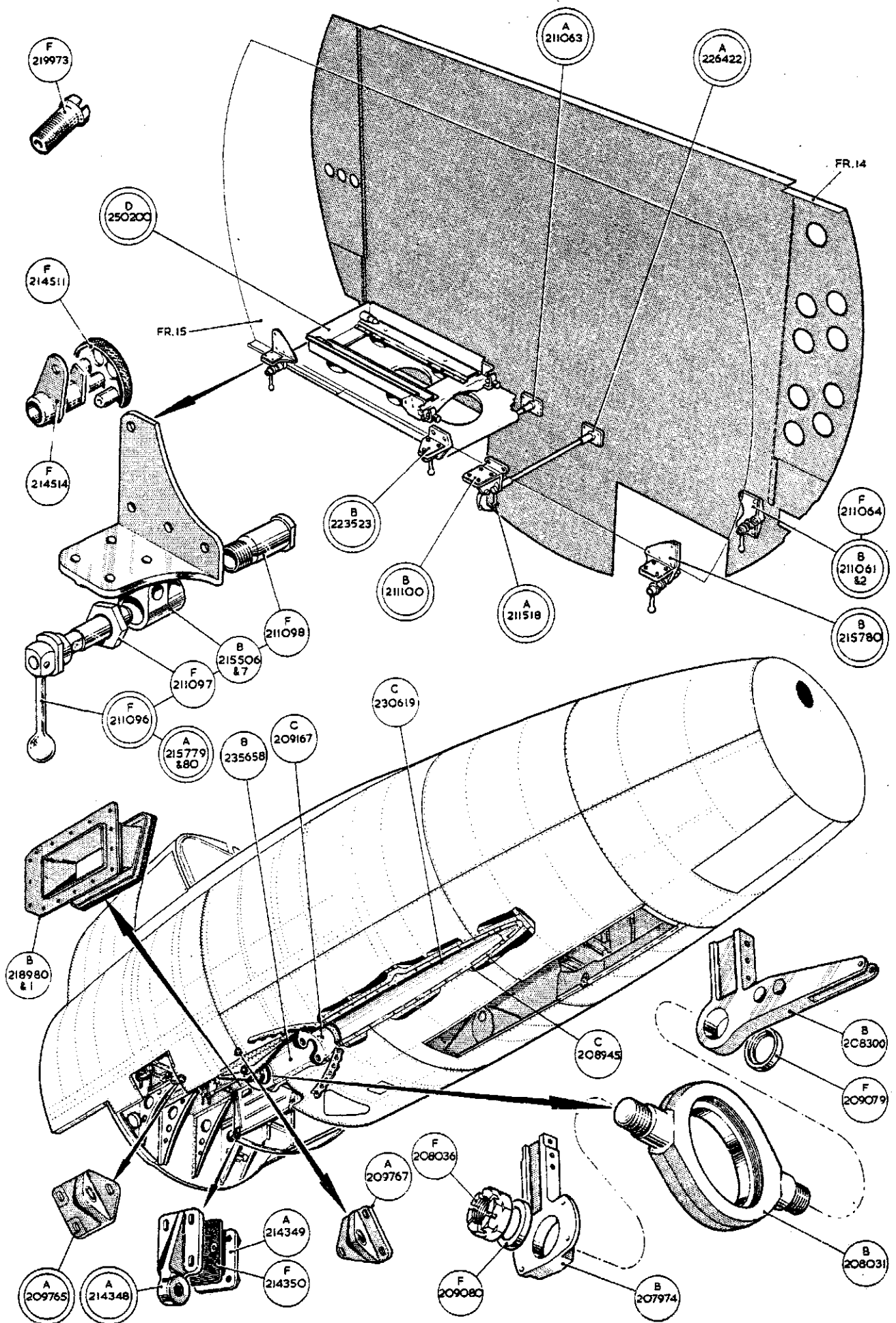
FRONT FUSELAGE
