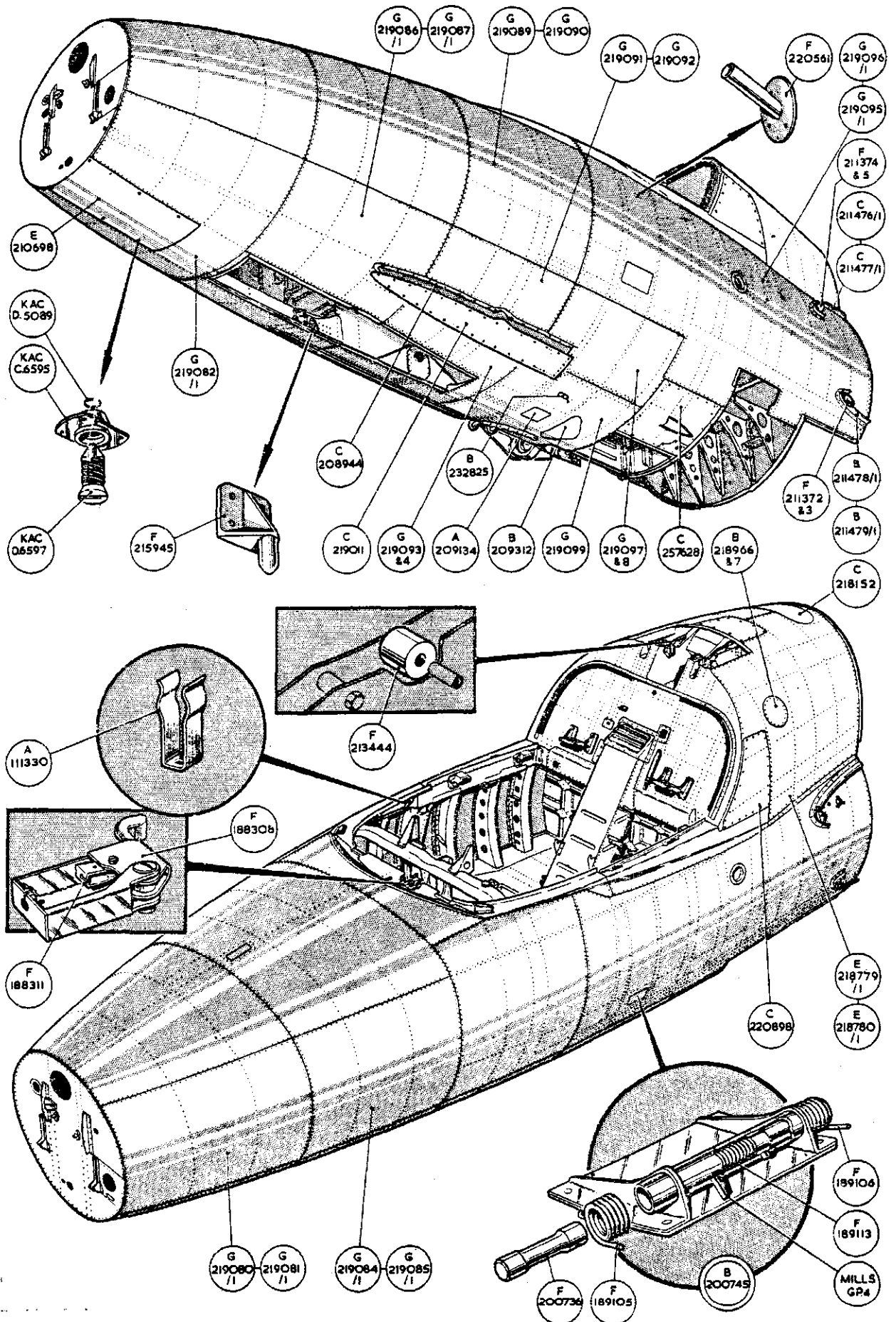
FRONT FUSELAGE
