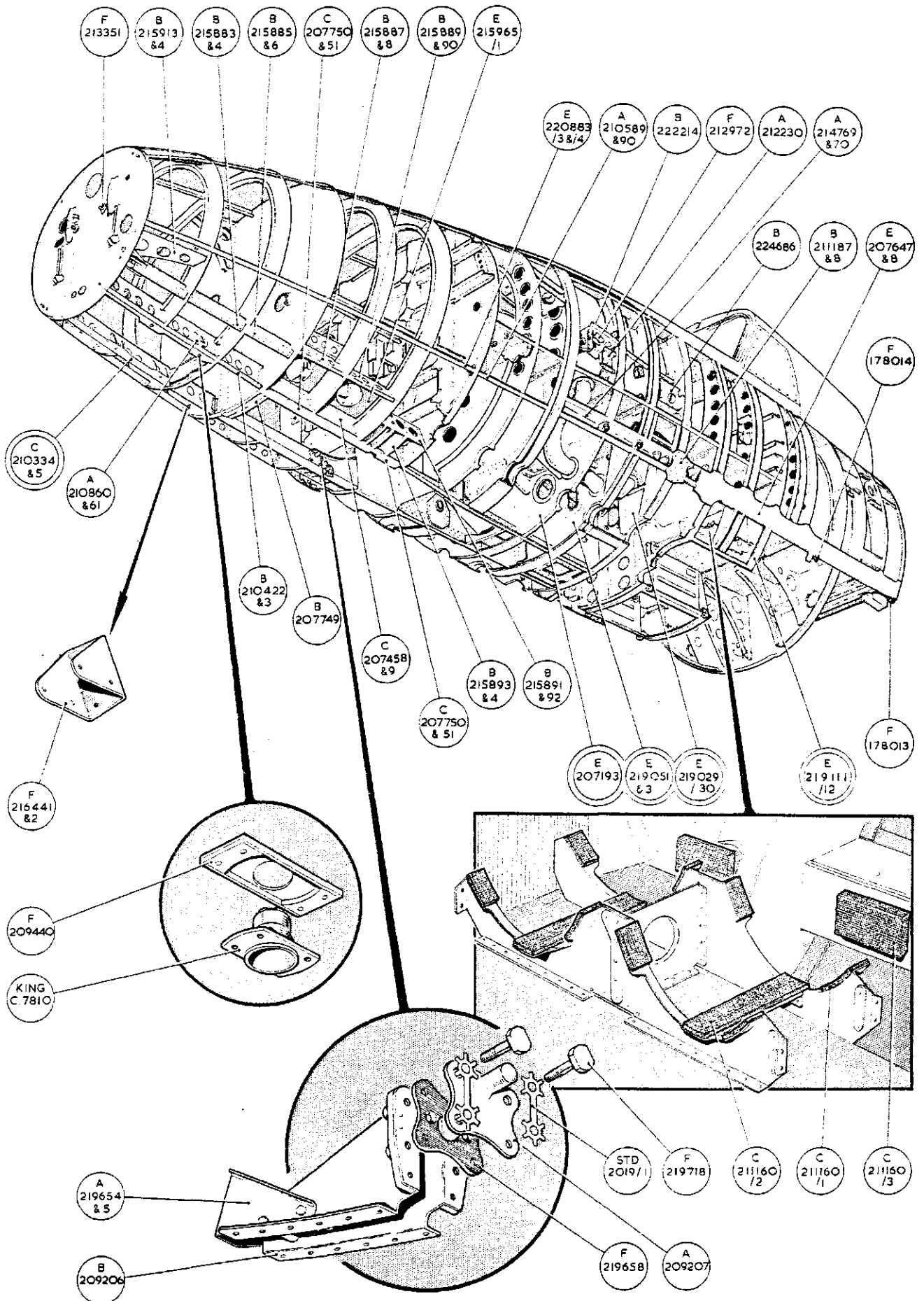
FRONT FUSELAGE
