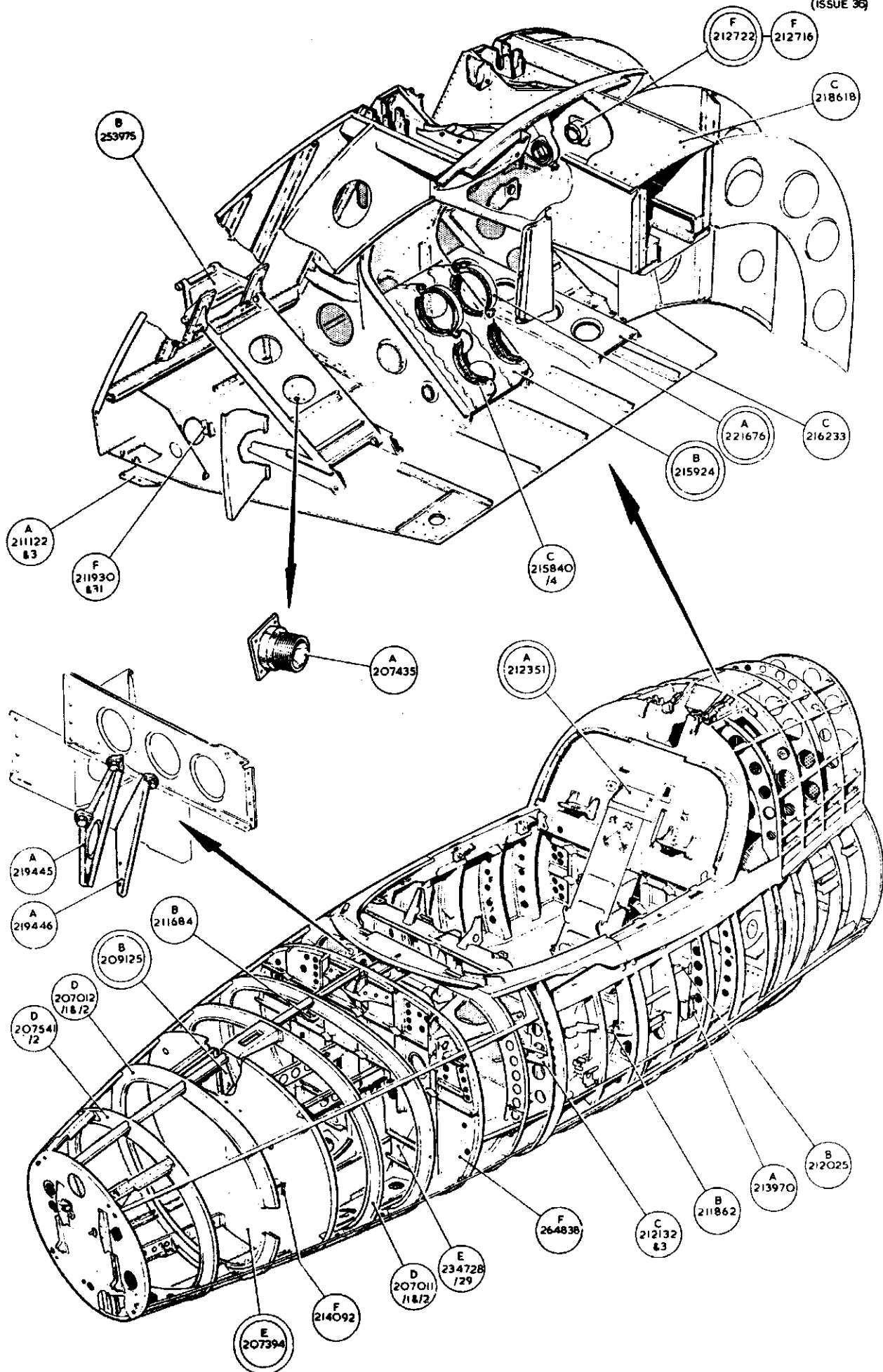
FRONT FUSELAGE
