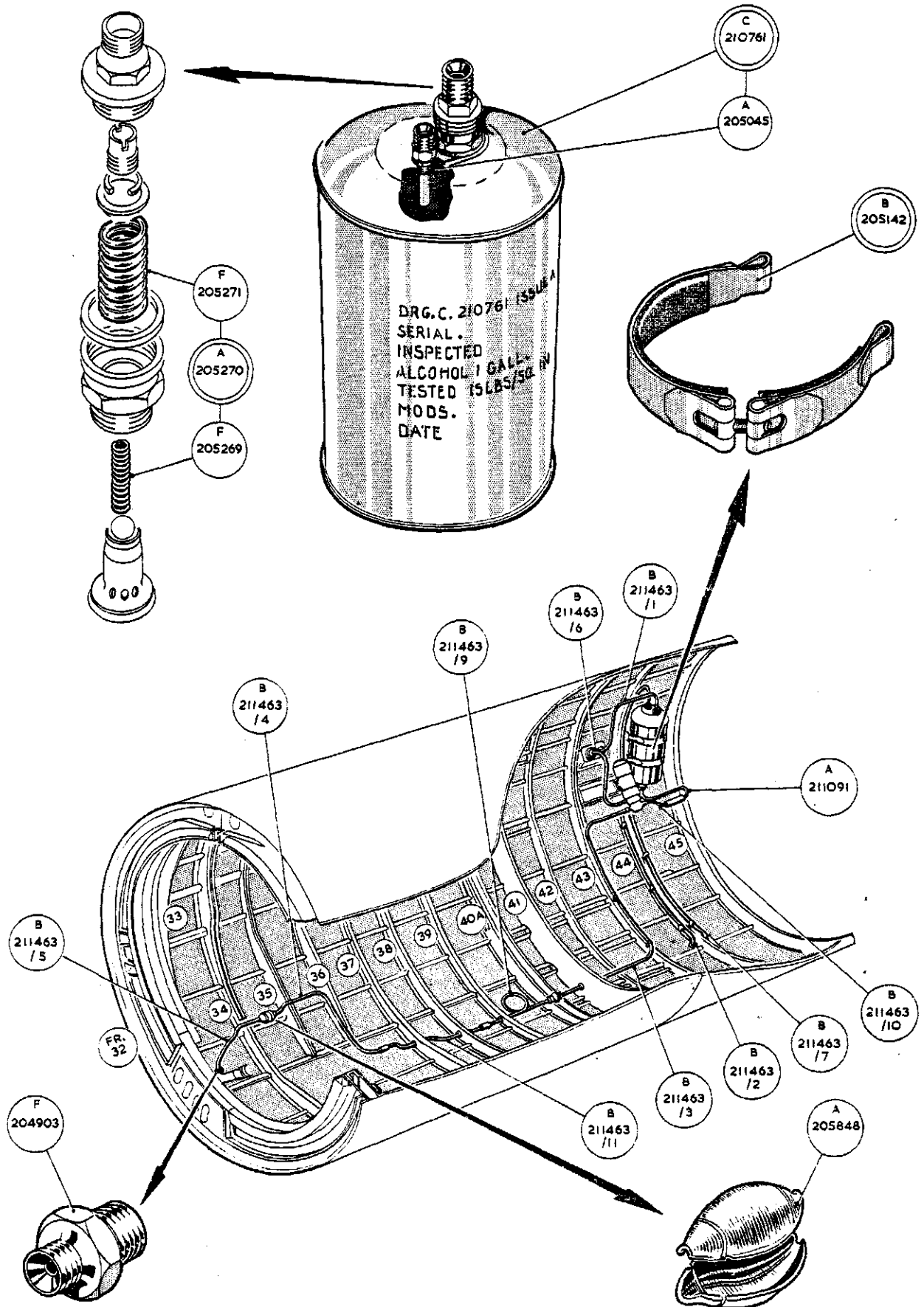
FUEL FILTER DE-ICING SYSTEM
