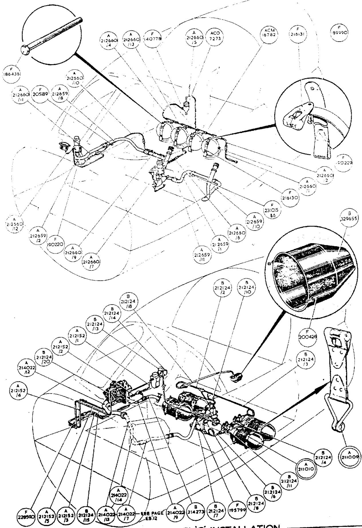
OXYGEN & ANTI 'G' INSTALLATION
