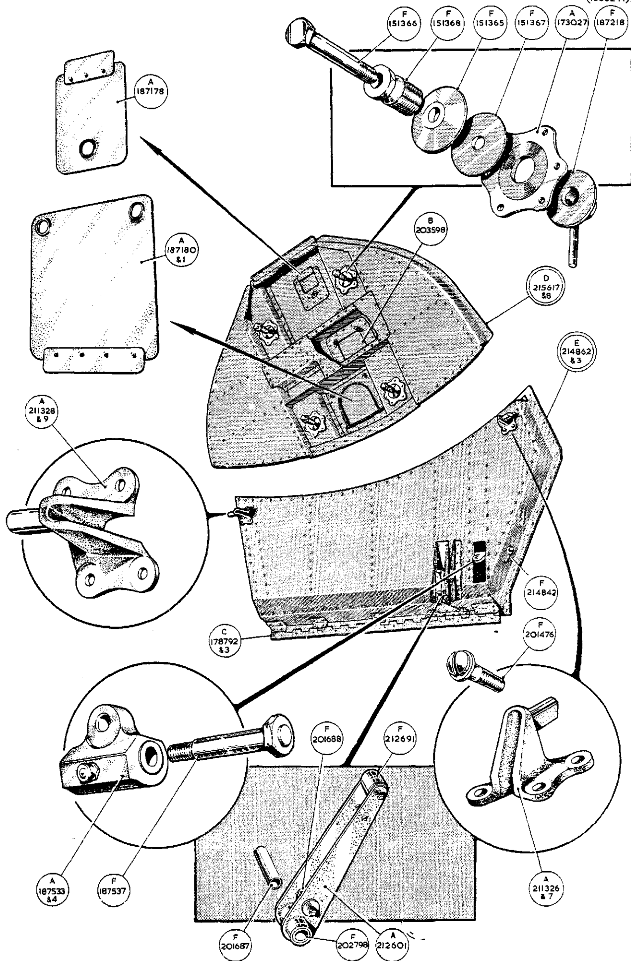
MAIN UNDERCARRIAGE
