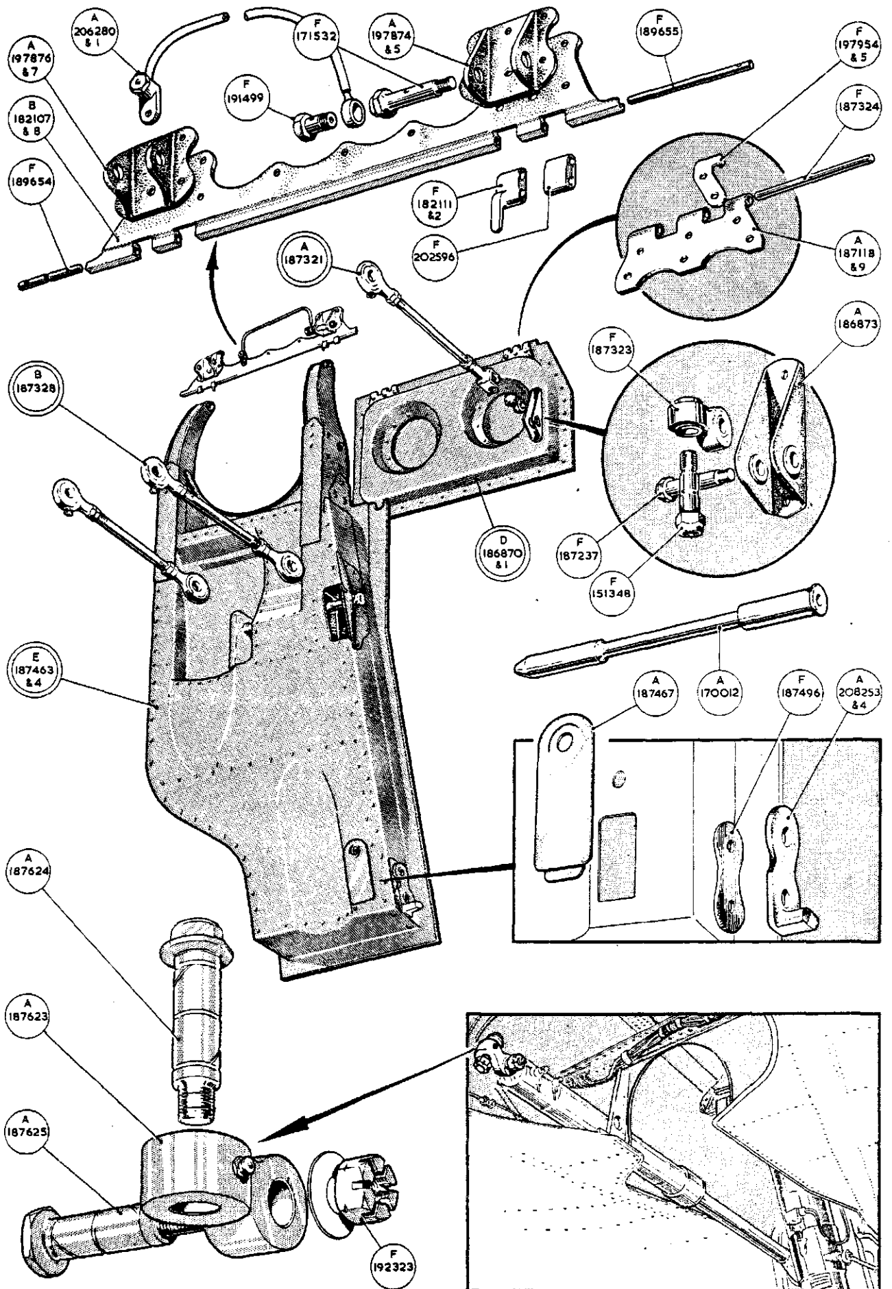
MAIN UNDERCARRIAGE
