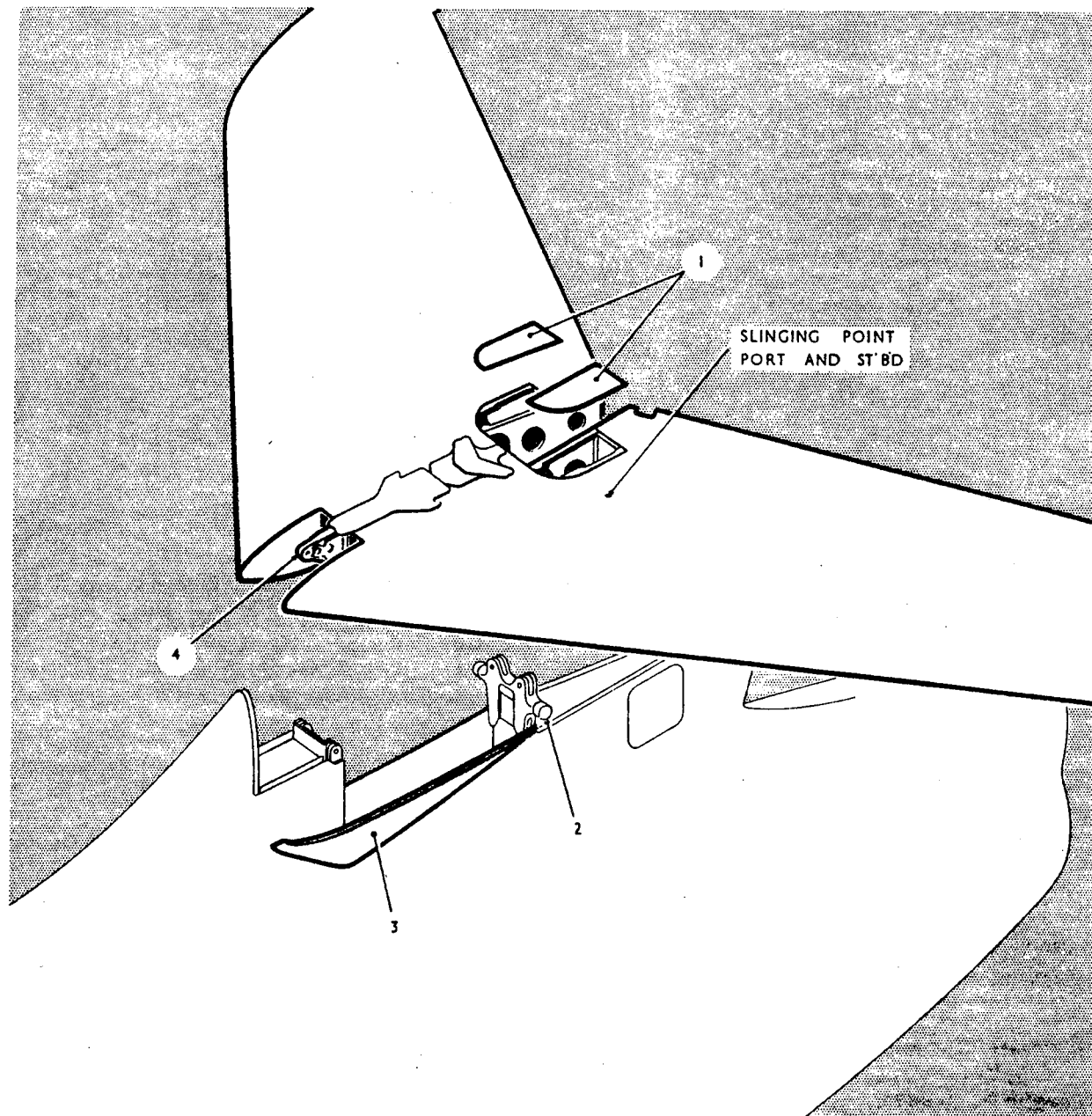
Fig. 10. Removal of tail plane
