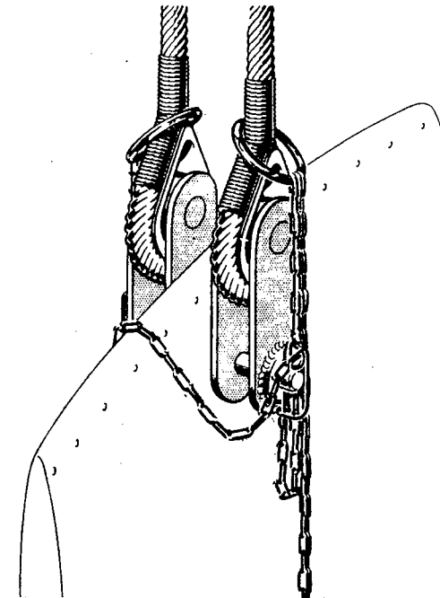
Fig. 4 Attachment of rudder sling
