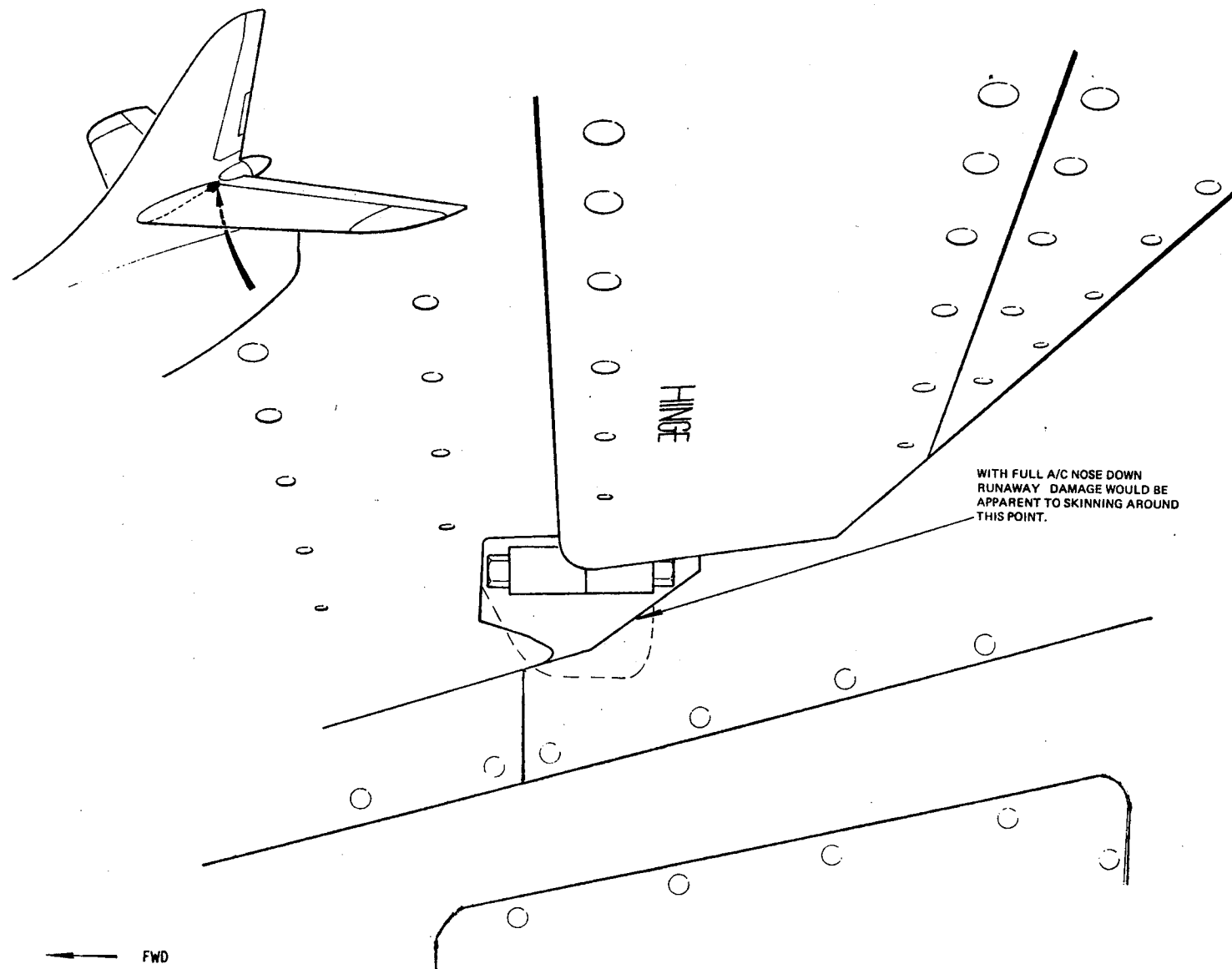
VIEW ON UNDERSIDE INBOARD PORT ELEVATOR
