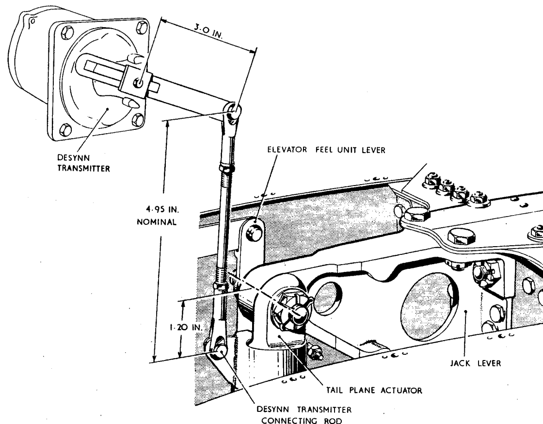
Fig. 11 Attachment of jack lever to tail plane actuator
