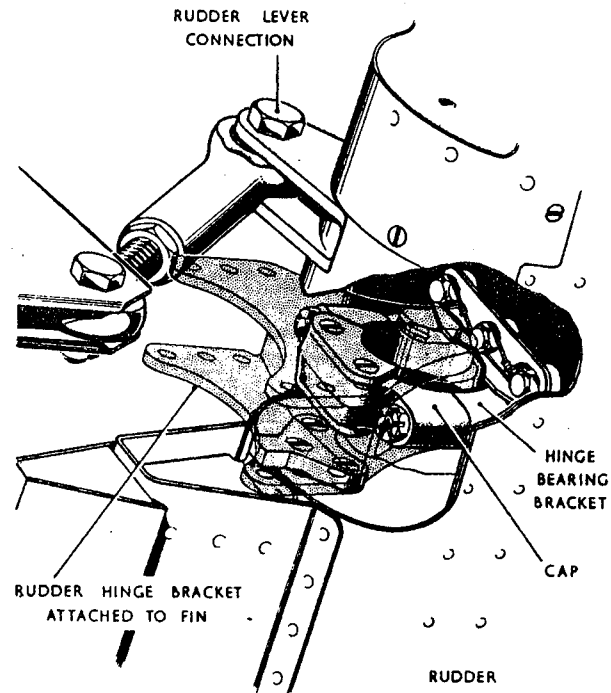
Fig. 3 Rudder operating lever and bottom hinge
