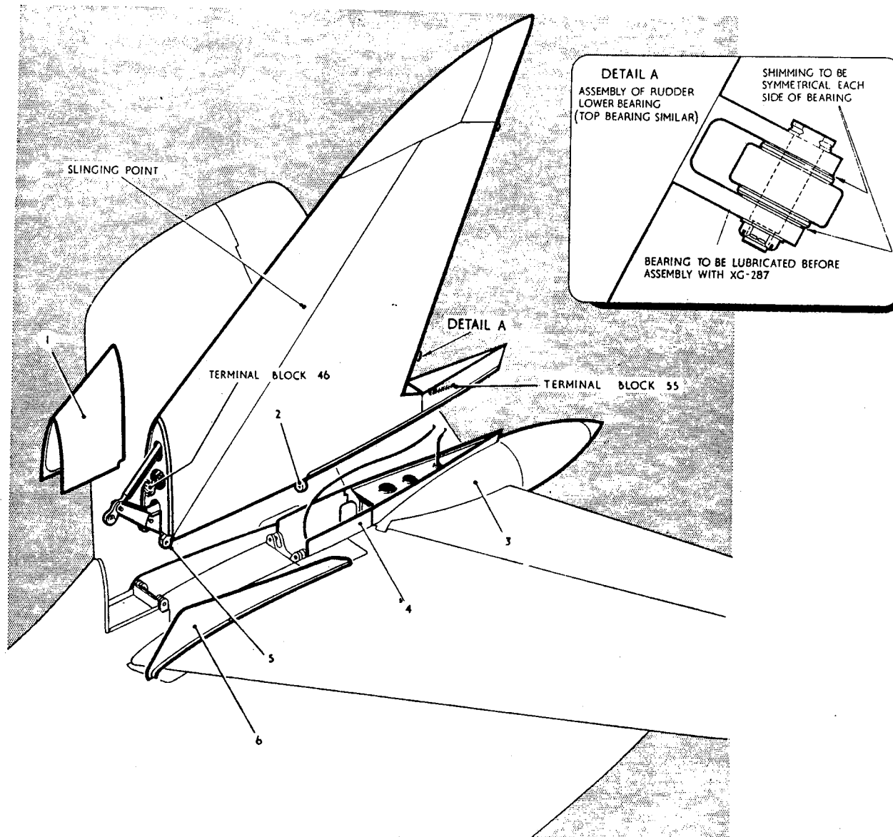
Fig.5. Removal of fin
