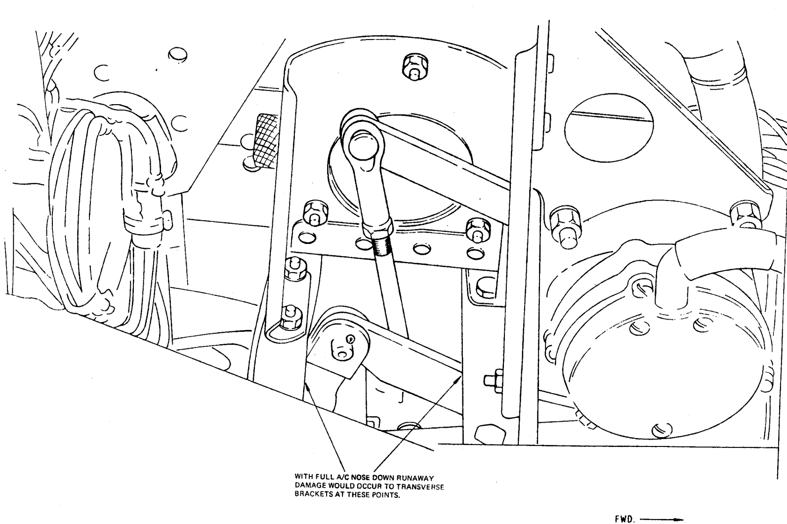
VIEW ON STBD. SIDE OF FIN SHOWING DESYNN CONTROL ACCESS PANEL REMOVED
