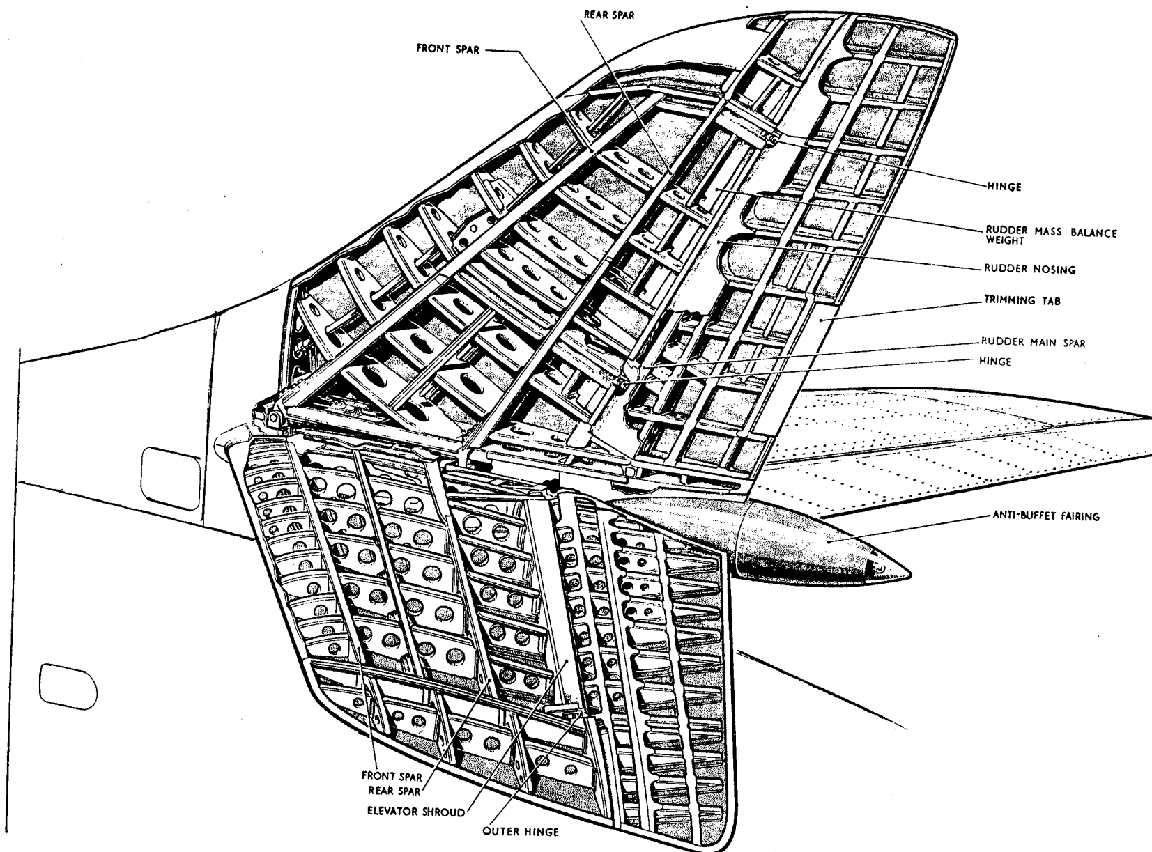
Fig. 1 Tail unit
