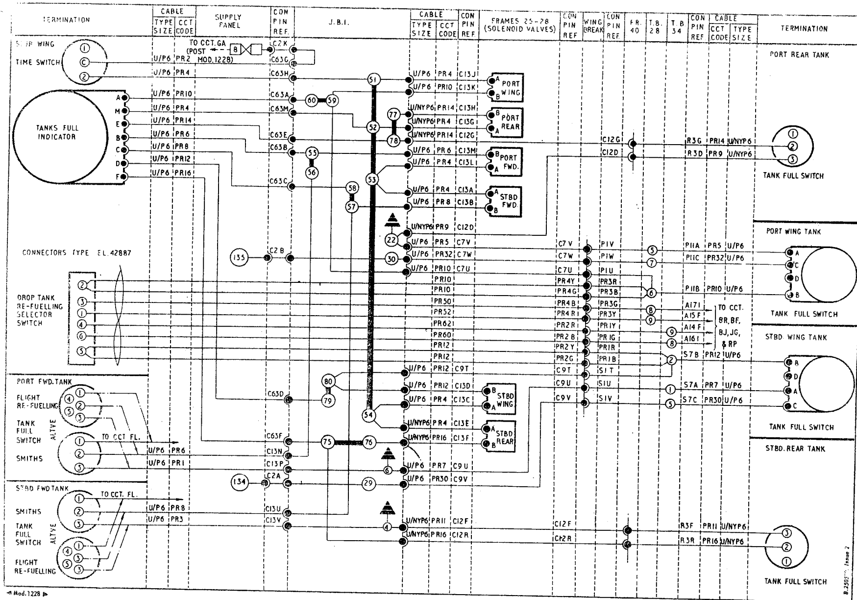
Fig.3 Pressure refuelling (routeing) RESTRICTED
