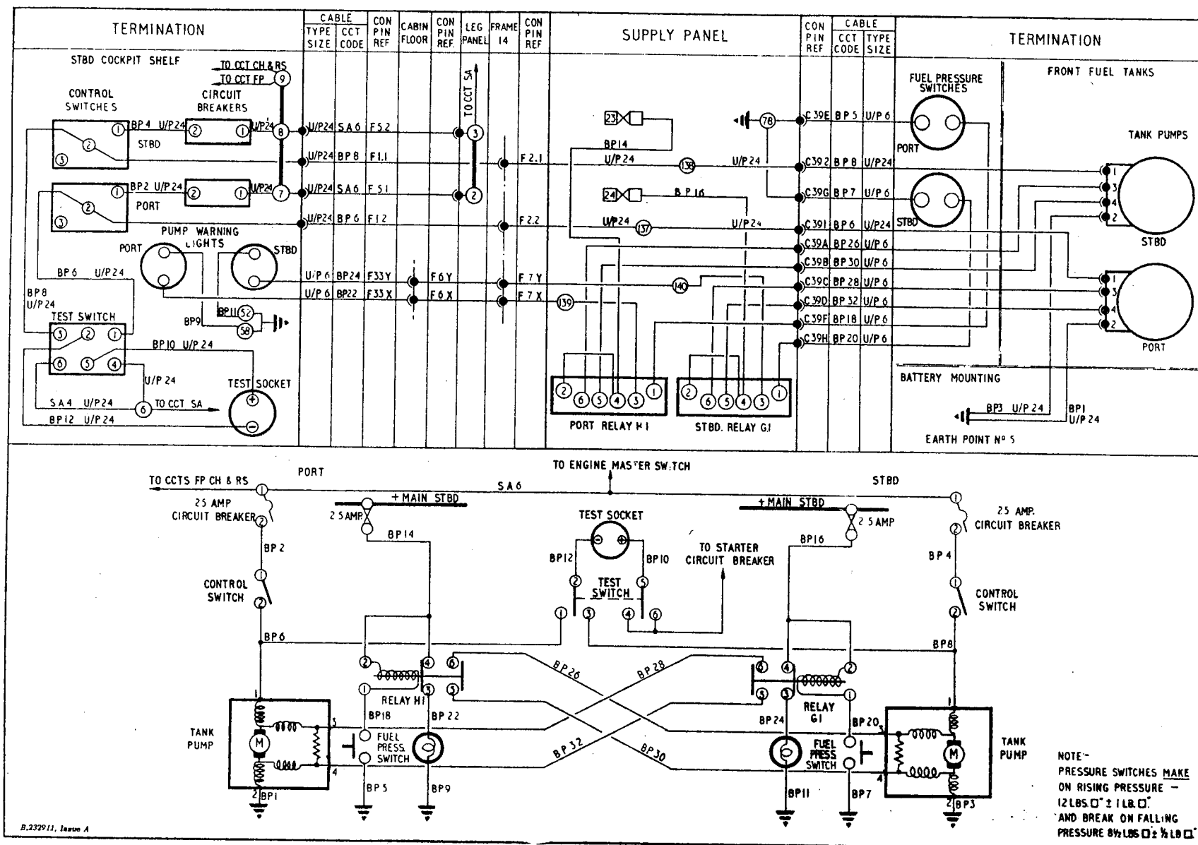
Fig.1. Tank pumps RESTRICTED
