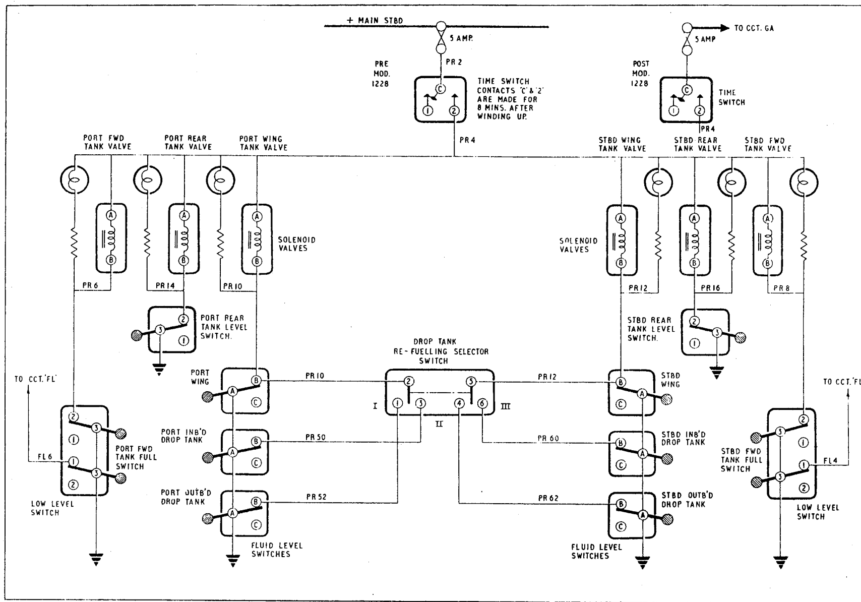
Fig.2. Pressure refuelling (theoretical) RESTRICTED
