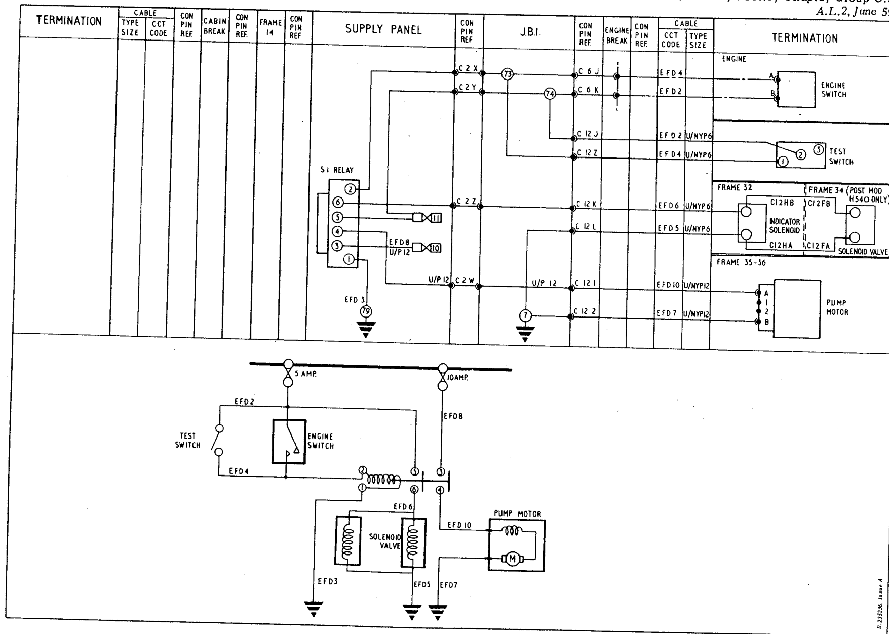
Fig.1. Fuel filter de-icing (routing and theoretical)
