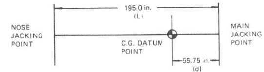
Fig. 1 Fixed dimensions
