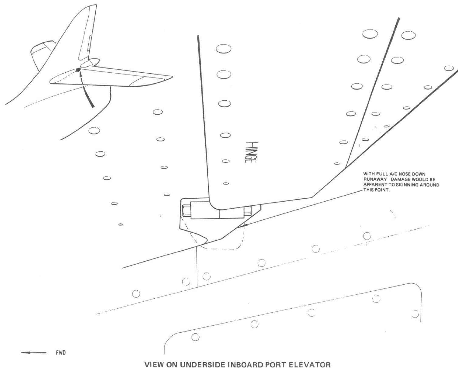
Fig.12 Tail plane inspection (1)
