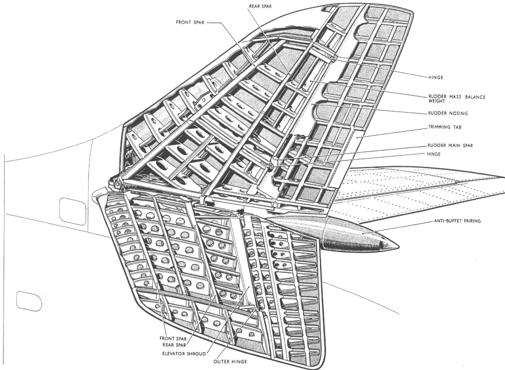
Fig. 1 Tail unit
