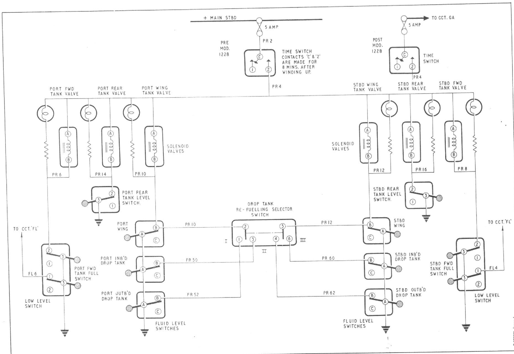
Fig.2. Pressure refuelling (theoretical) RESTRICTED
