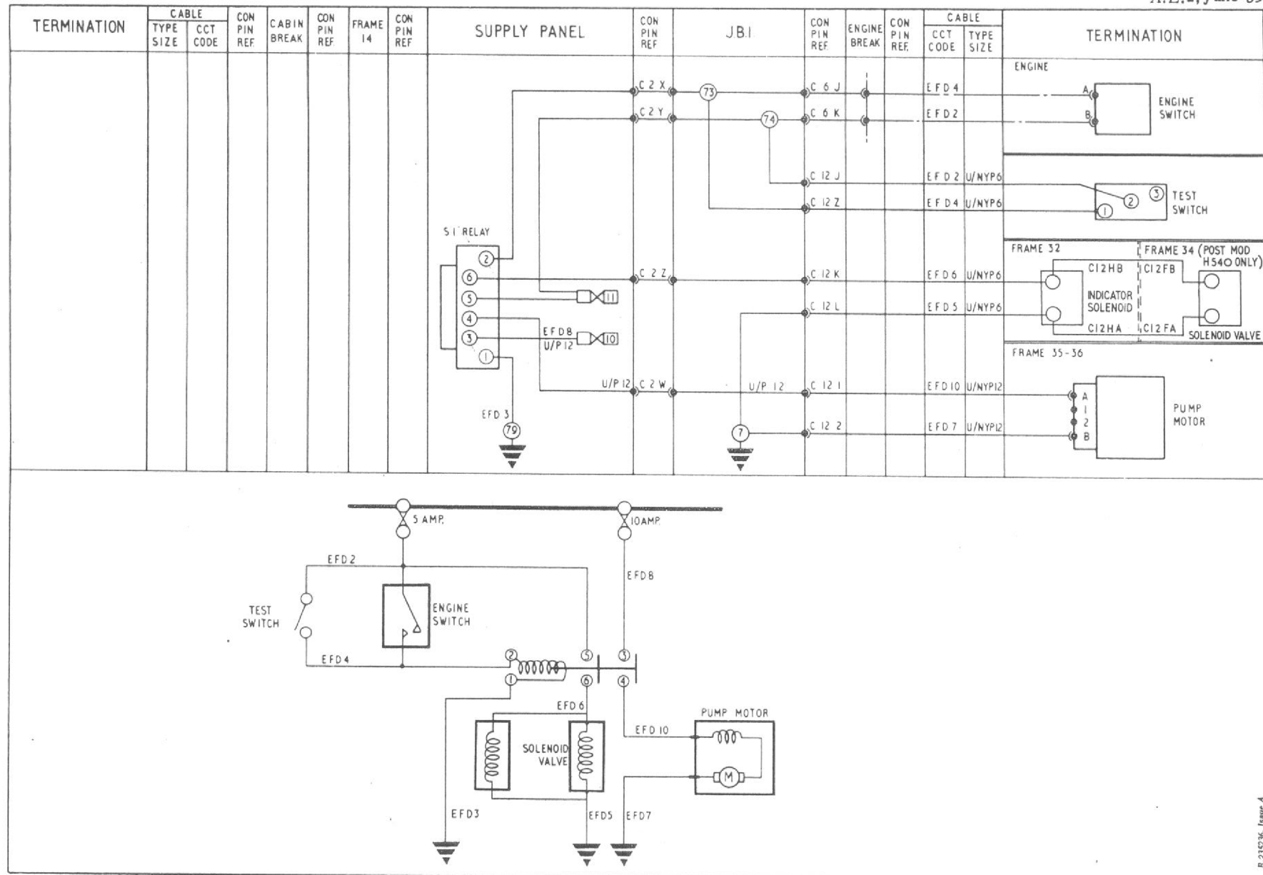
Fig.1. Fuel filter de-icing (routing and theoretical)
