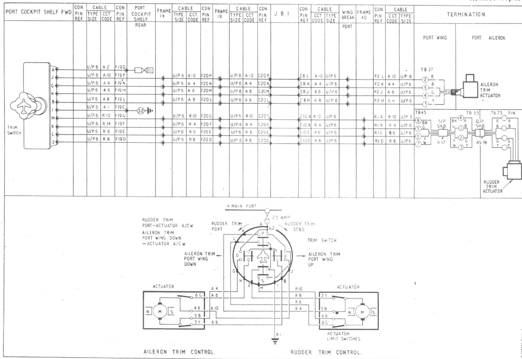
Fig.1. Rudder and aileron trim control (routeing and theoretical)
