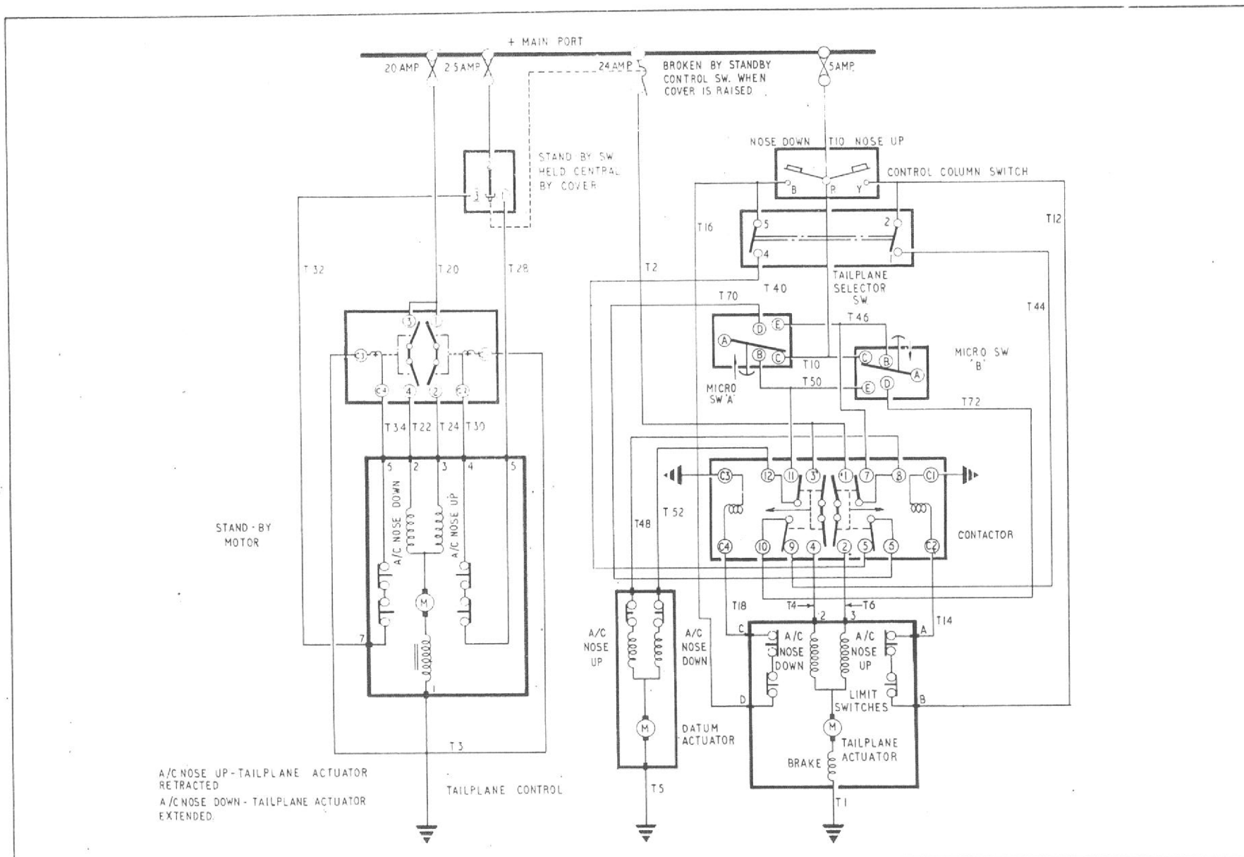
Fig.2. Tail plane control (theoretical) RESTRICTED
