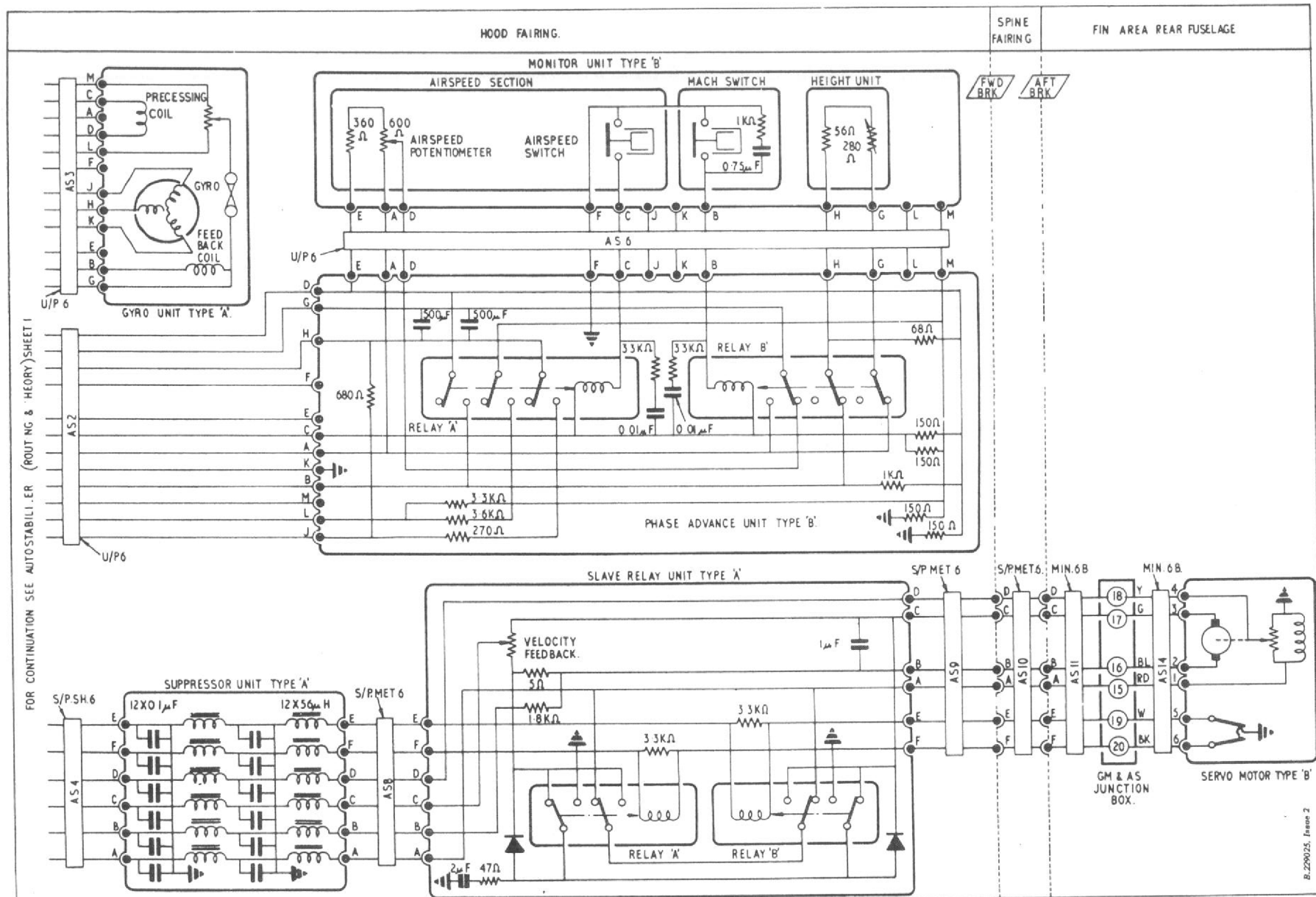
Fig.2. Autostabilizer (sheet 2)
