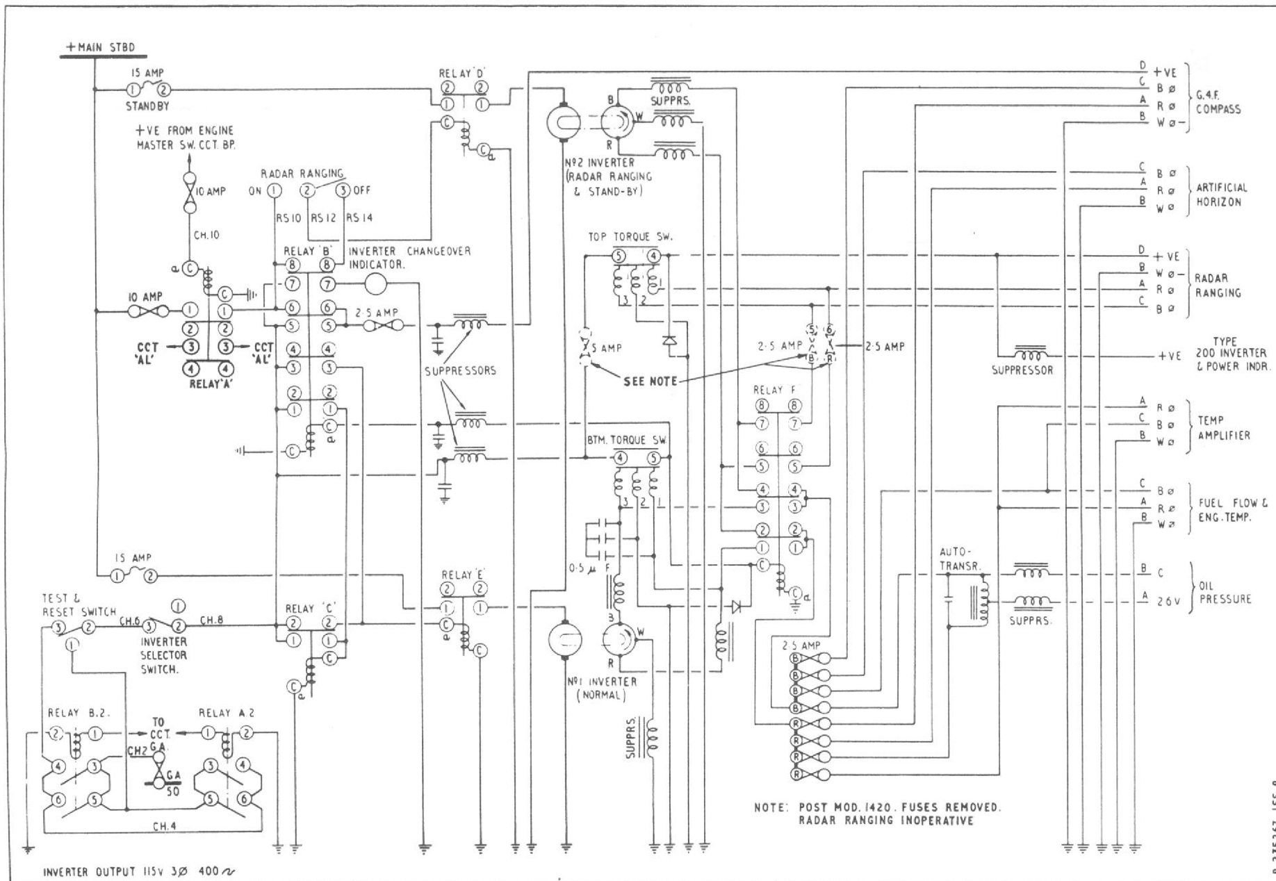
Fig. 3 A.C. supplies theoretical (post Mod.1375)
