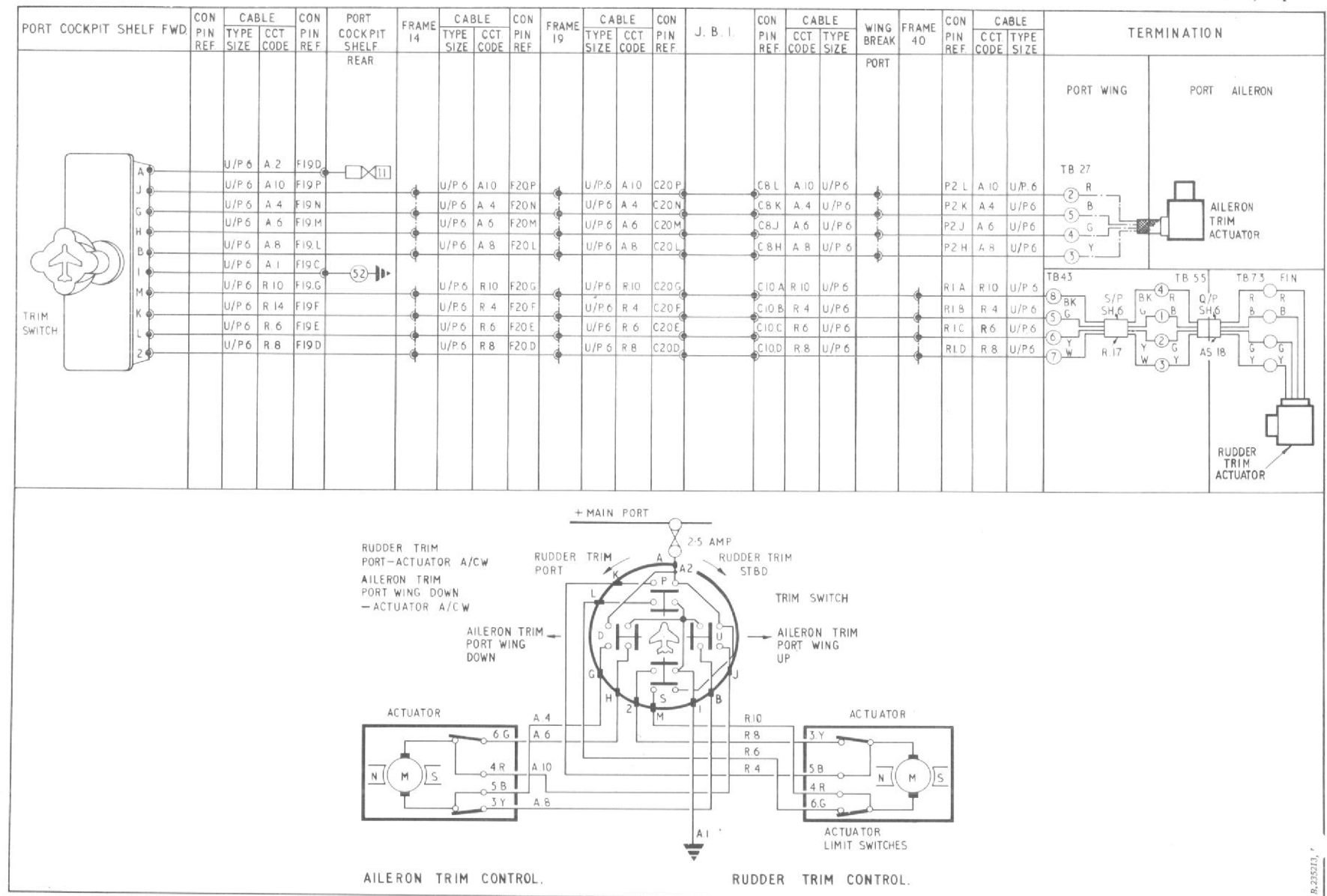
Fig.1. Rudder and aileron trim control (routing and theoretical)
