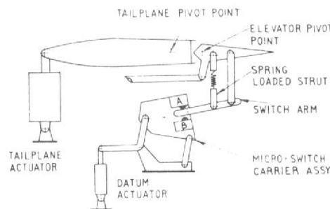
Fig.1 Tail plane and elevator linkage
