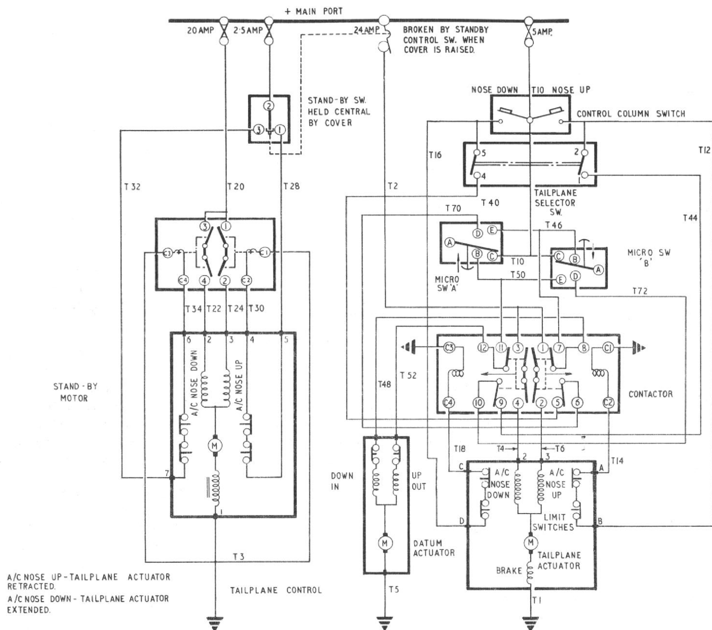
Fig.2. Tail plane control (theoretical)
