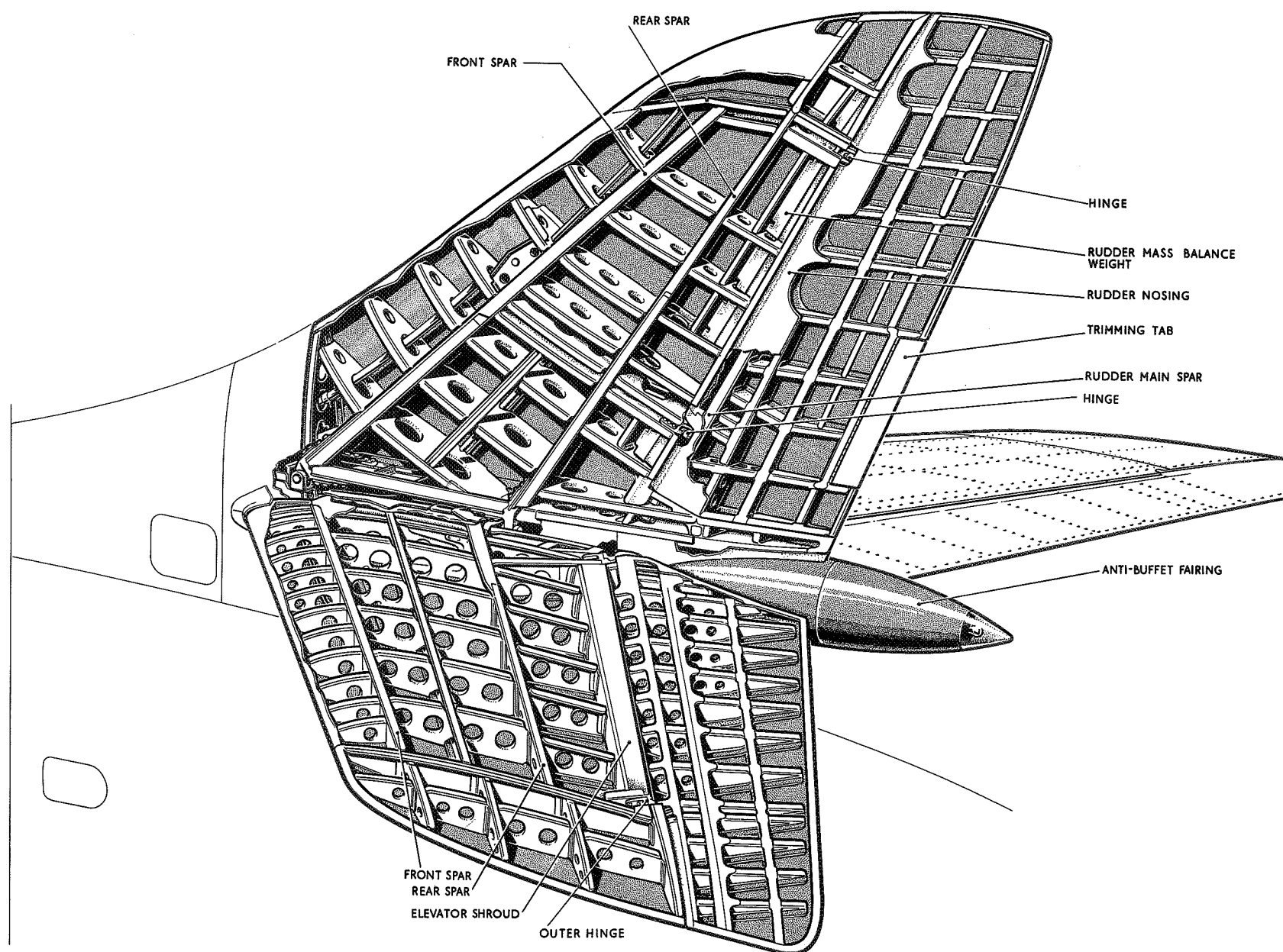
Fig. 1 Tail unit
