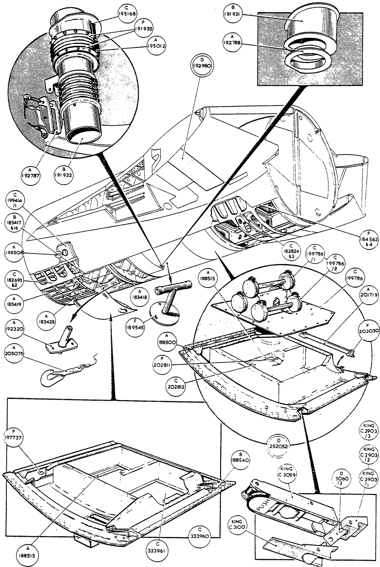
CENTRE FUSELAGE
