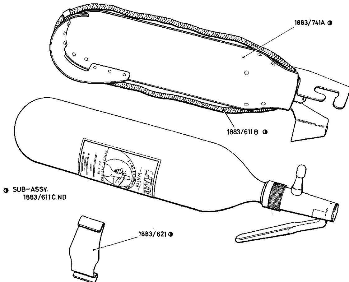
FIRE EXTINGUISHER & MOUNTING (REF DRG 1883/611A)
