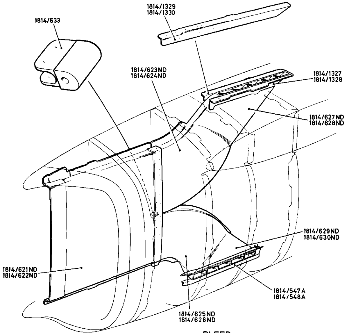
BLEED ASSEMBLY BOUNDARY LAYER (REF. DRG. 1814/11-12A)
