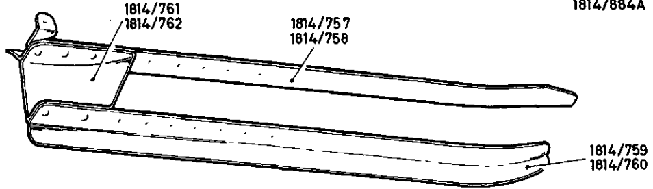
COLLAR, ASSEMBLY, BOTTOM BLEED EXIT REF. DRG. 1814/547A 1814/548A
