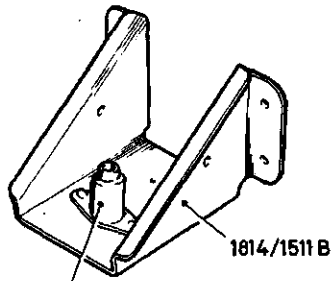
F.1968/3 (KEYLOCK) BRACKET, ASSEMBLY REF. DRG. 1814/1511A
