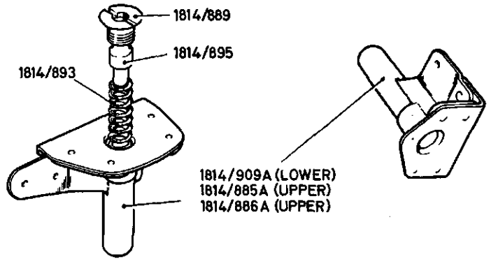
CATCH, ASSEMBLY, GROUND RUNNING INLET REF. DRG. 1814/883A 1814/884A
