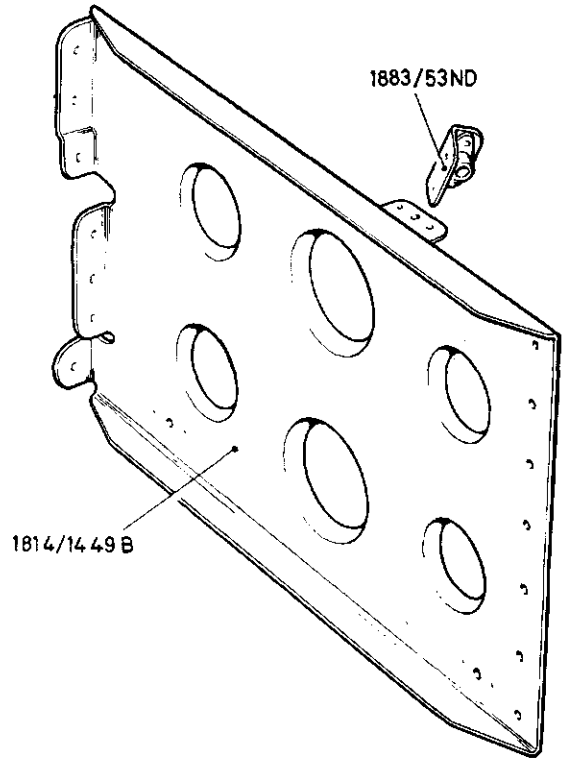
MOUNTING ASSEMBLY, CENTRALISED WARNING (BETWEEN FRAMES 10 - 11) REF. DRG. 1814/1449A
