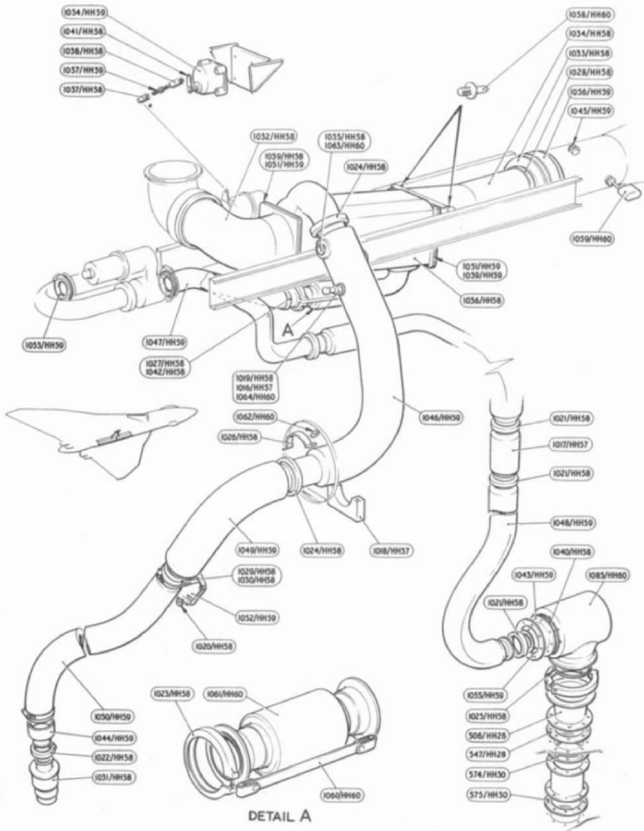
EQUIPMENT SPECIAL OPERATIONAL STORE HEATING EQUIPMENT
