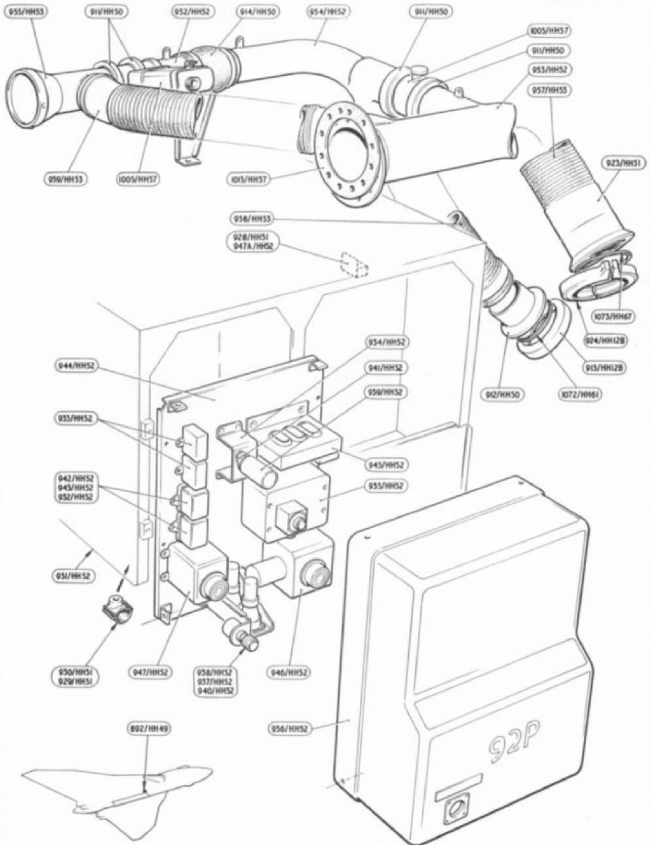
EQUIPMENT SPECIAL OPERATIONAL HYDRAULIC UNIT-COOLING SYSTEM & PANEL 92.
