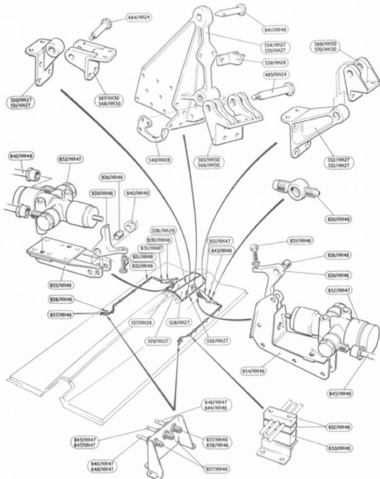
EQUIPMENT SPECIAL OPERATIONAL FIN GAP DOORS & HYDRAULIC EQUIPMENT
