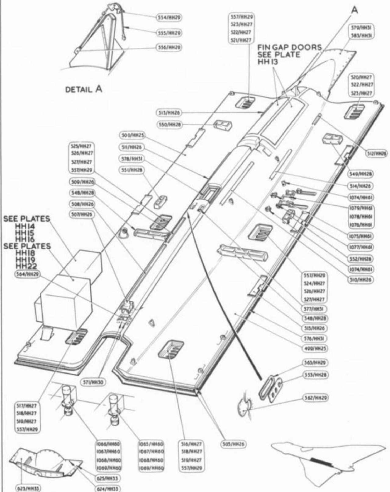
EQUIPMENT SPECIAL OPERATIONAL FAIRING DOORS
