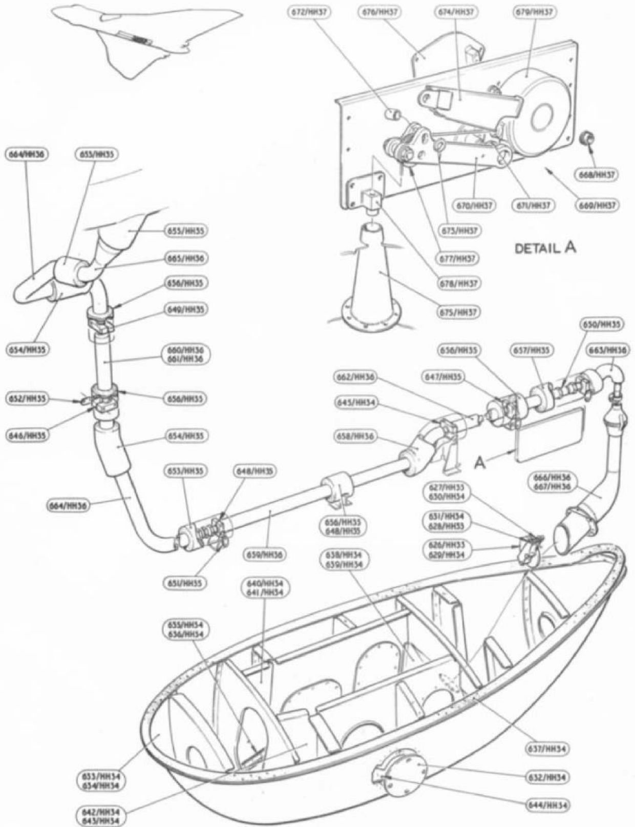
EQUIPMENT SPECIAL OPERATIONAL A.L.S.U. FAIRING & SERVICES
