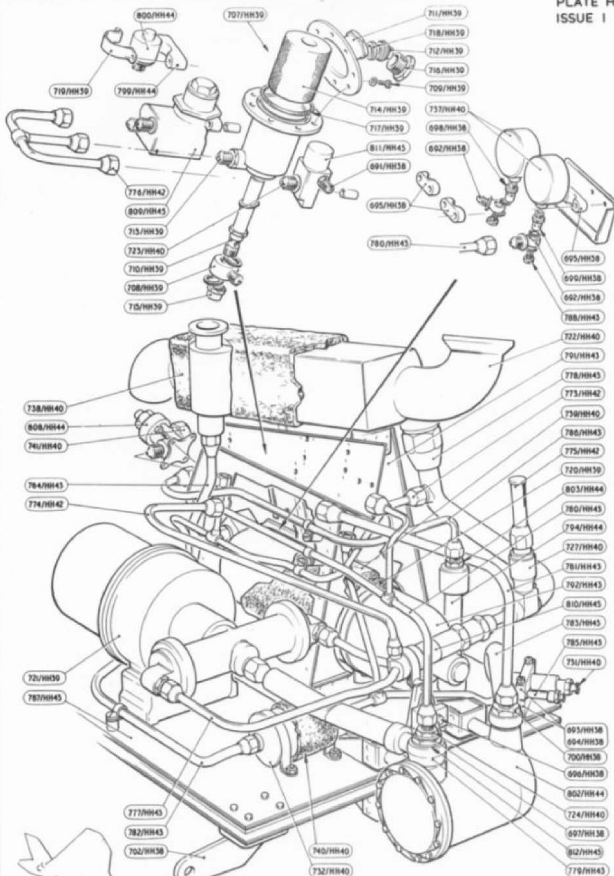
EQUIPMENT SPECIAL OPERATIONAL REFRIGERATION PACK
