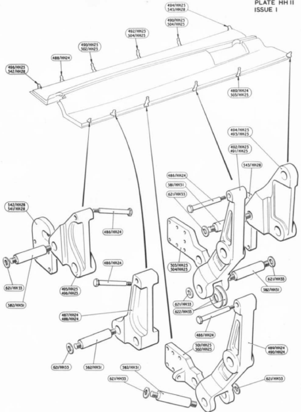
EQUIPMENT SPECIAL OPERATIONAL FAIRING DOOR HINGES
