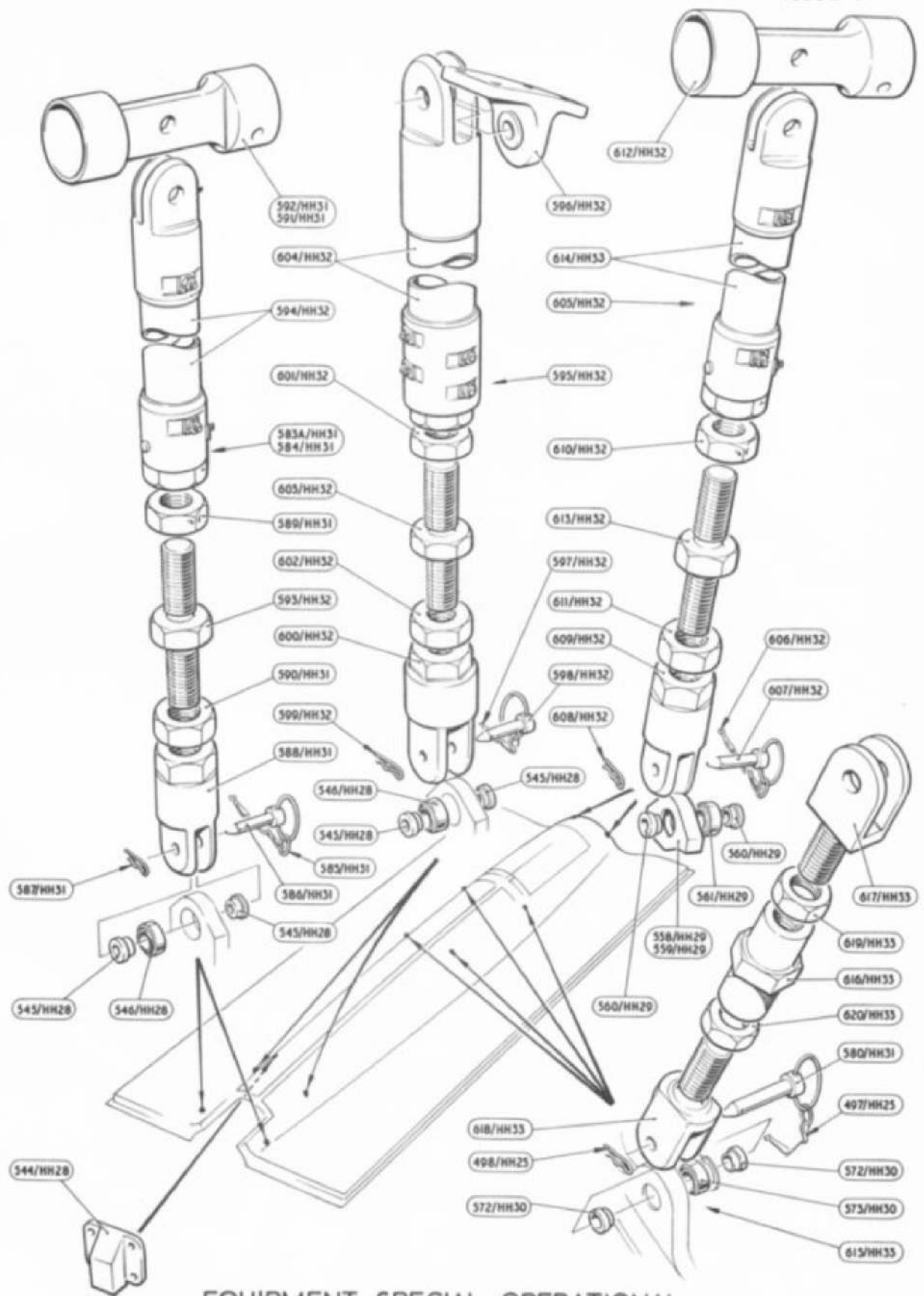
EQUIPMENT SPECIAL OPERATIONAL FAIRING DOOR SUPPORTS
