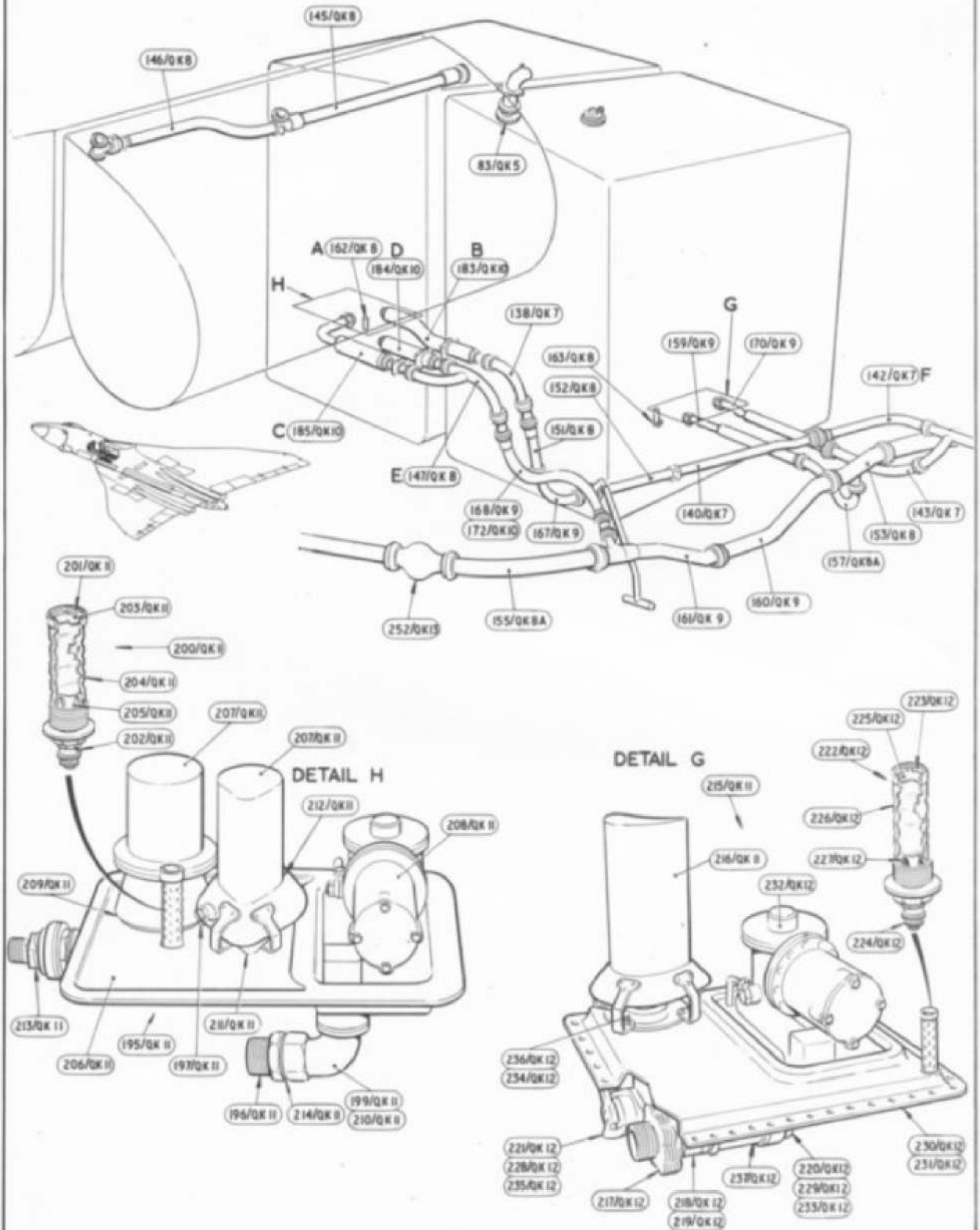
FUEL SYSTEM No.1 AND 2 TANKS IN FUSELAGE
