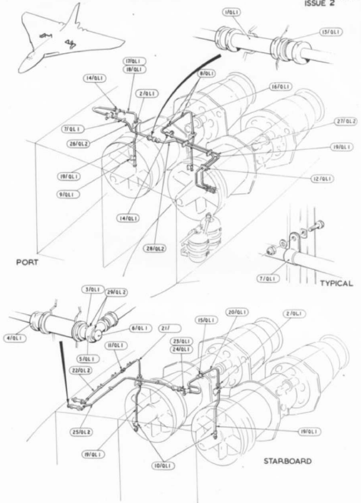
FUEL SYSTEM FUSELAGE CENTRE SECTION
