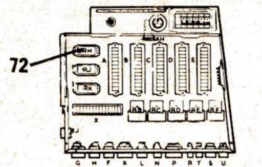
DISTRIBUTION PANEL DP
