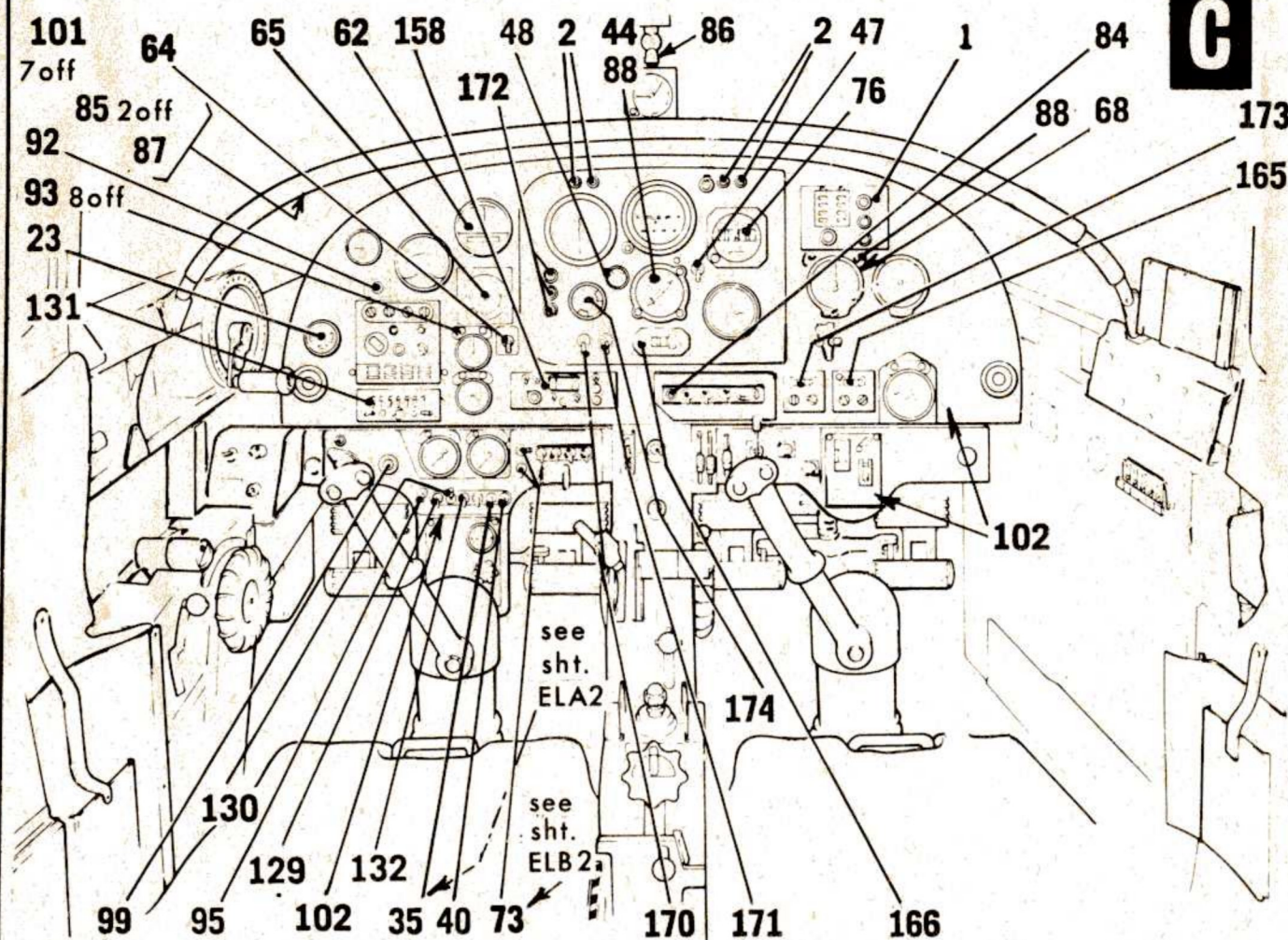
COCKPIT
