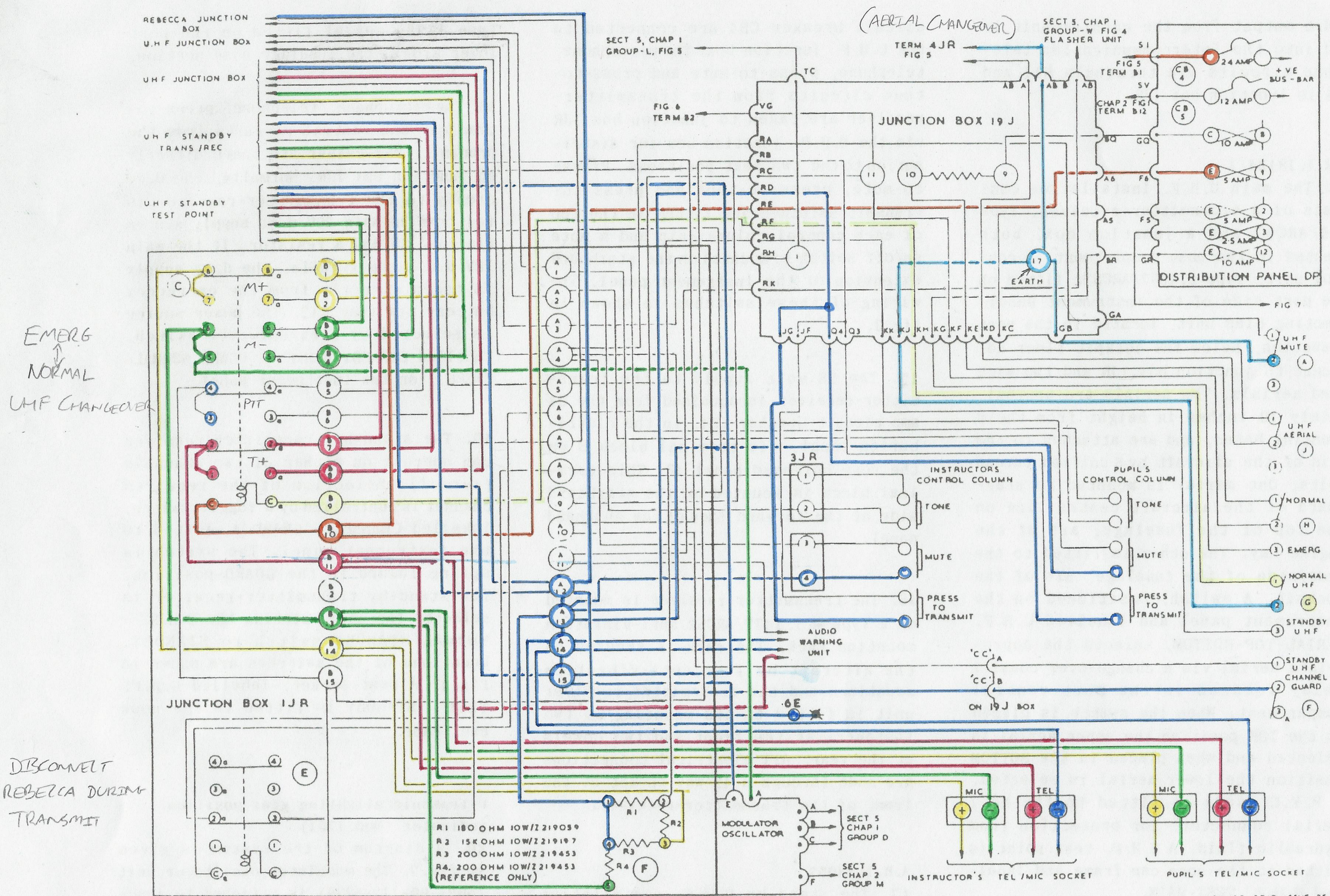
FIG. 3. INTERCOMMUNICATION AND RADIO SUPPLIES-THEORETICAL DIAGRAM ◀MOD 1701 ADDED▶
