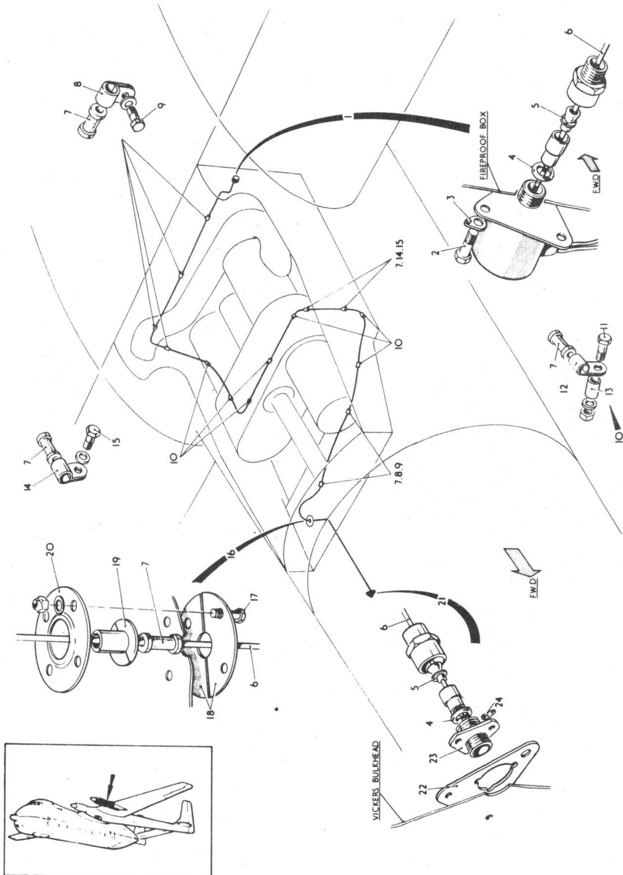
INSTALLATION REAR OF FIREPROOF BULKHEAD OUTBOARD (L.H)
