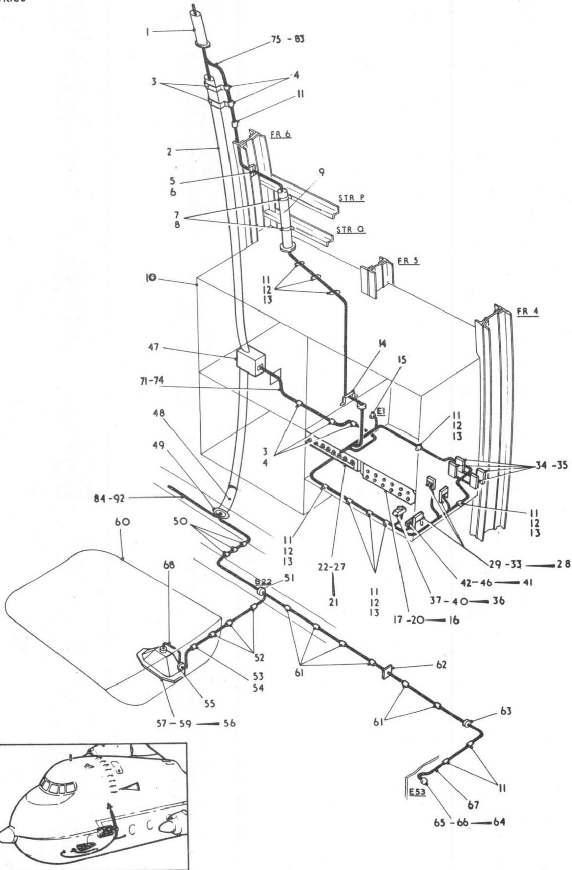
CABLE RUN TO FORWARD CRASH SWITCH FIGURE 2 RESTRICTED
