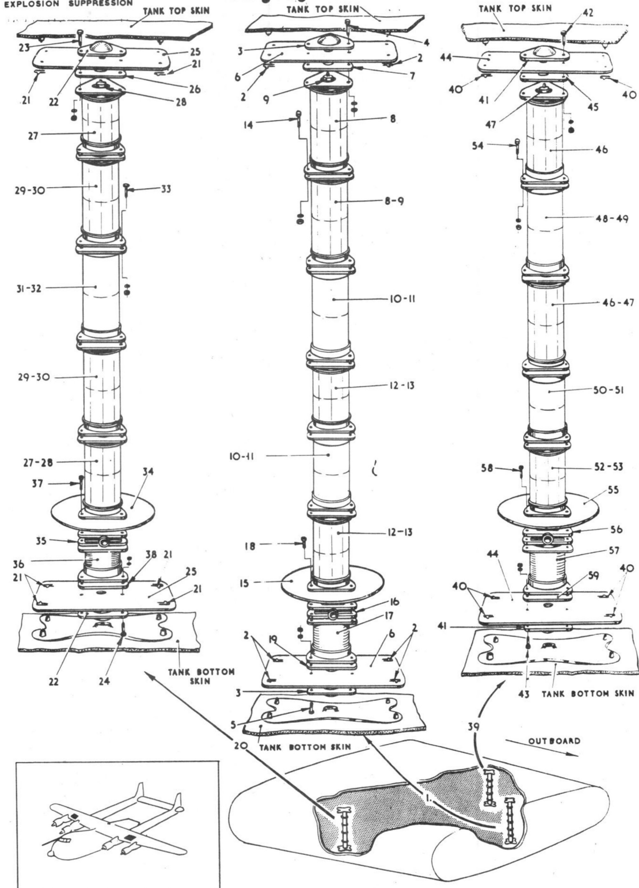
EXPLOSION SUPPRESSION No 2 TANK
