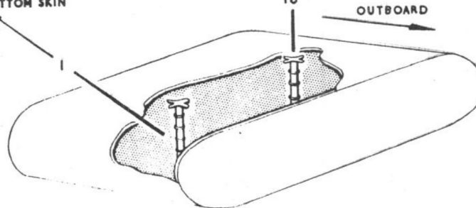
EXPLOSION SUPPRESSION AUXILIARY TANK
