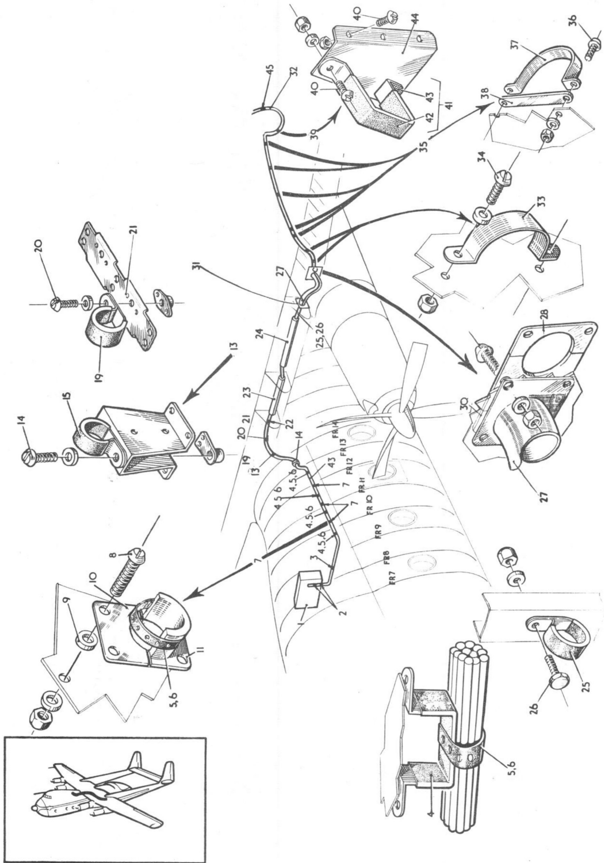
CABLE RUN FROM J1 TO BOOM (LH)
