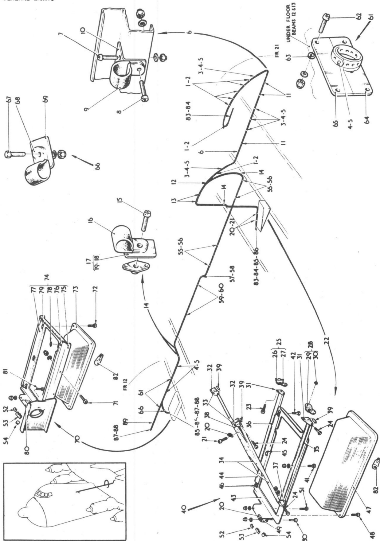
CABIN LIGHTS, FR. 21 TO FR.12 (R.H.)
