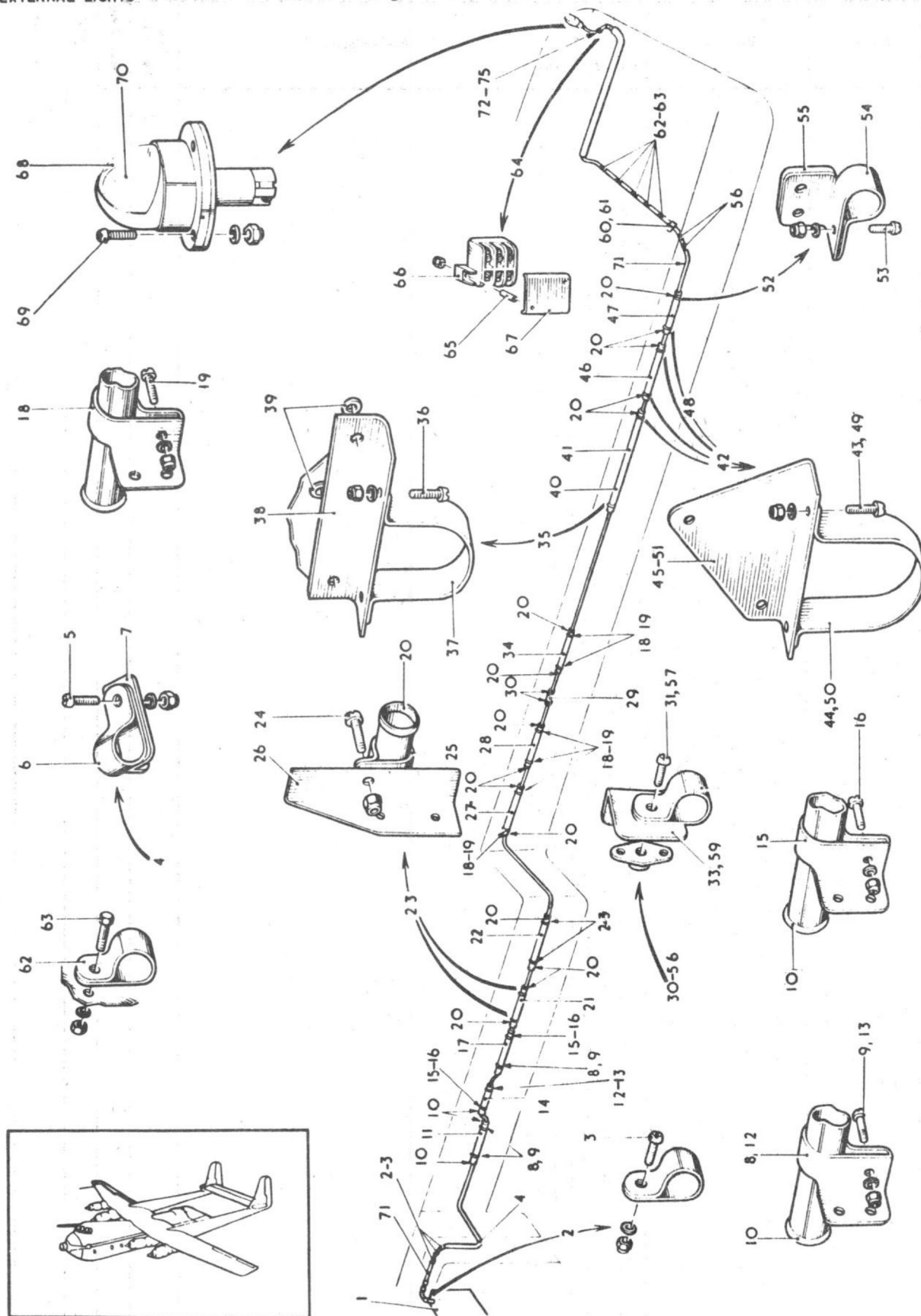
CABLE RUN IN WING (R.H.)
