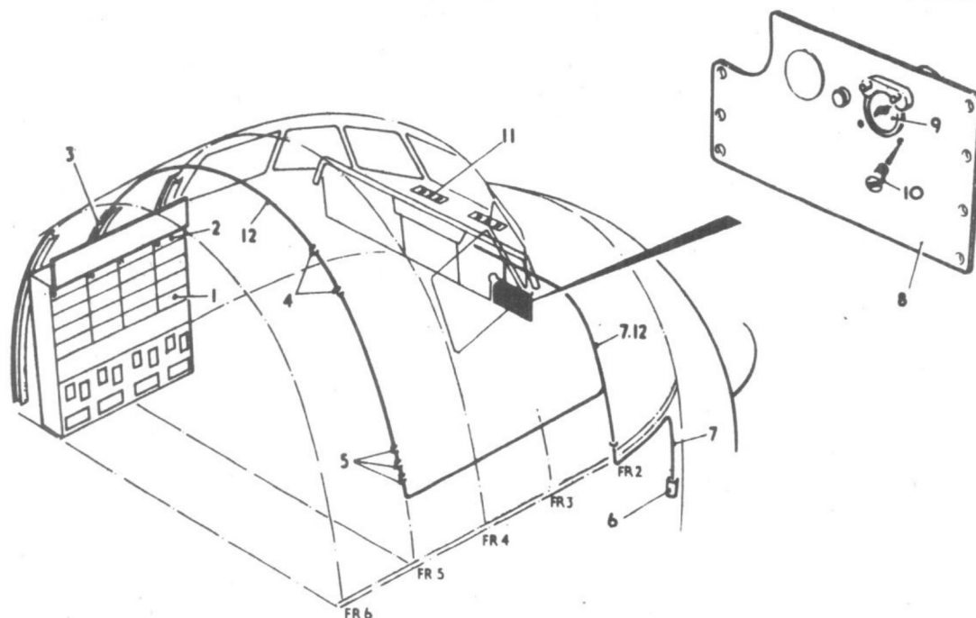
CABLE RUN TO OXYGEN PRESSURE GAUGE FIGURE 3
