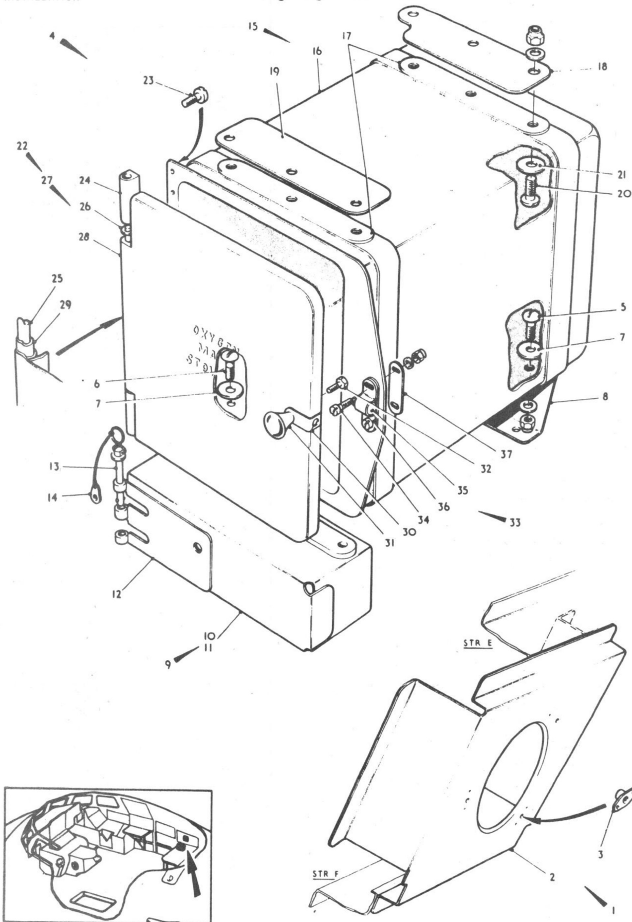
OXYGEN MASK STORAGE AND REGULATOR MOUNTING
