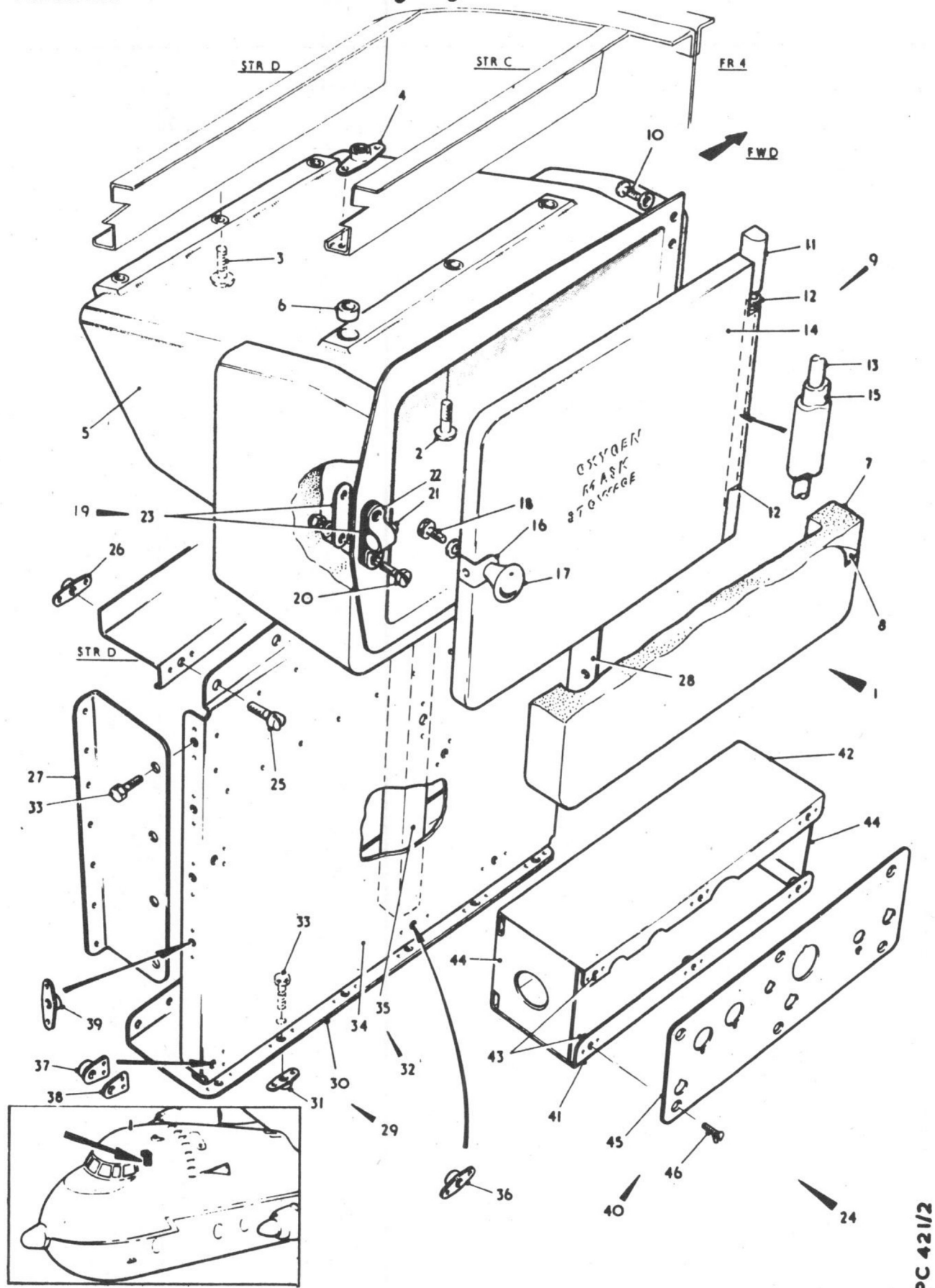
OXYGEN MASK STOWAGE AND REGULATOR MOUNTING FOR SUPERNUMERARY
