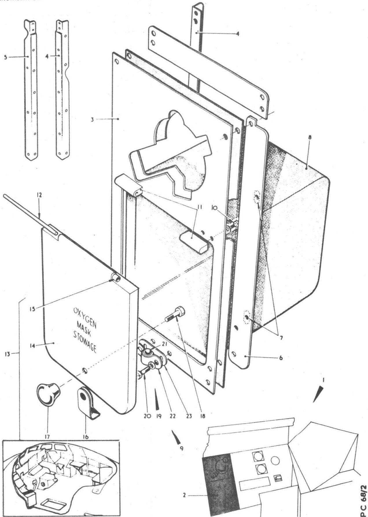
OXYGEN MASK PANEL ASSEMBLIES IN SIDE CONSOLES
