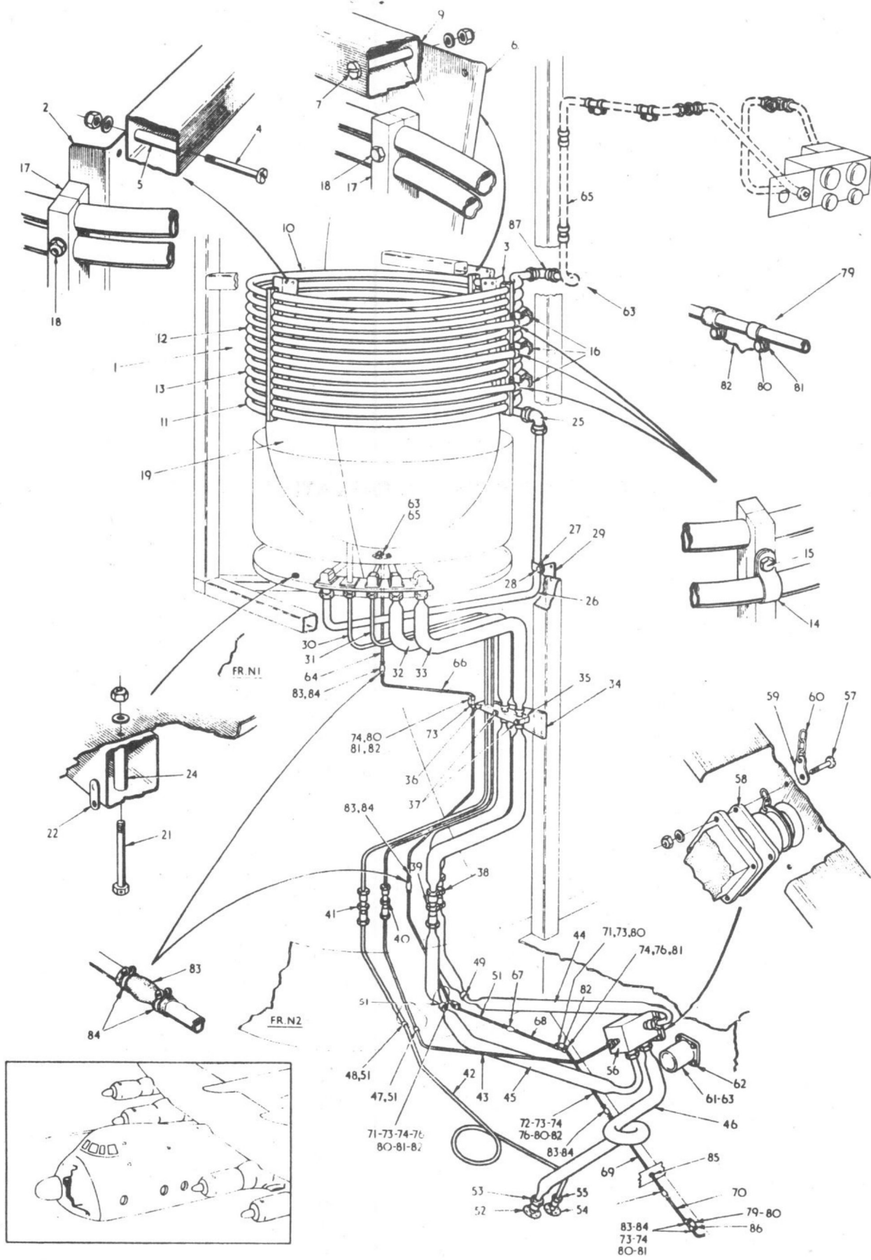
CONVERTER PACK MOUNTING & ASSEMBLY FIGURE I
