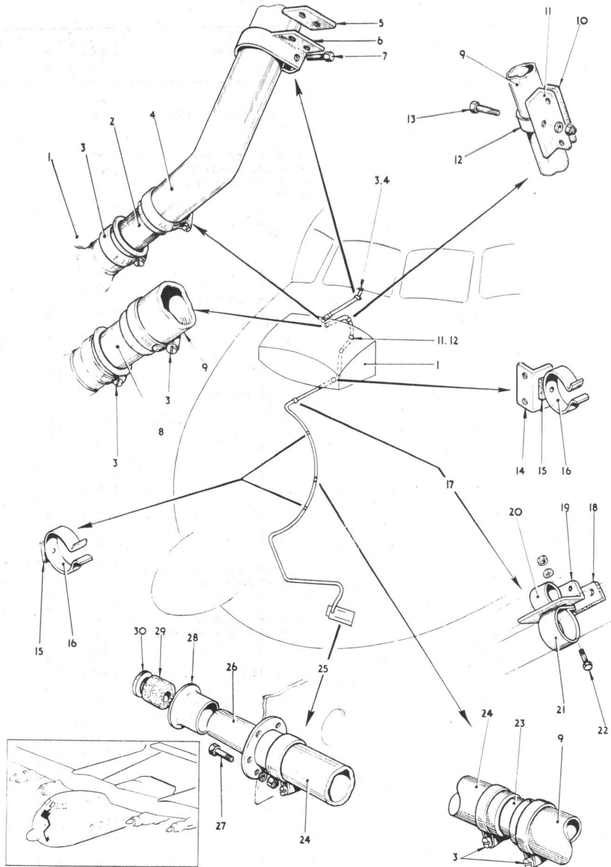
VENT & OVERFLOW (FRESH WATER TANK)
