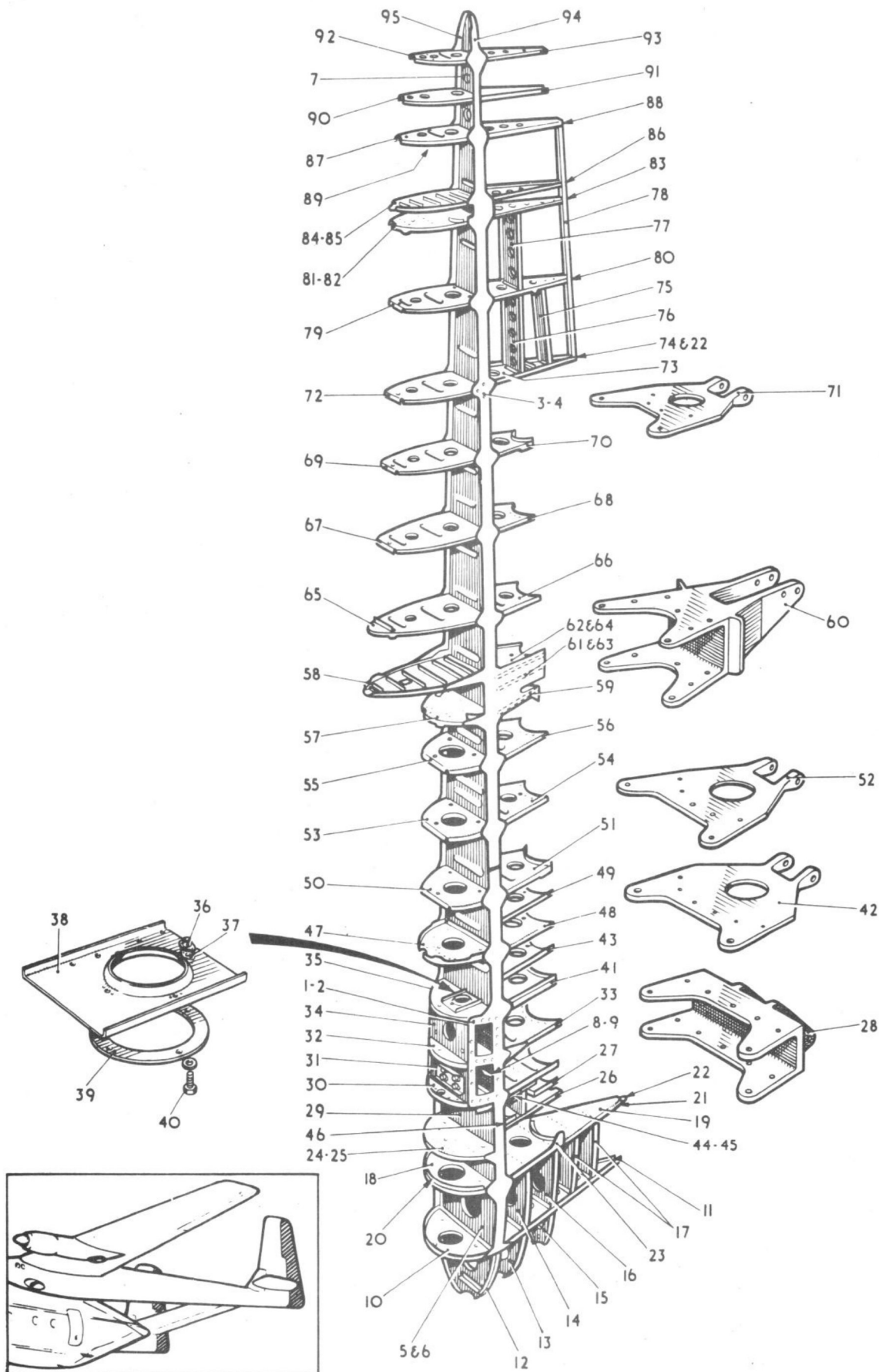
RUDDER ASSEMBLY STRUCTURE
