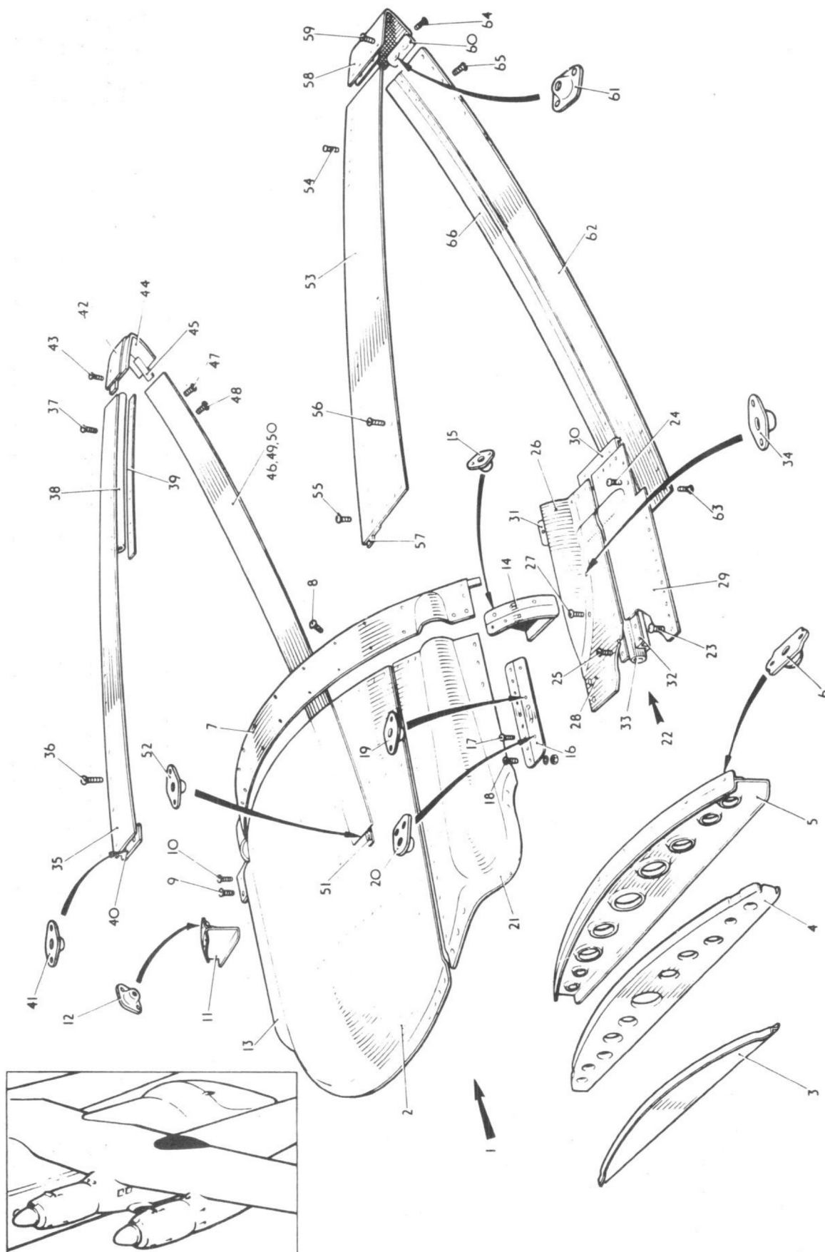
TAIL BOOM FAIRINGS
