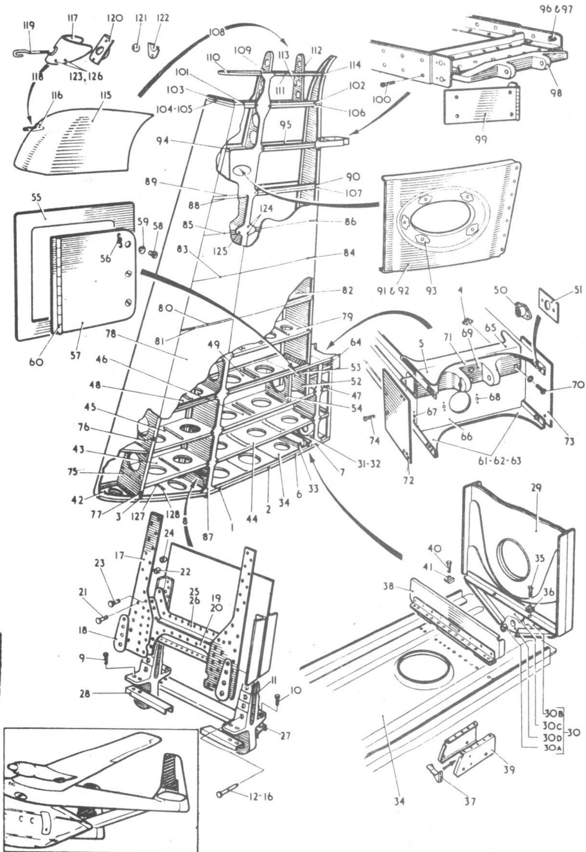
FIN ASSEMBLY, STRUCTURE
