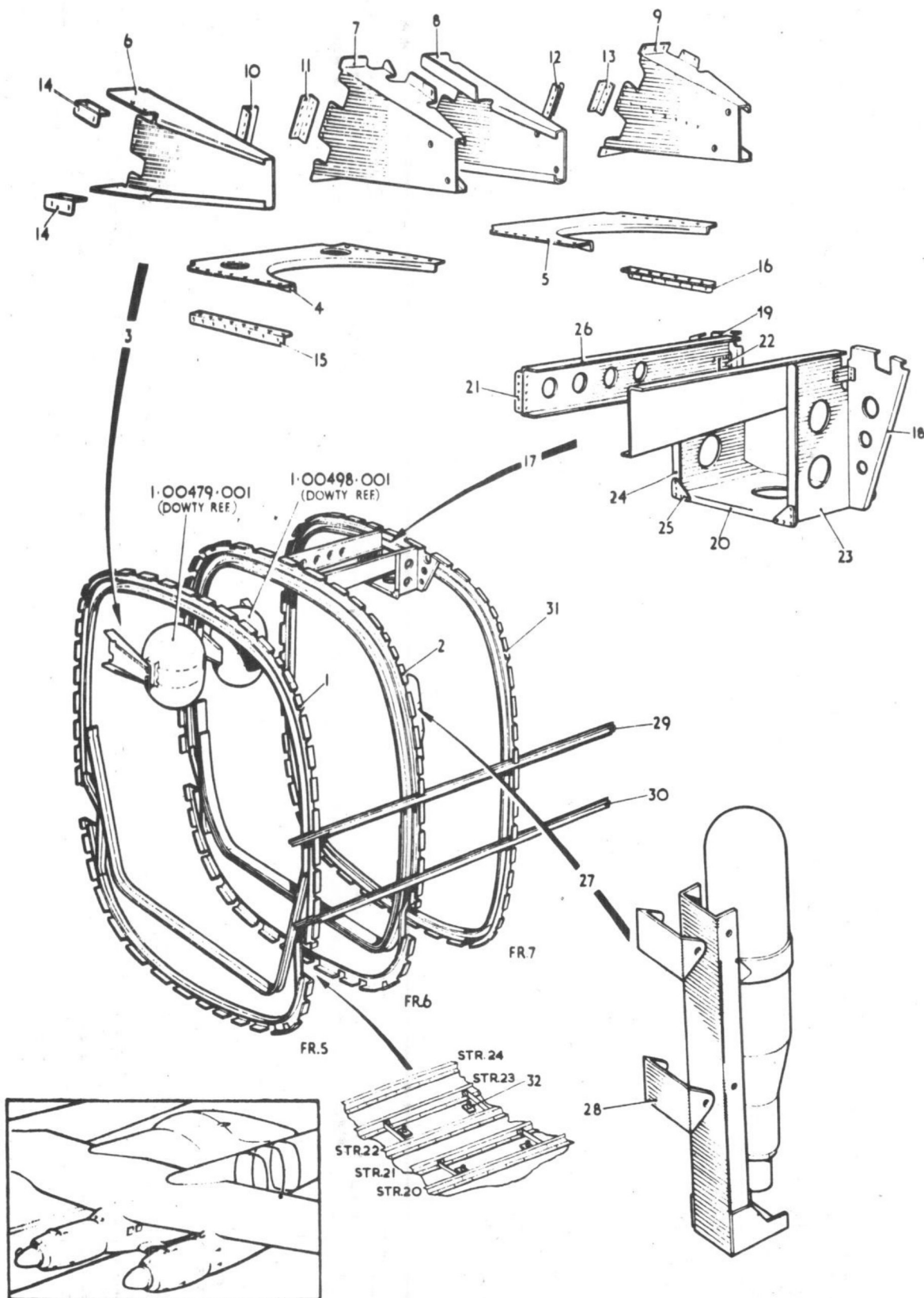
TAIL BOOMS FRAMES 5 TO 7
