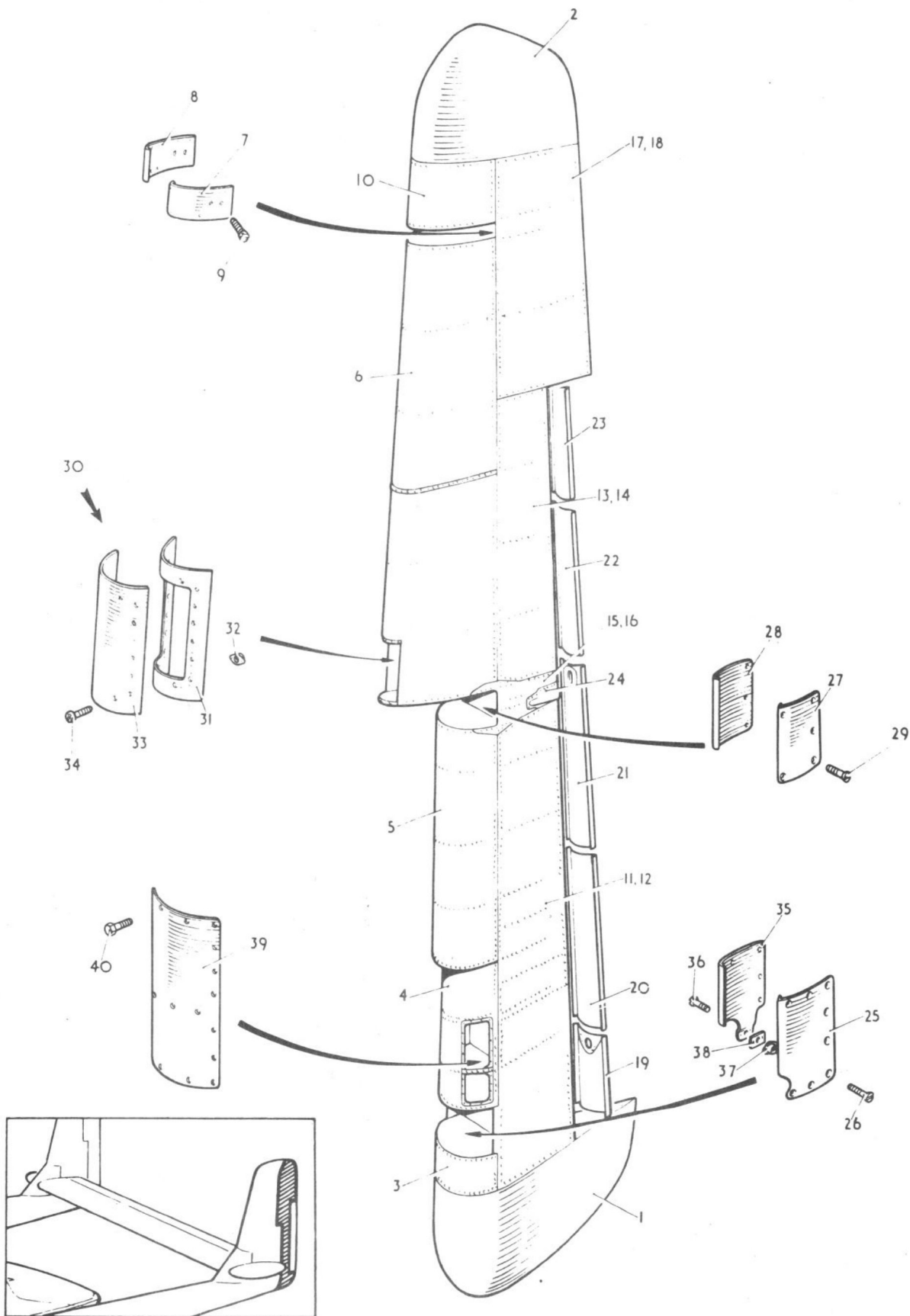
RUDDER ASSEMBLY SKINS
