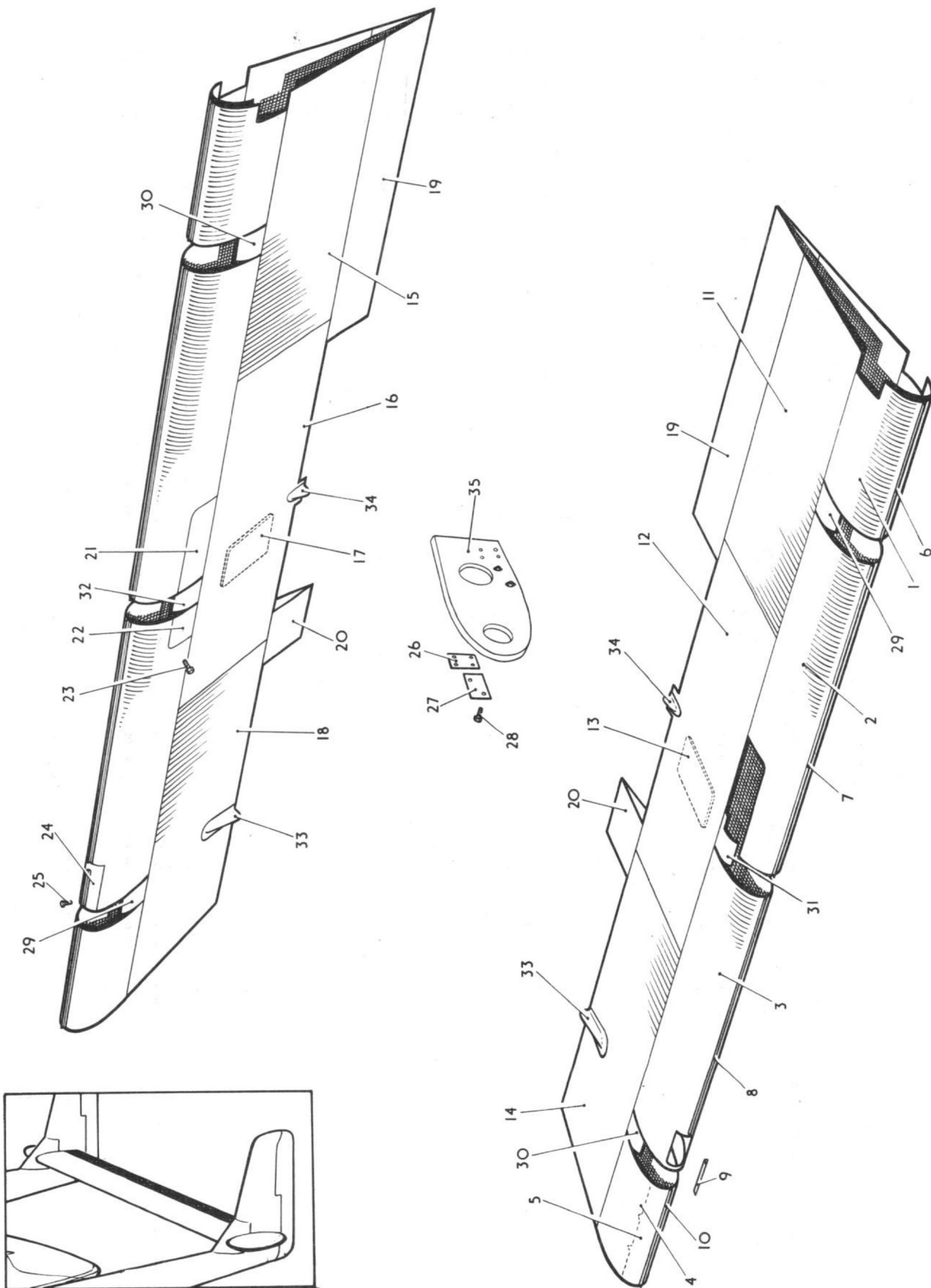
ELEVATOR SKINS AND ACCESS PANELS
