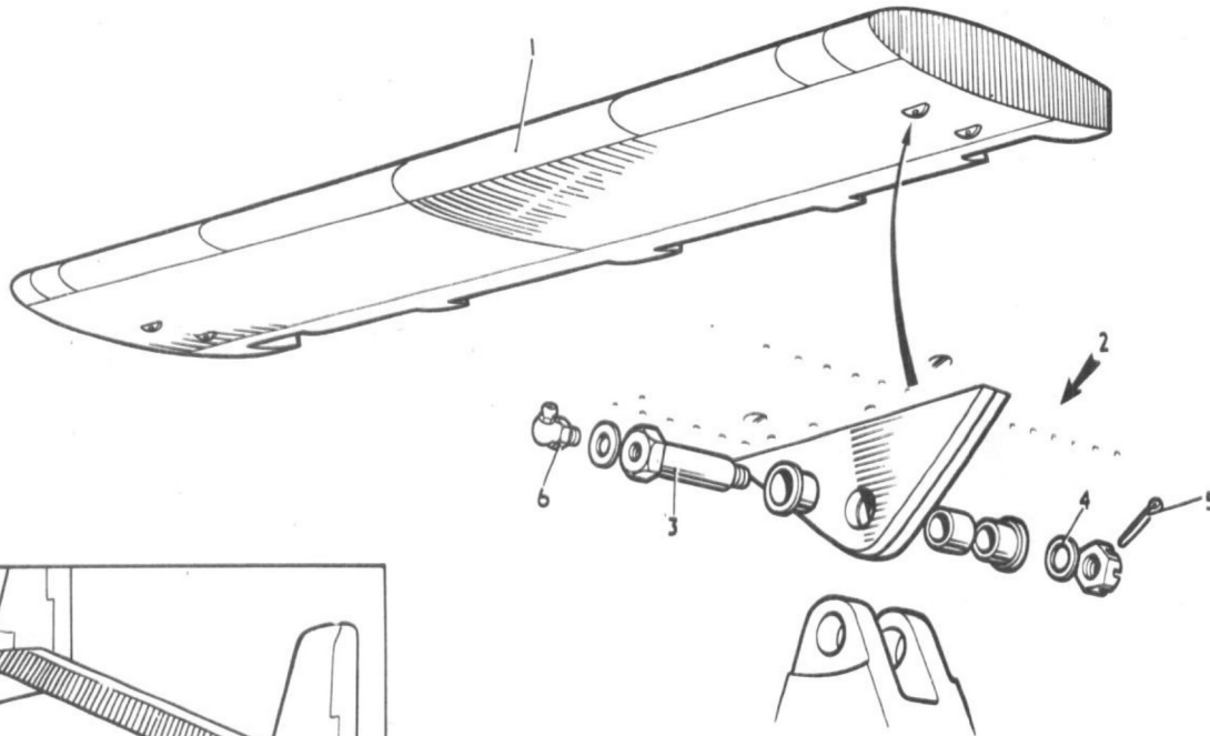
INSTALLATION OF TAILPLANE FIGURE I
