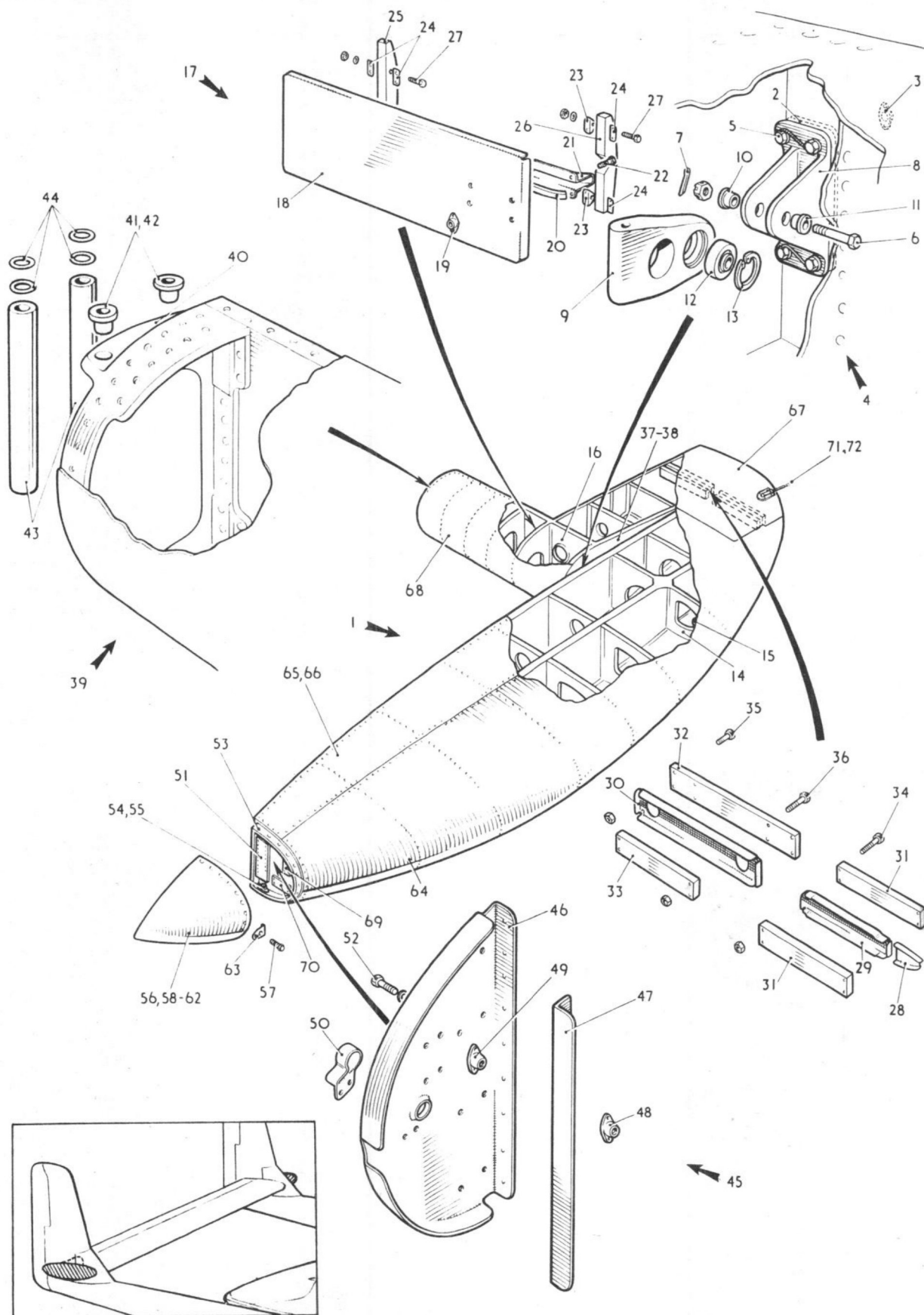
HORN BALANCE ASSEMBLY
