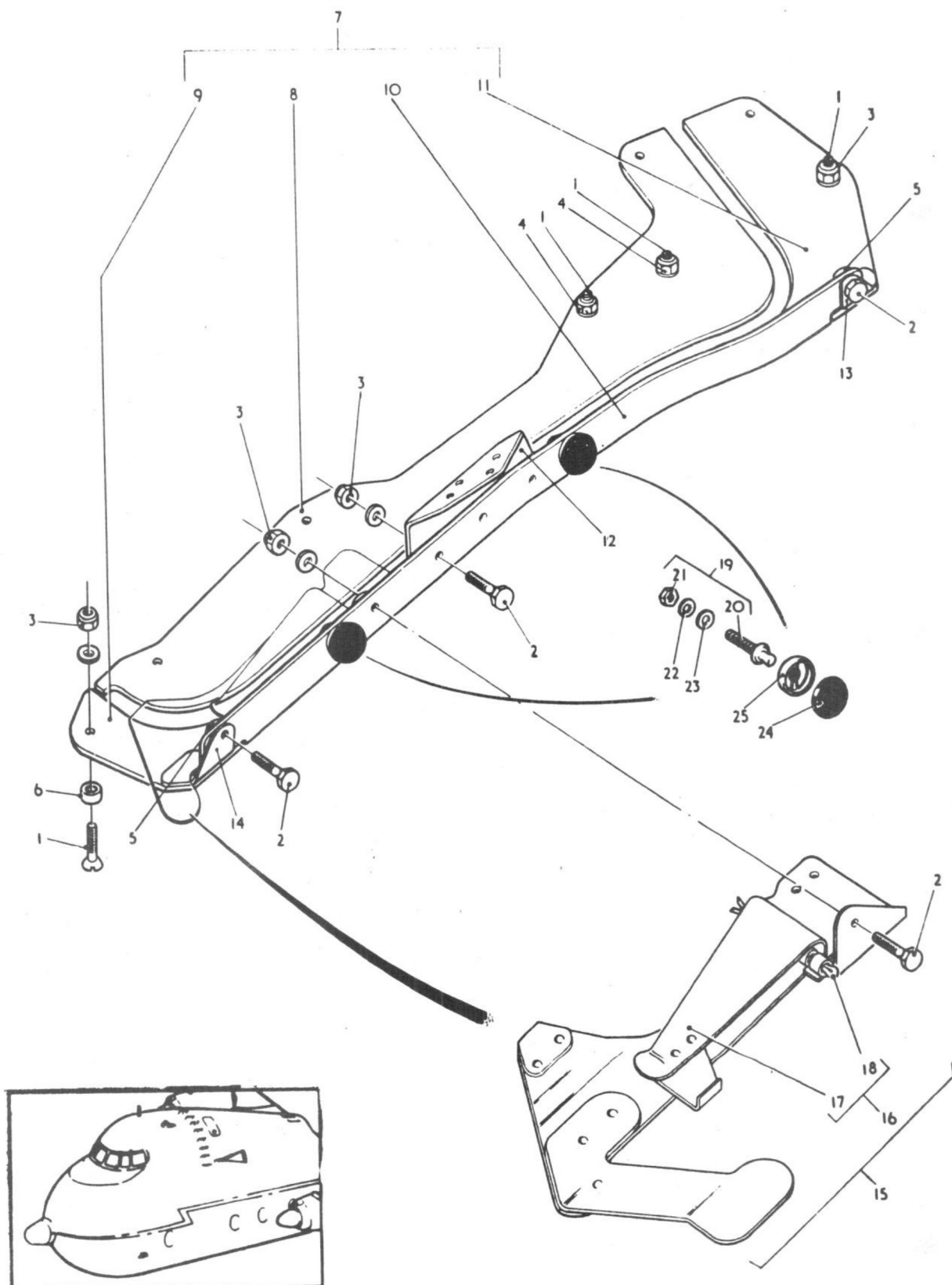
UPPER GUIDE TRACK ASSEMBLY
