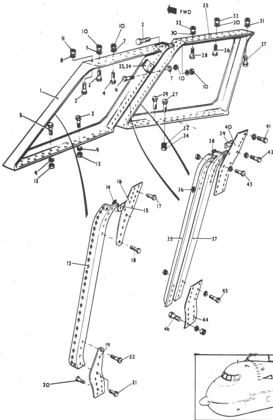
FRAME INSTALLATION WINDSCREEN
