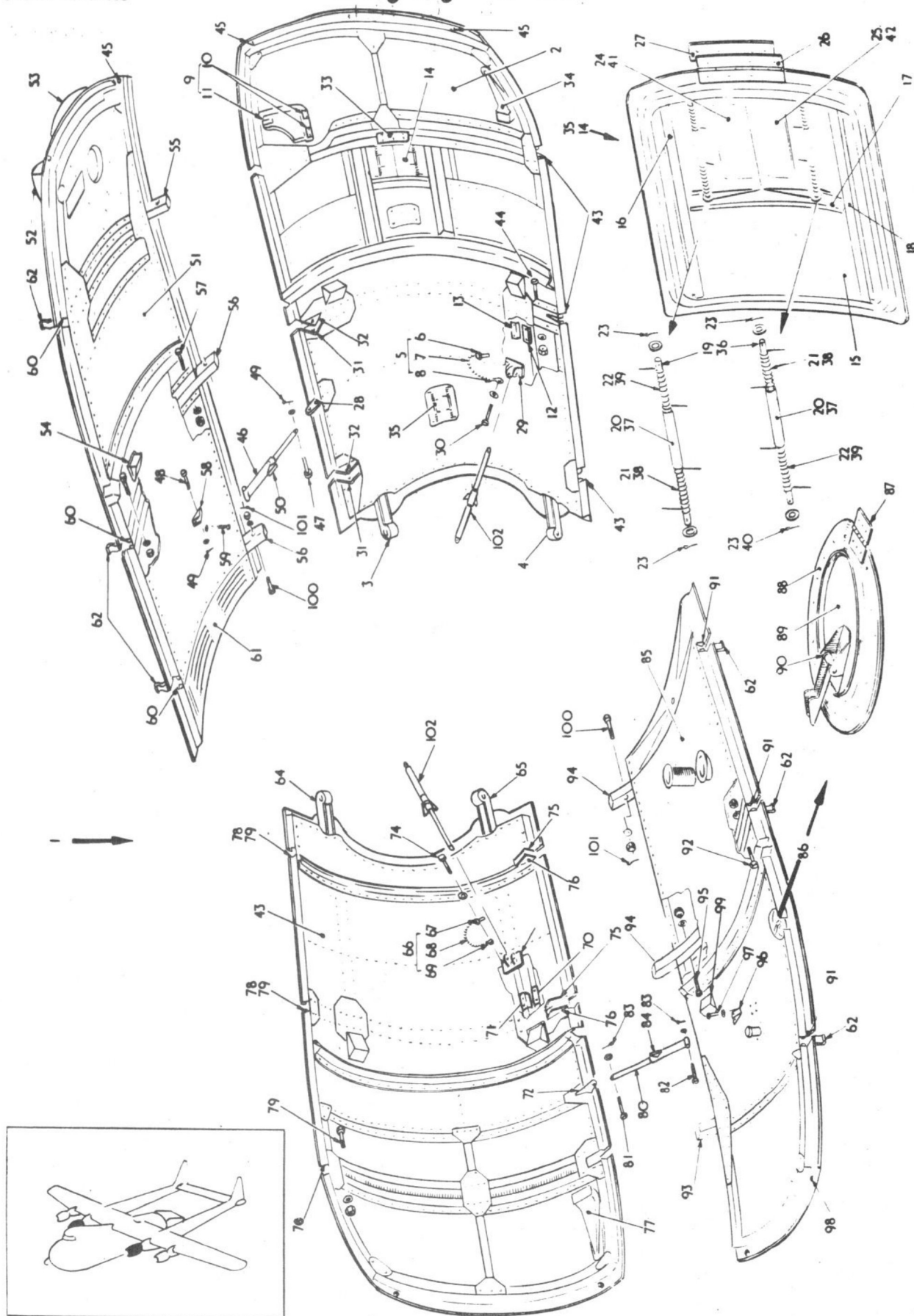
INBOARD COWLING FIGURE 1
