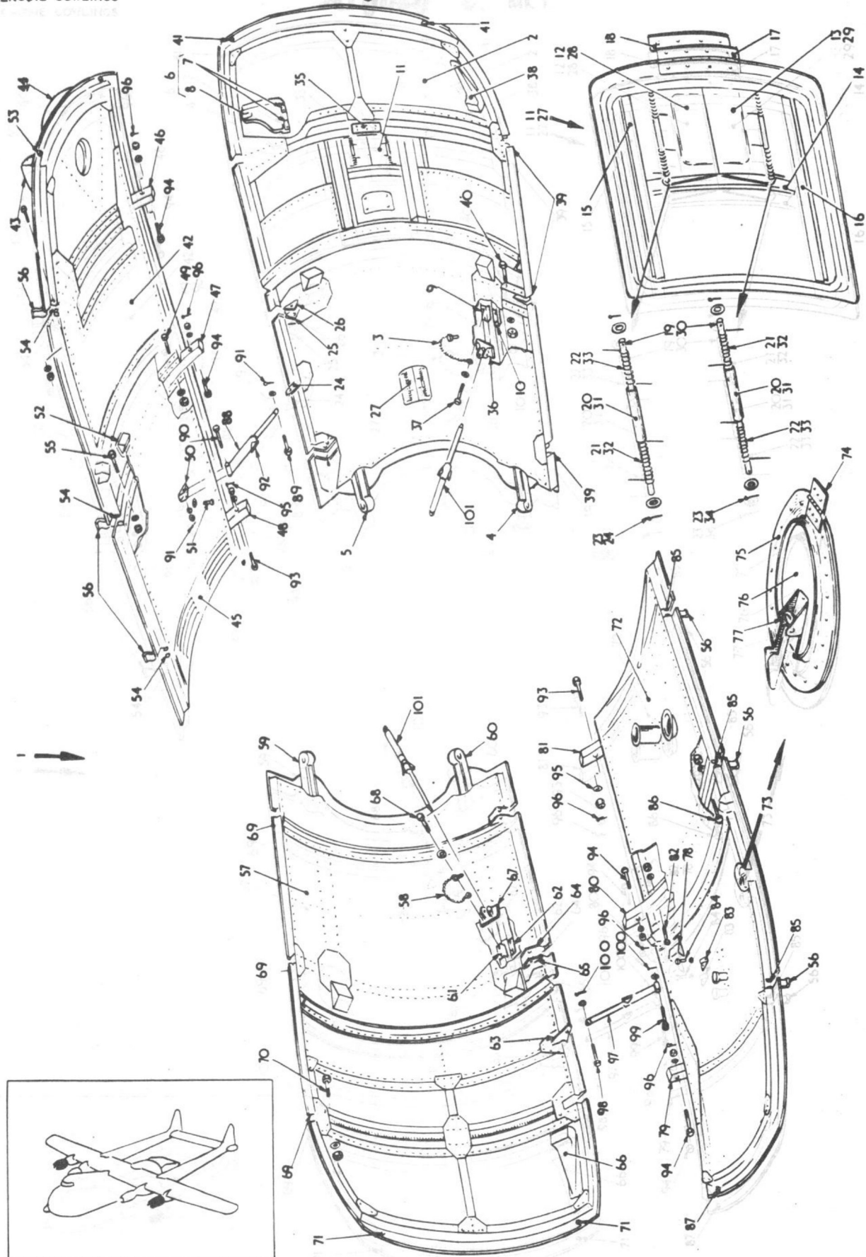
OUTBOARD COWLING FIGURE 2 RESTRICTED
