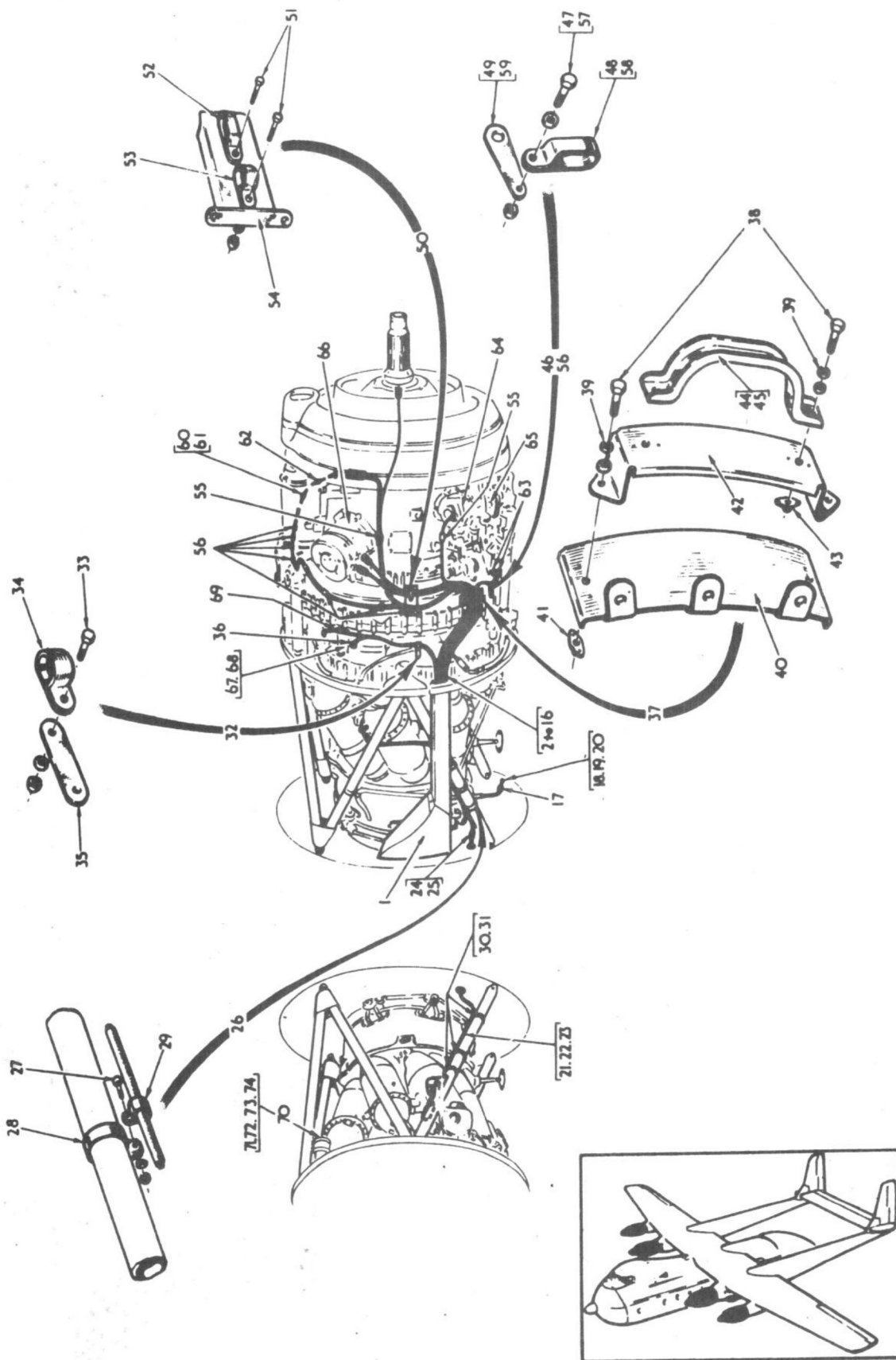
CABLES AND CLIPPINGS
