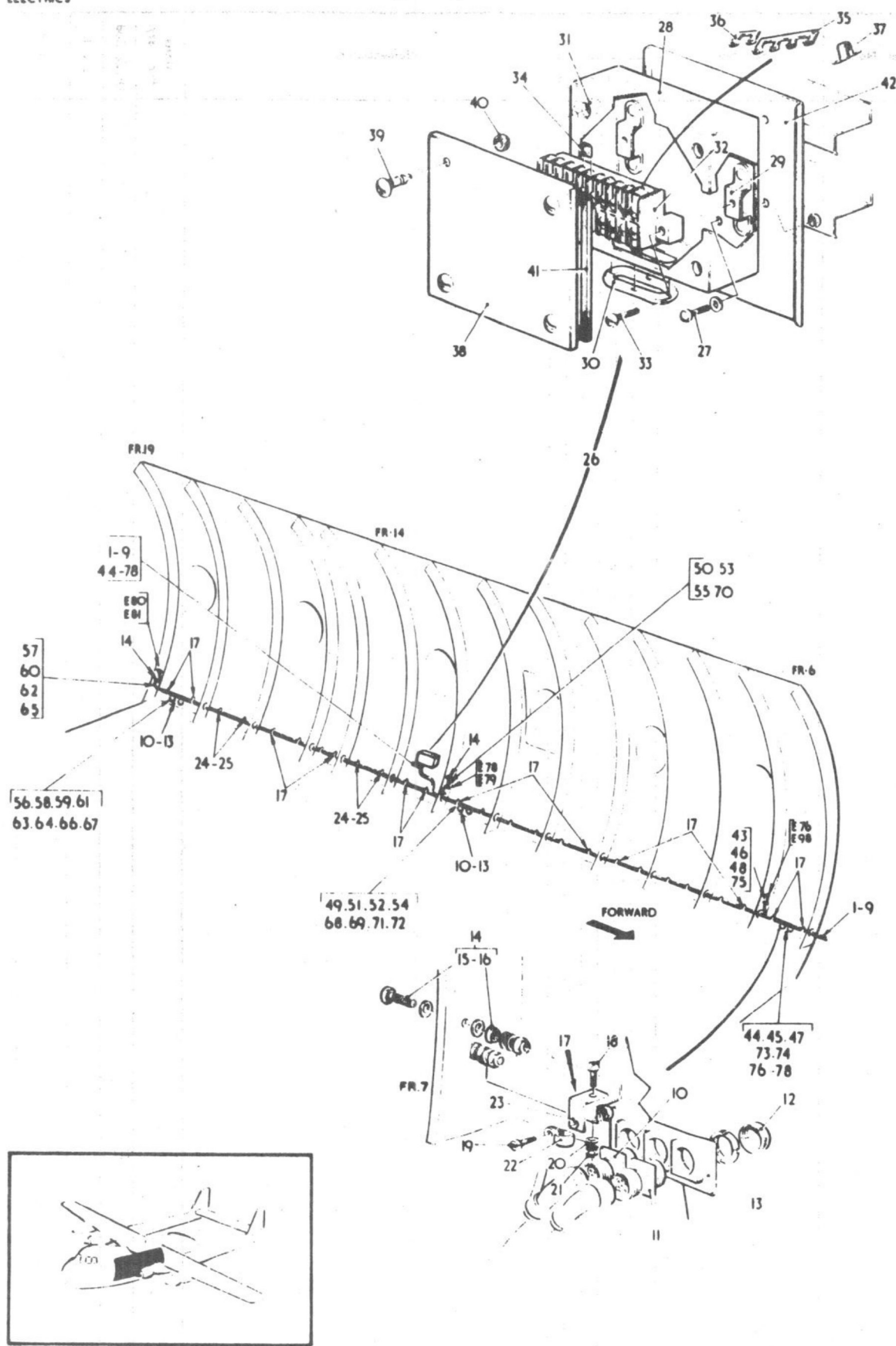
CABLE RUN TO BOMB SOCKETS (L-H)
