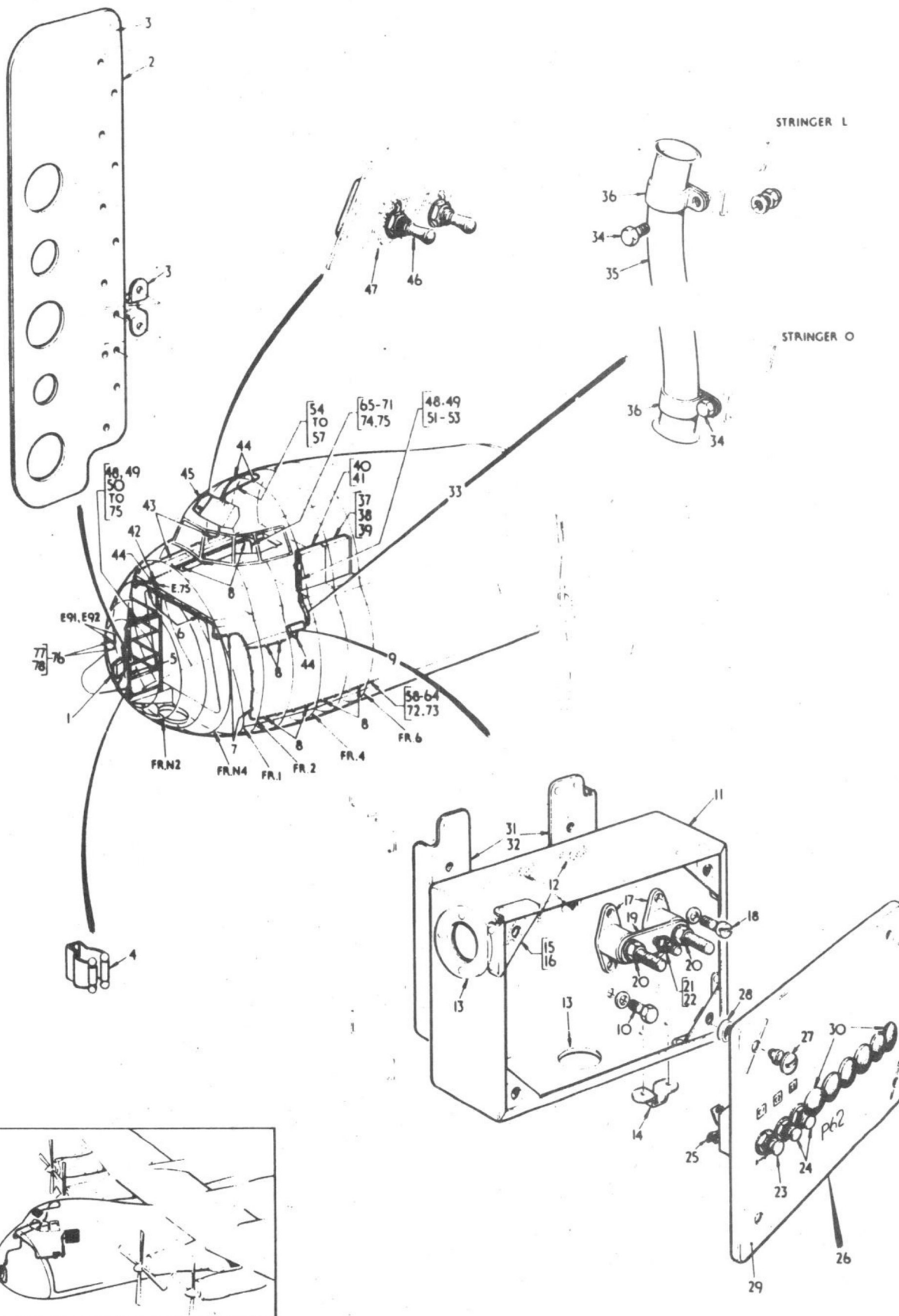
CABLE RUN FROM P63 TO FRAME 6.
