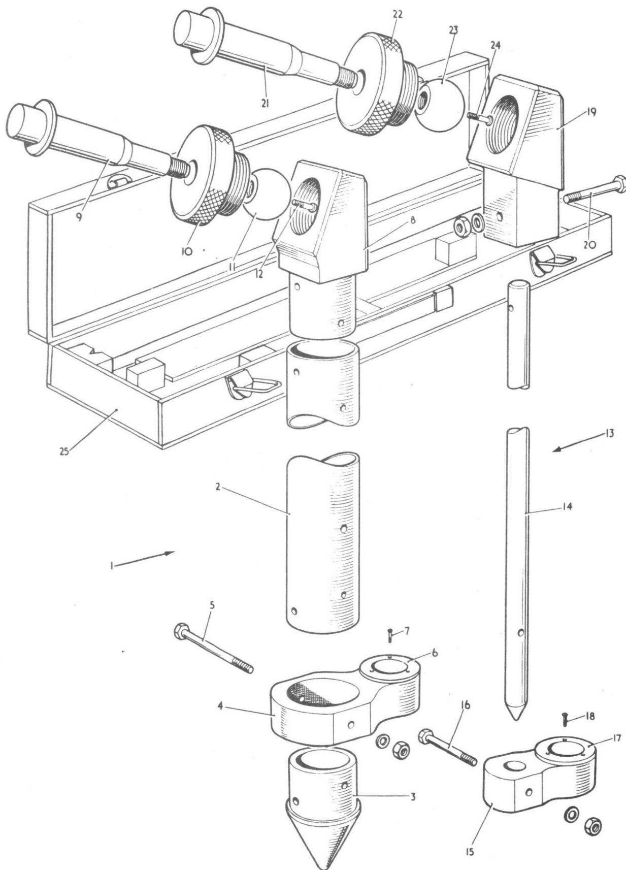
WAND ASSYS., FWD. &amp; AFT ALIGNMENT
