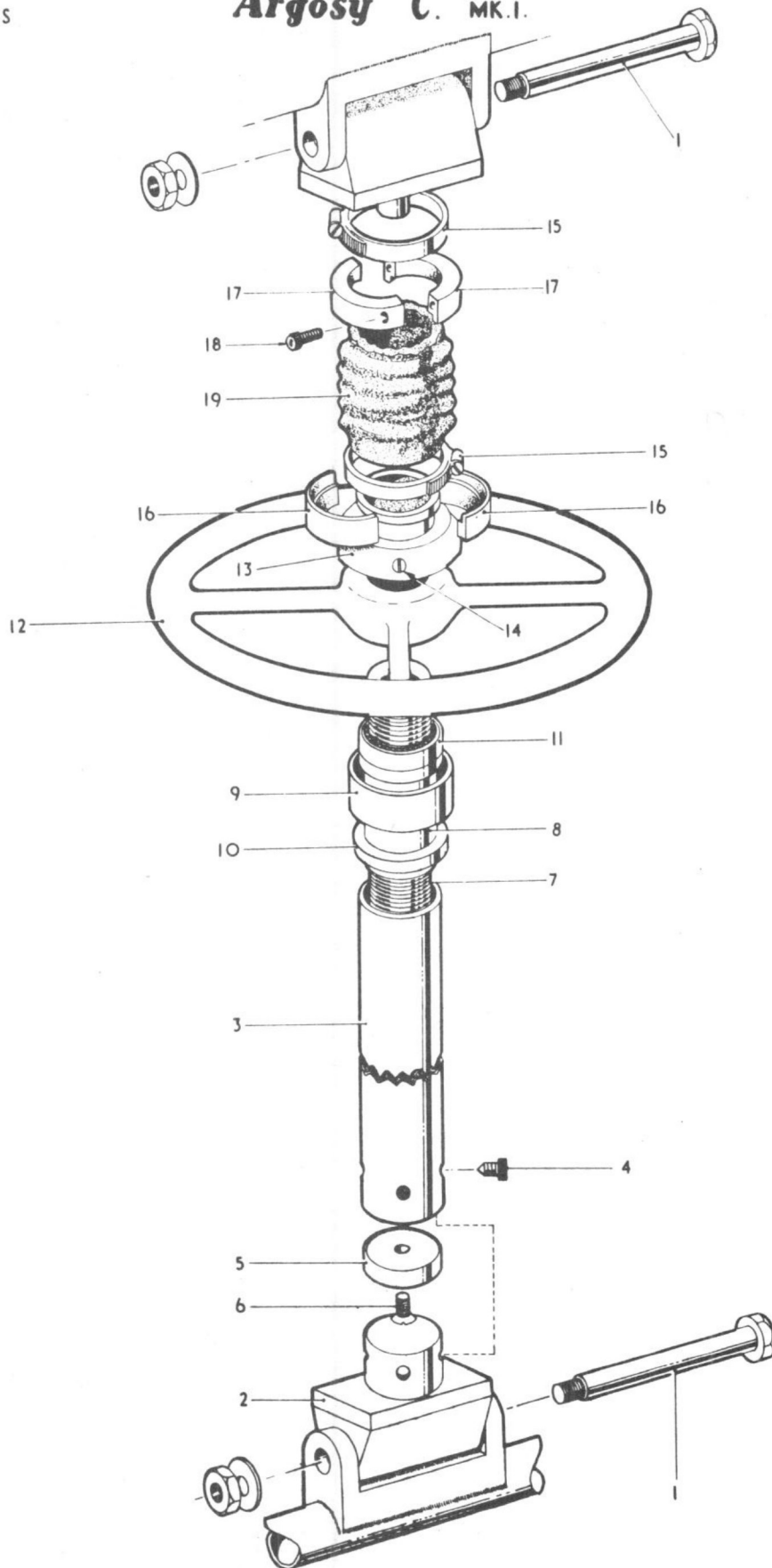
JACK AND BELLOWS ASSEMBLY
