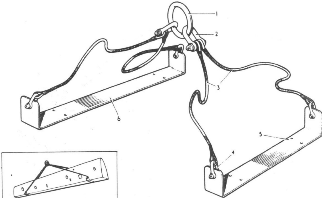
SLING ASSEMBLY, INTERMEDIATE MAINPLANE CARRIAGE
