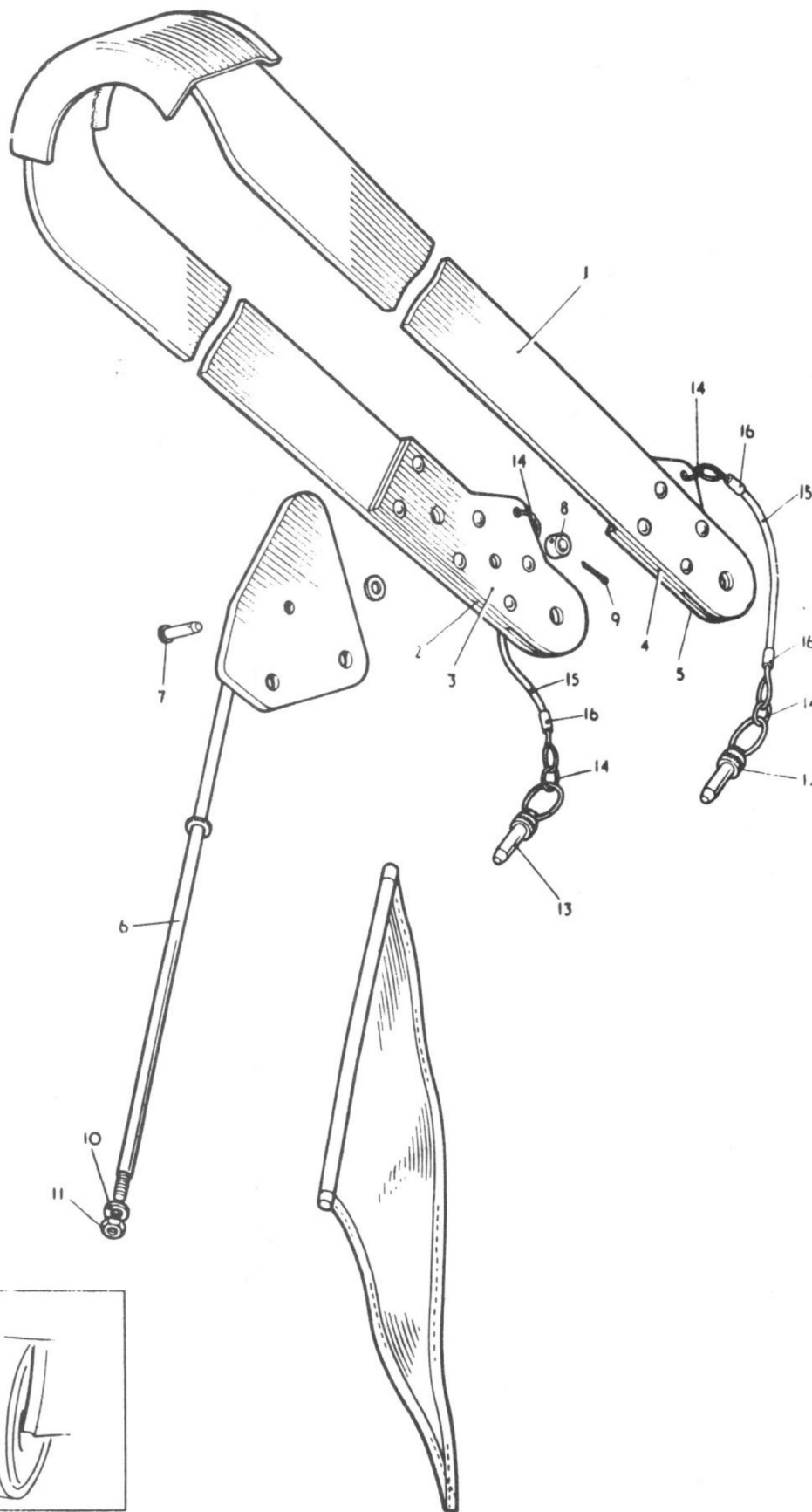
GAG ASSEMBLY, NOSEWHEEL UNDERCARRIAGE
