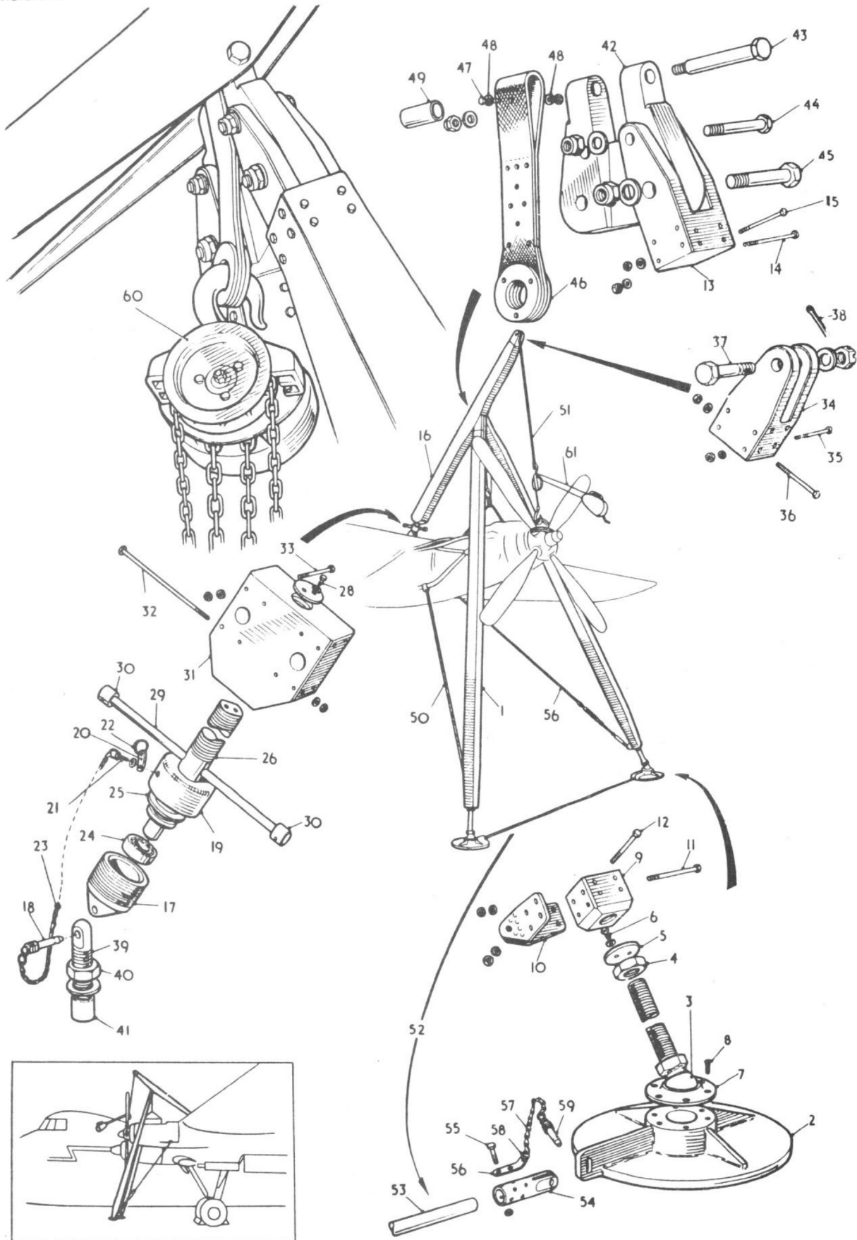
ENGINE CHANGE UNIT
