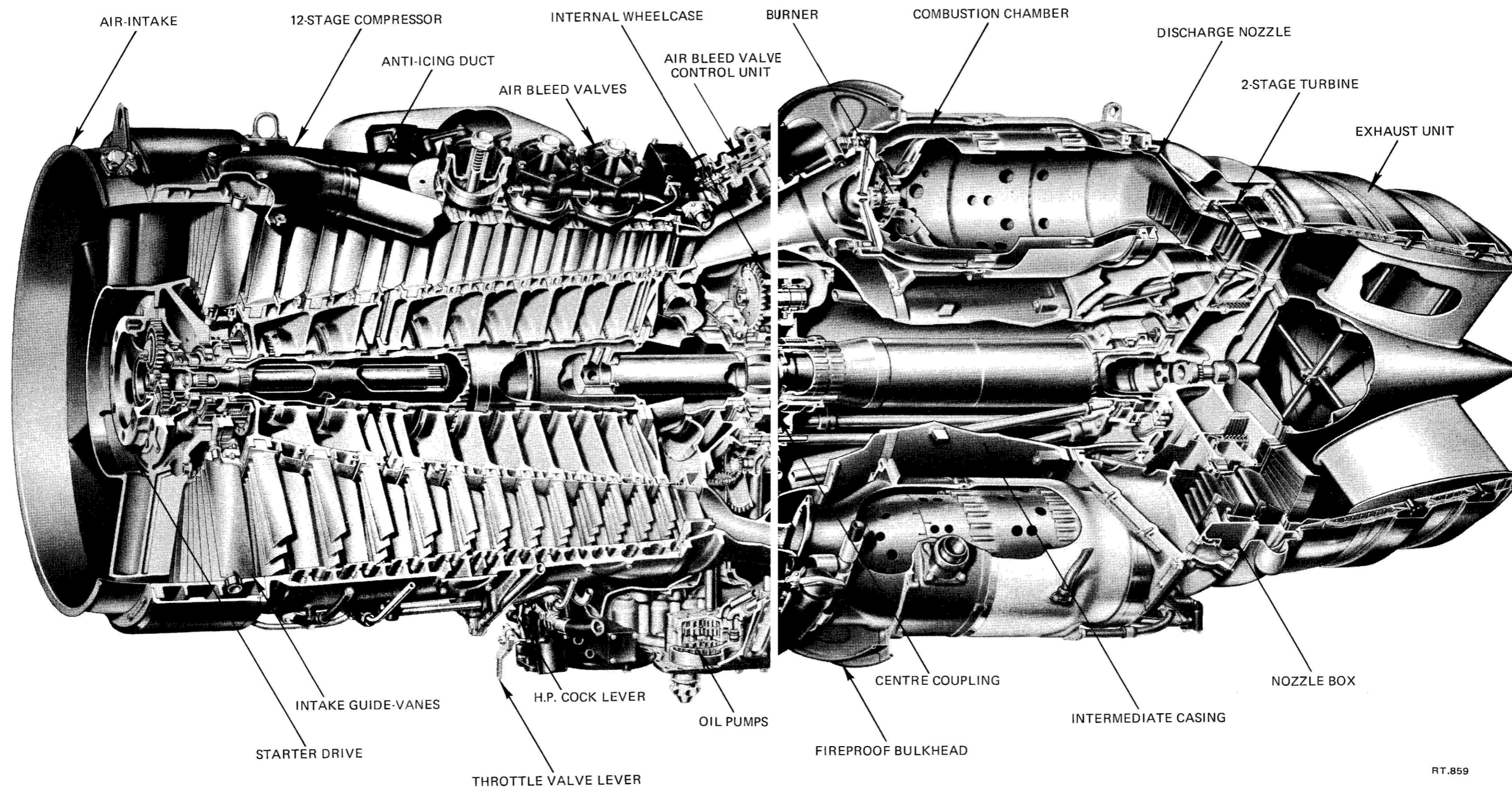
Frontispiece—Internal Construction
