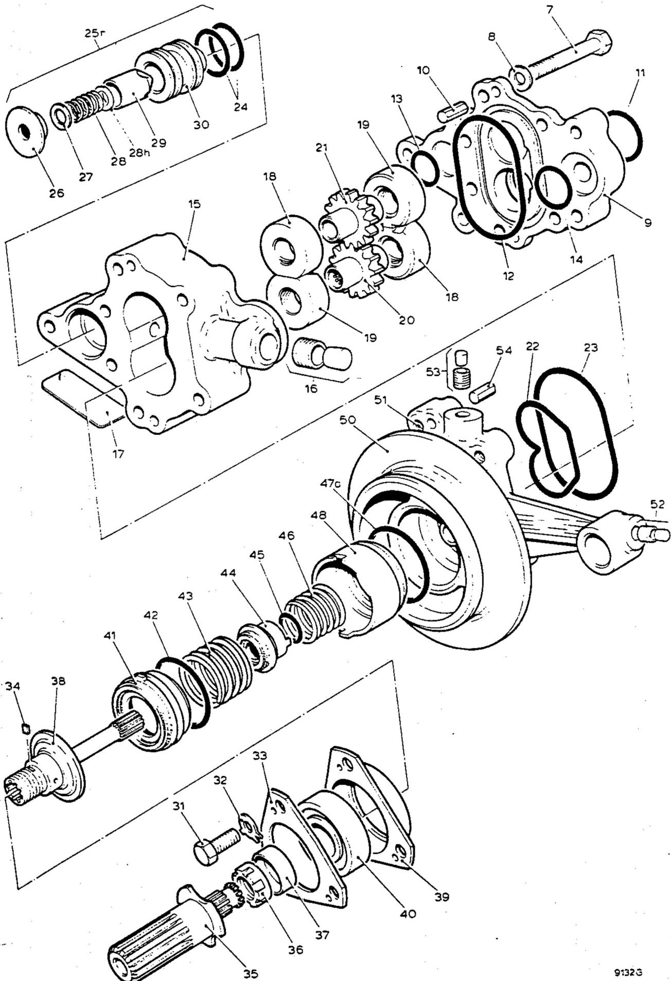
Fig 7 Fuel pump assembly (Effect of Mod 2724)
