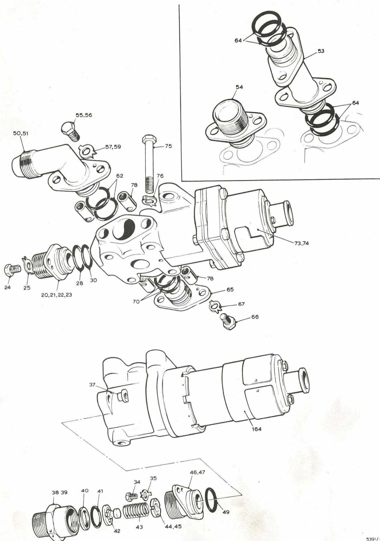
Fig.1 H.P. switch and solenoid valve
