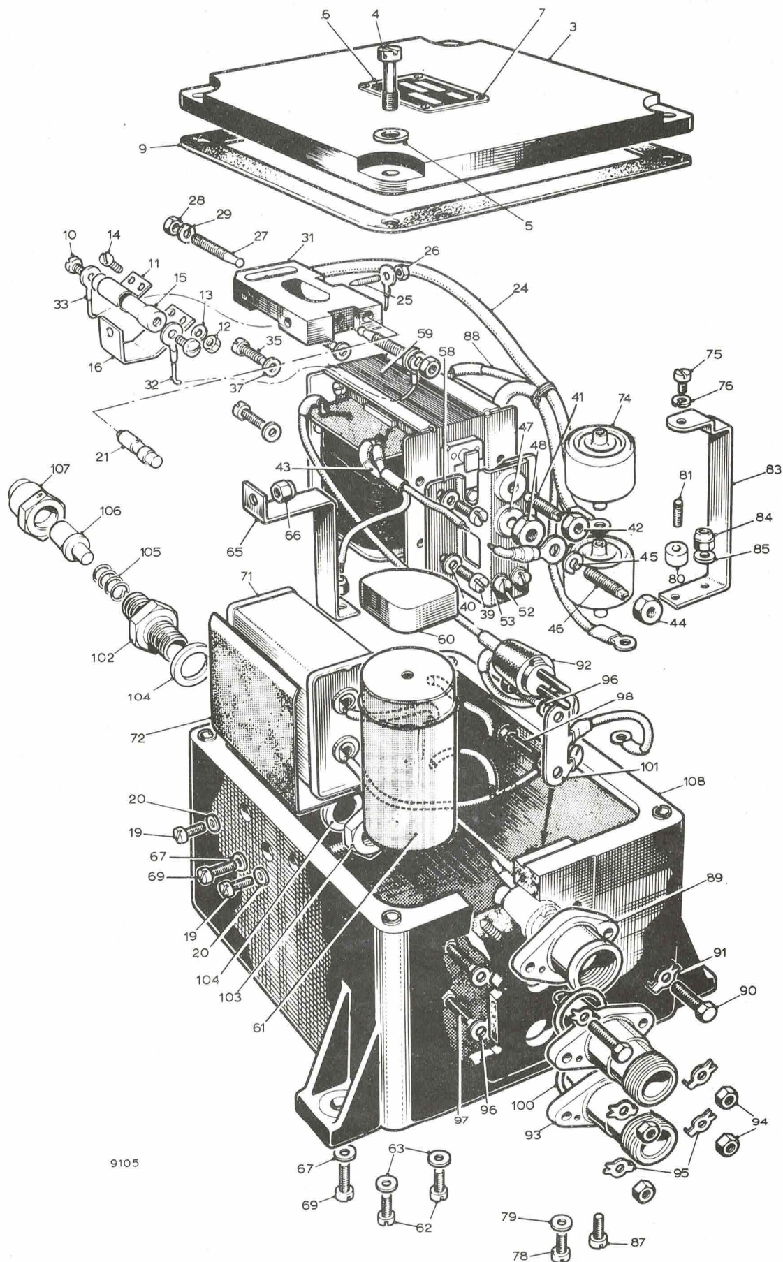
Fig.1 Ignition unit
