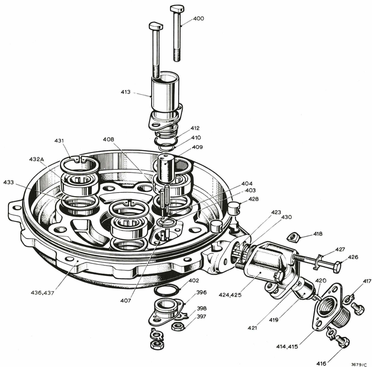
Fig.10 Rear bearing housing
