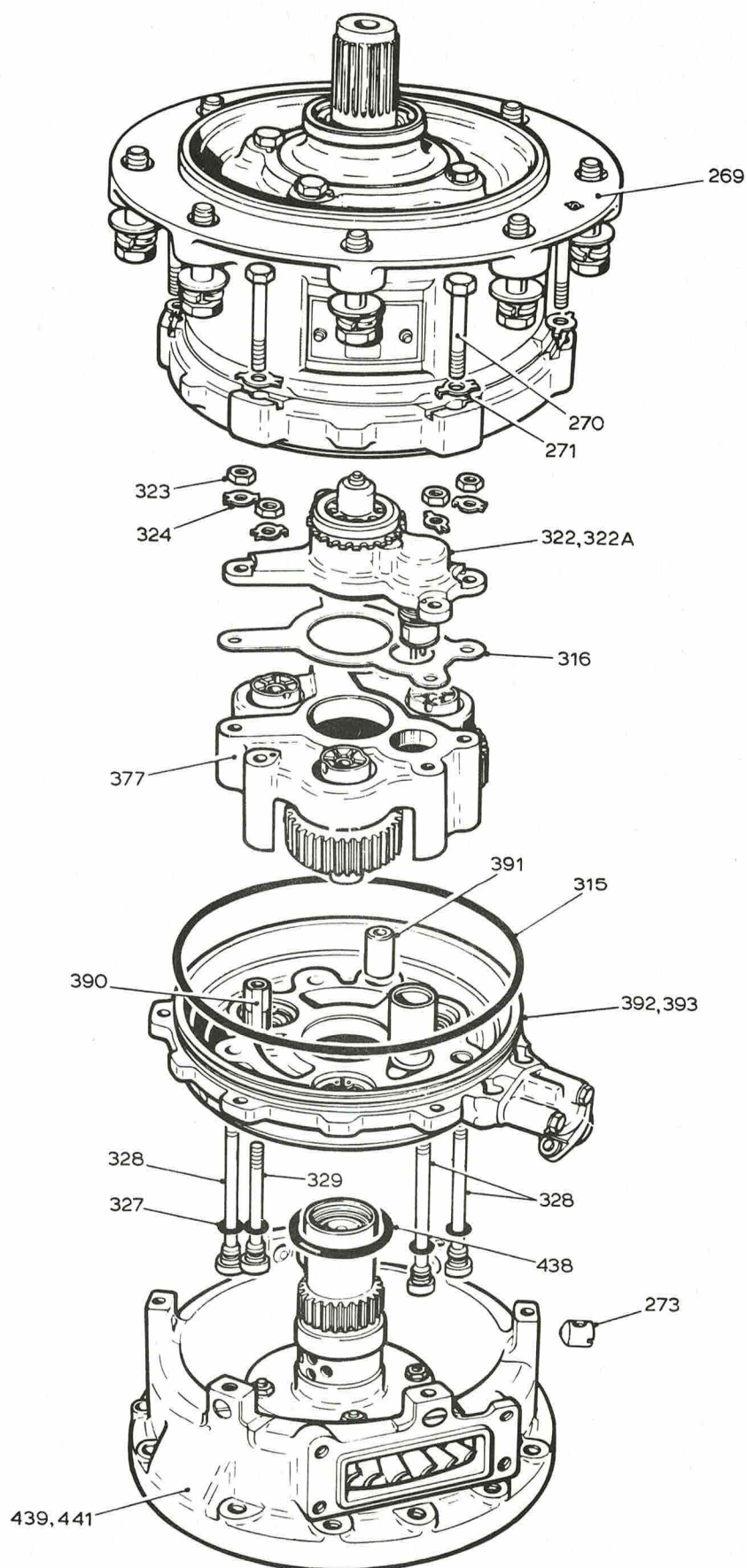
Fig.6 Gearbox assembly
