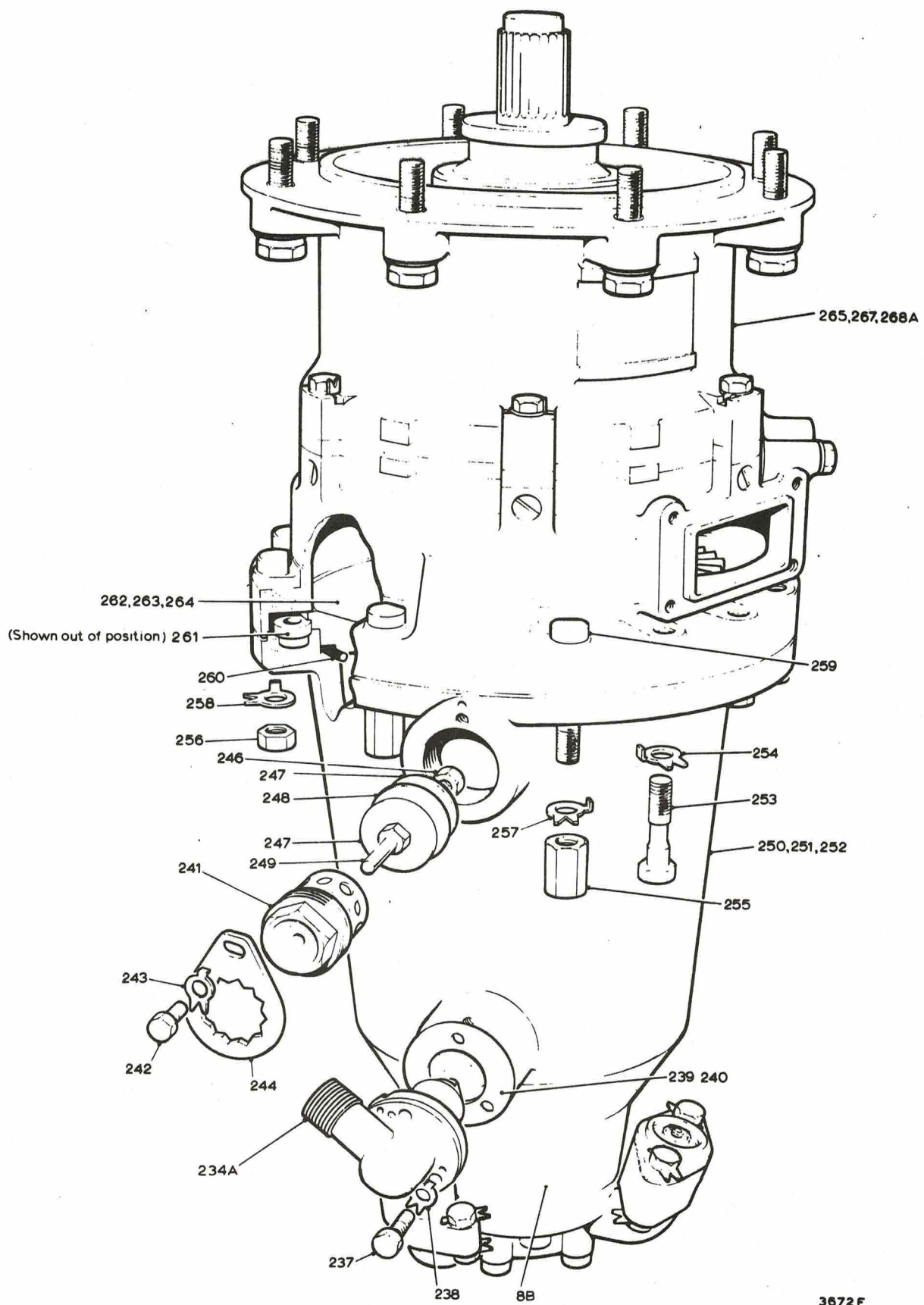
Fig.1 Starter Motor
