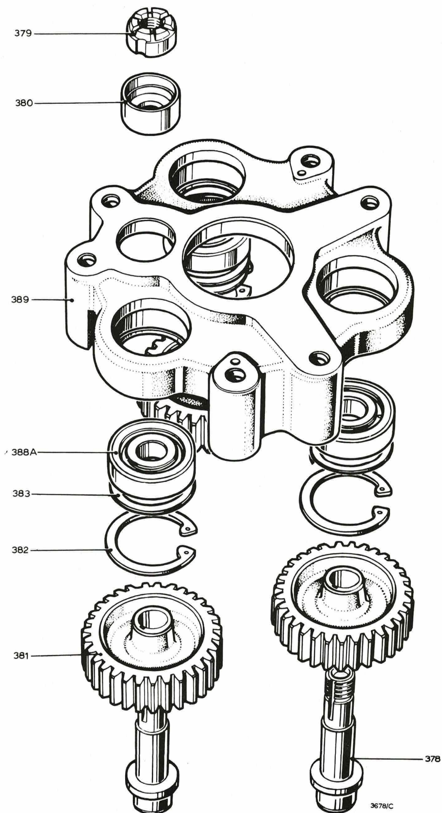
Fig.9 Layshaft bearing housing
