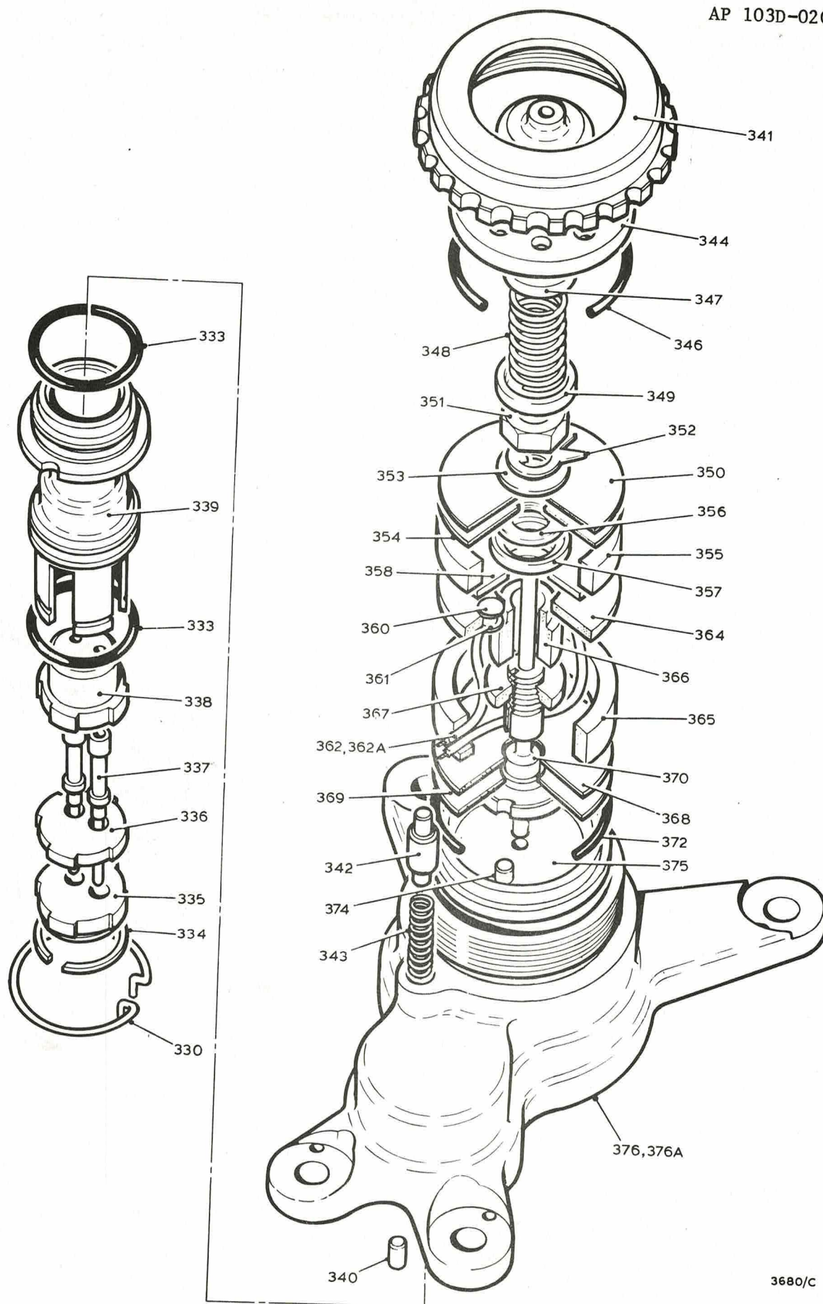
Fig.8 Speed control switch
