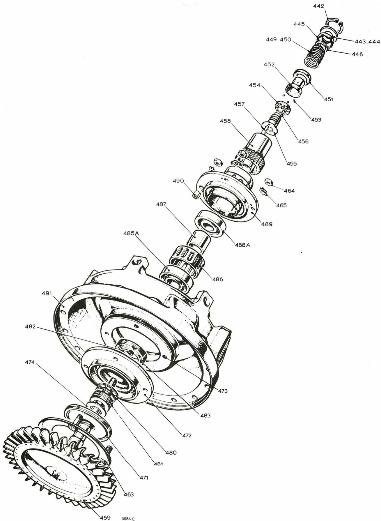
Fig.11 Turbine unit
